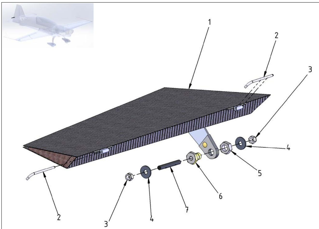
Figure 27-37 Elevator & Tab – Trim Tab
