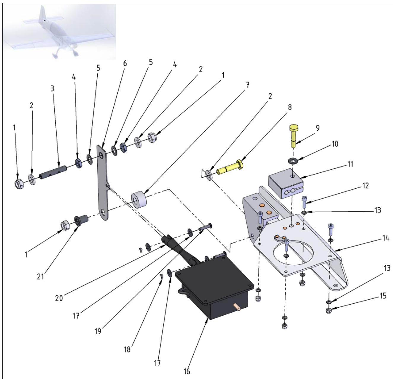
Figure 27-38 Elevator & Tab – Trim Control
