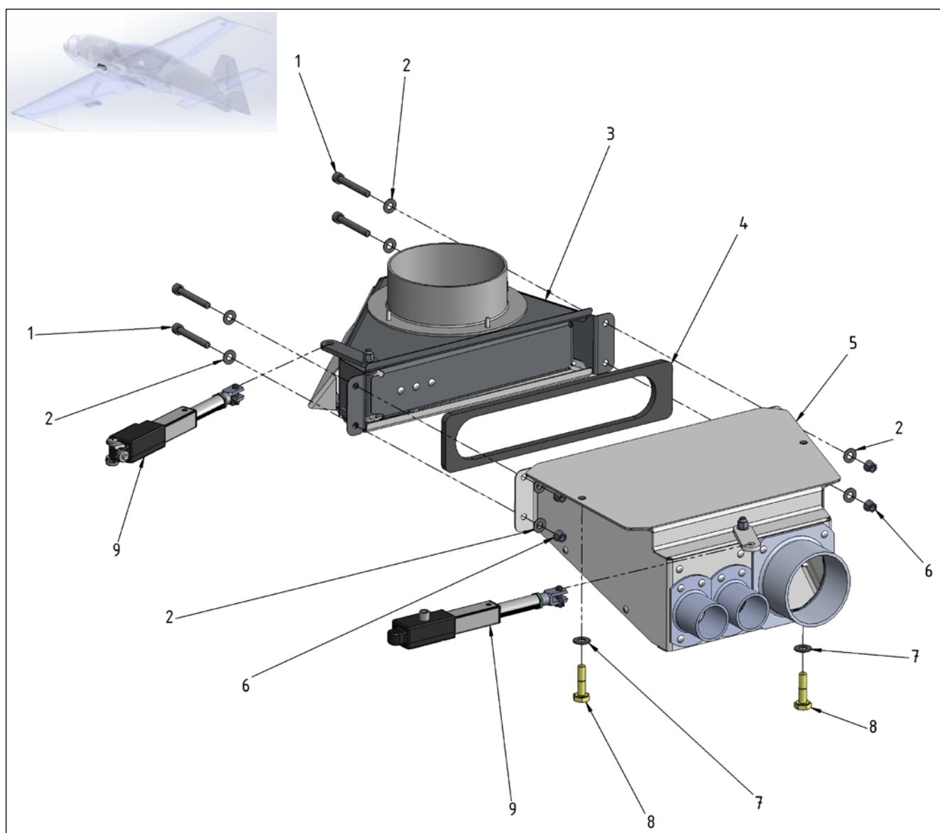
Figure 21-2 Boxes
