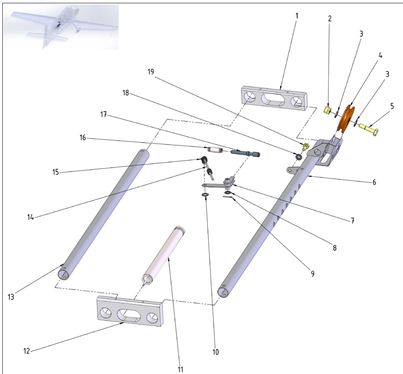
Figure 27-32 Rear Pedal LH - Base
