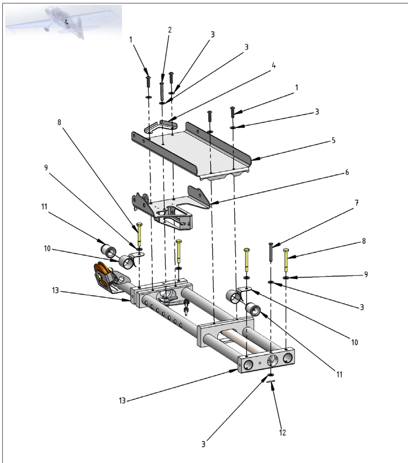
Figure 27-34 Rear Pedal RH - Footrest
