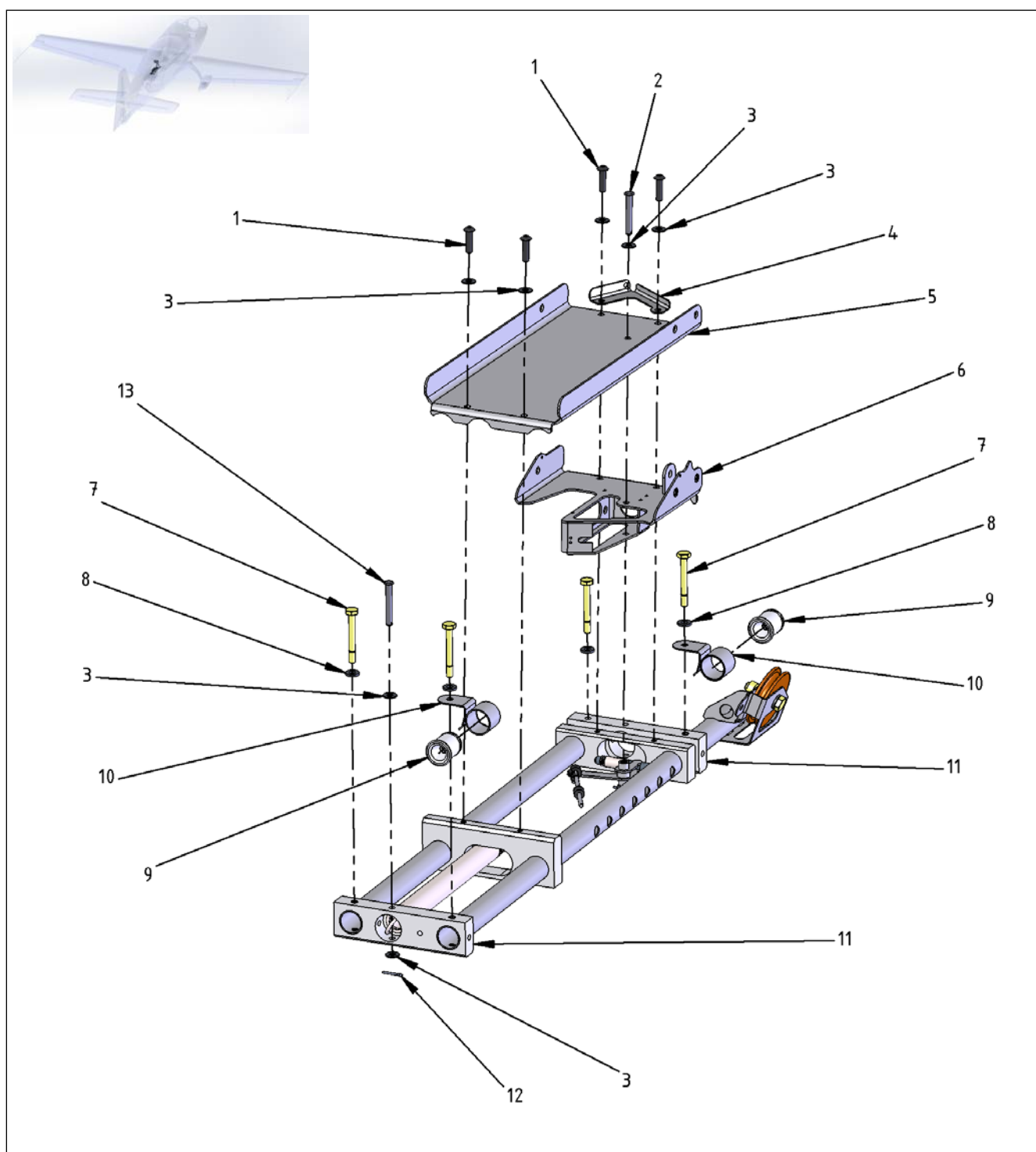
Figure 27-31 Rear Pedal LH - Footrest
