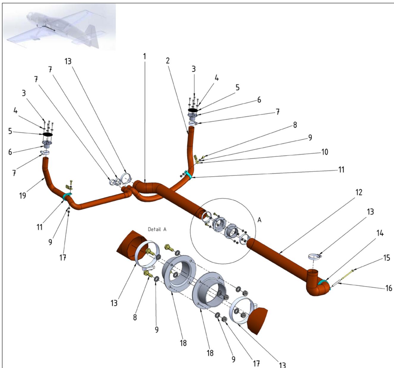
Figure 21-3 Hoses
