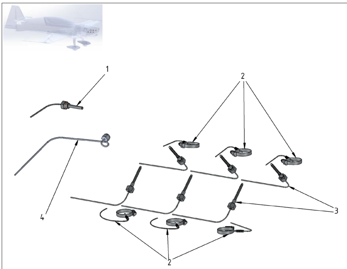
Figure 77-2 Engine Sensors
