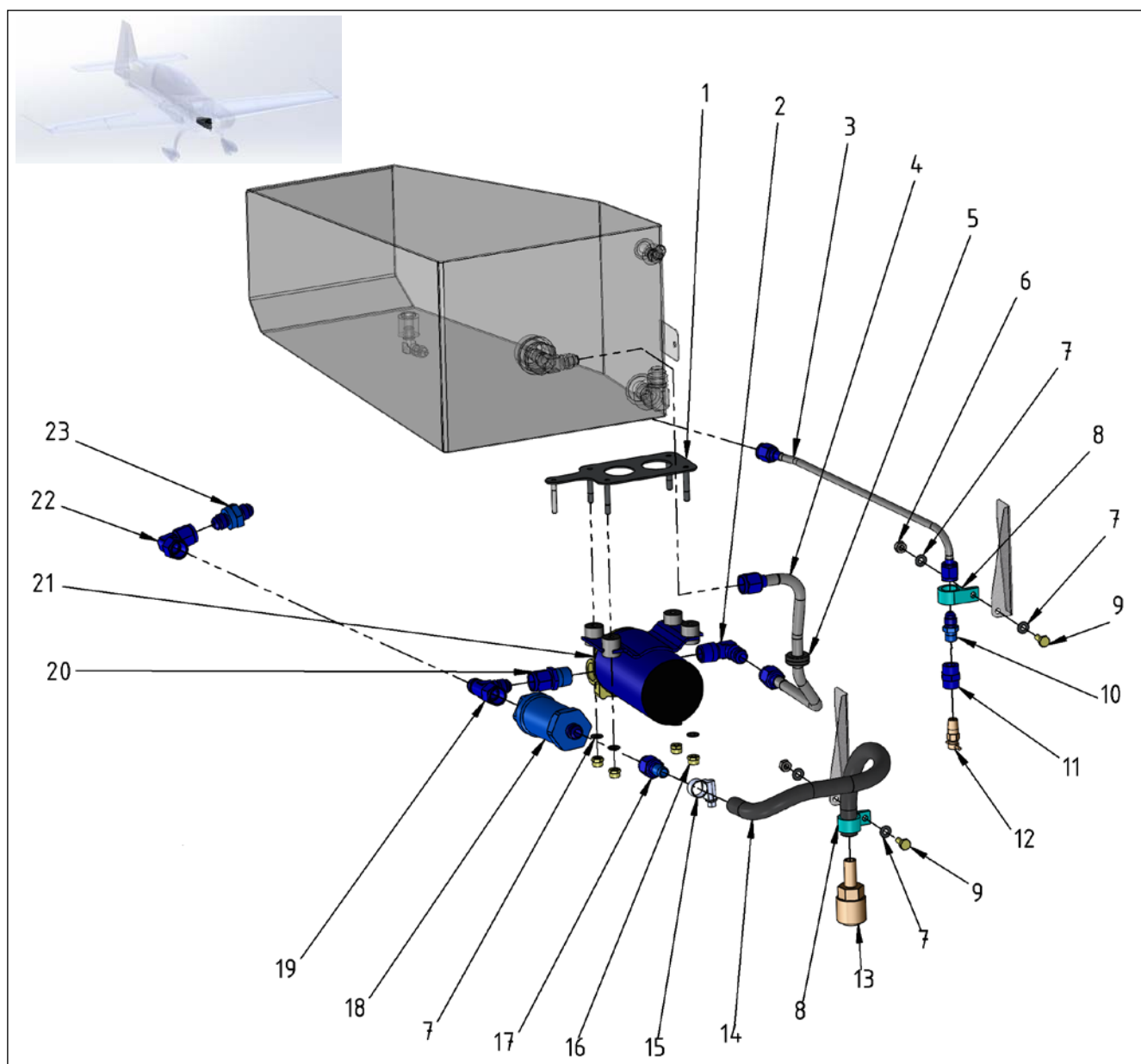
Figure 87-2 Smoke - Distribution
