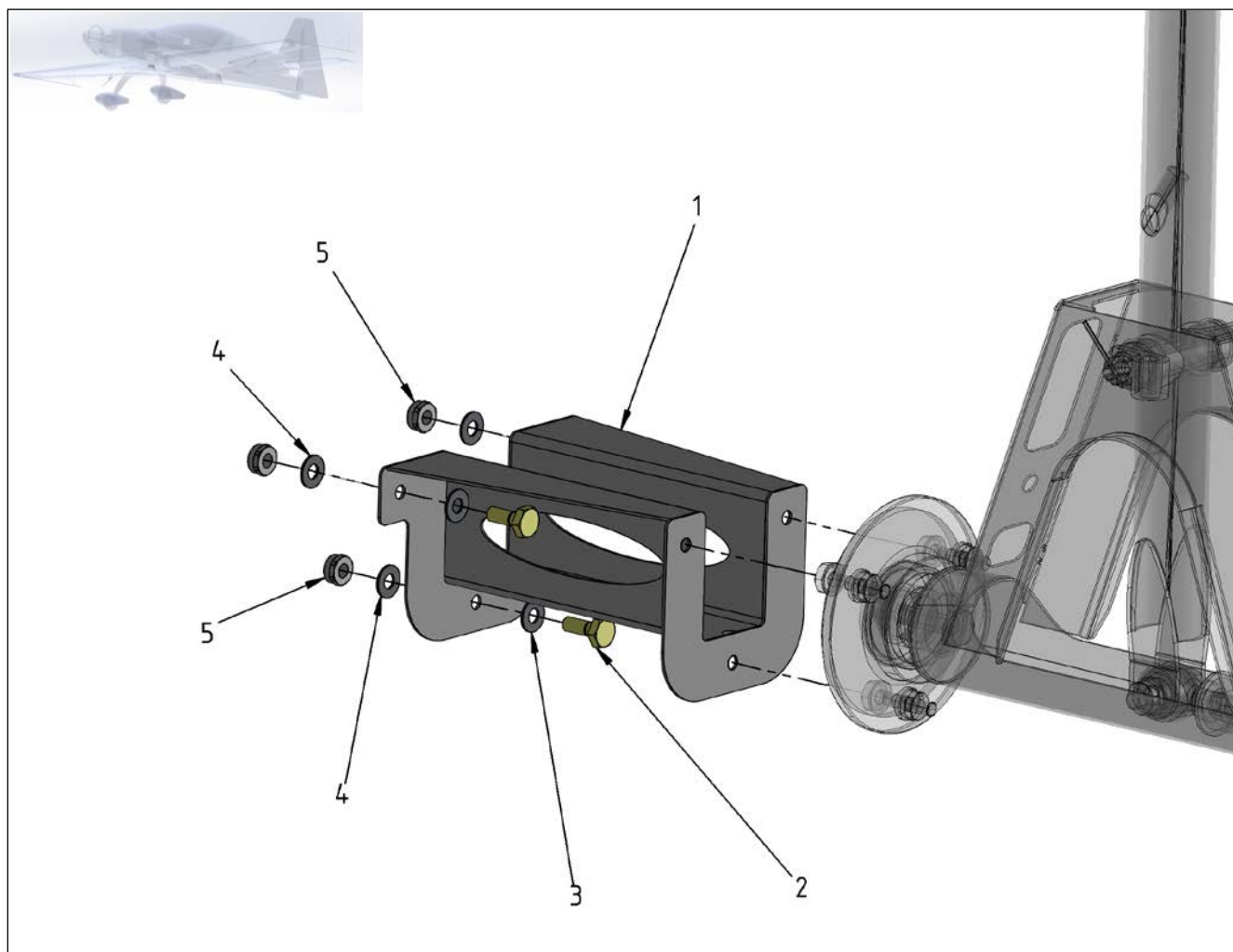
Figure 27-12 Torque Tube Bracing
