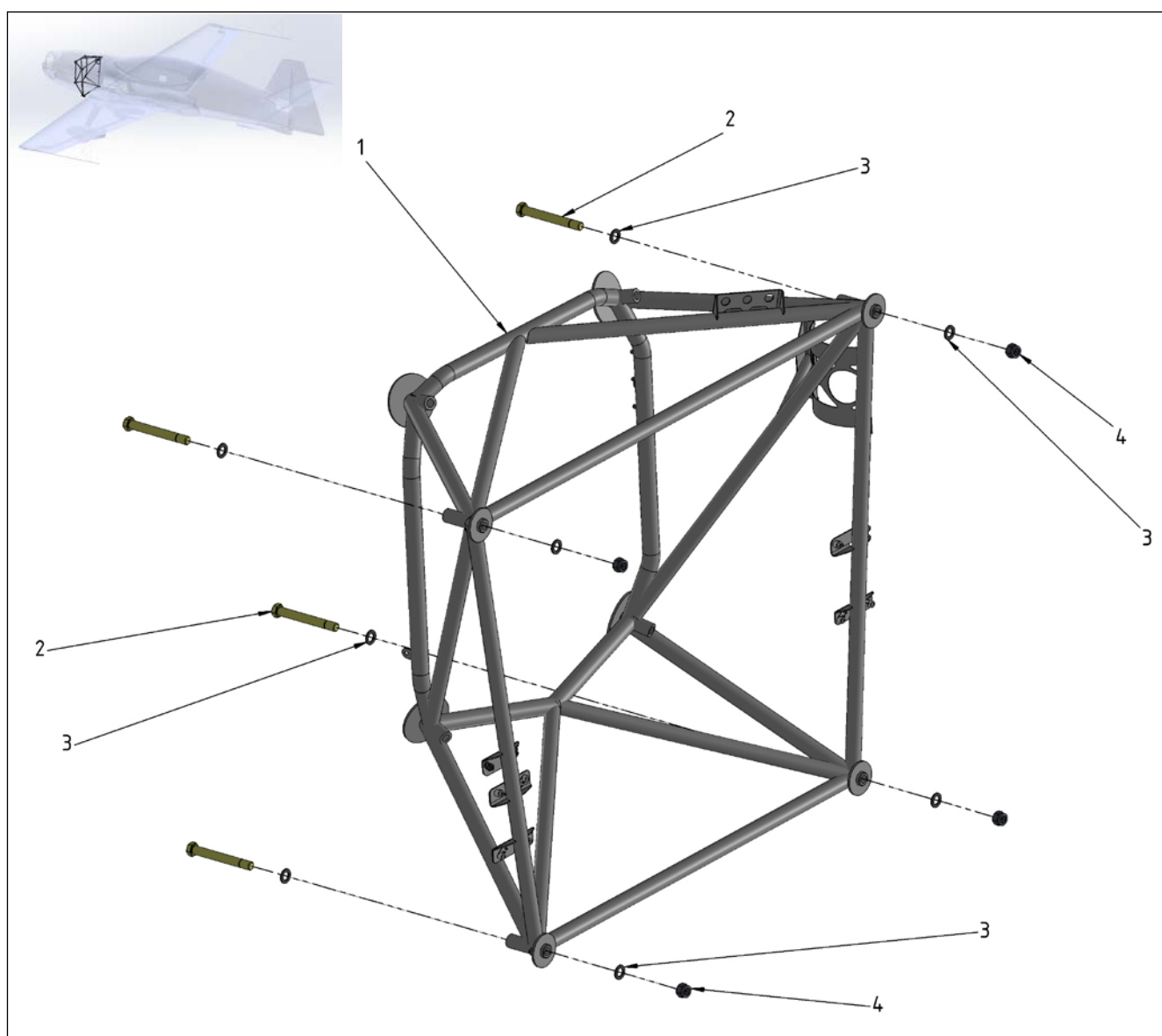
Figure 71-1 Engine Mount
