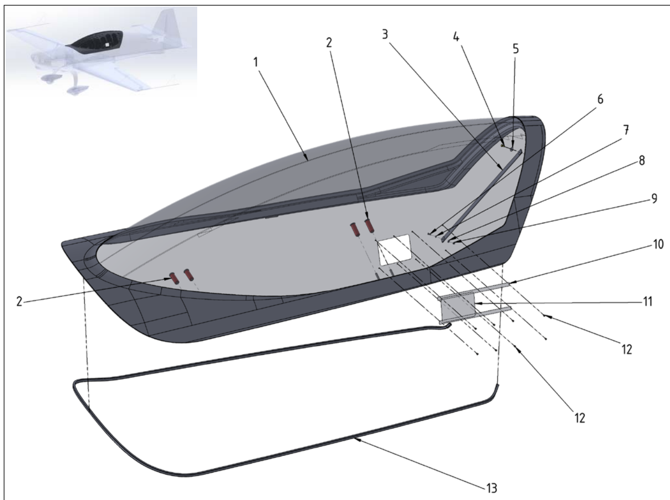
Figure 53-2 Canopy
