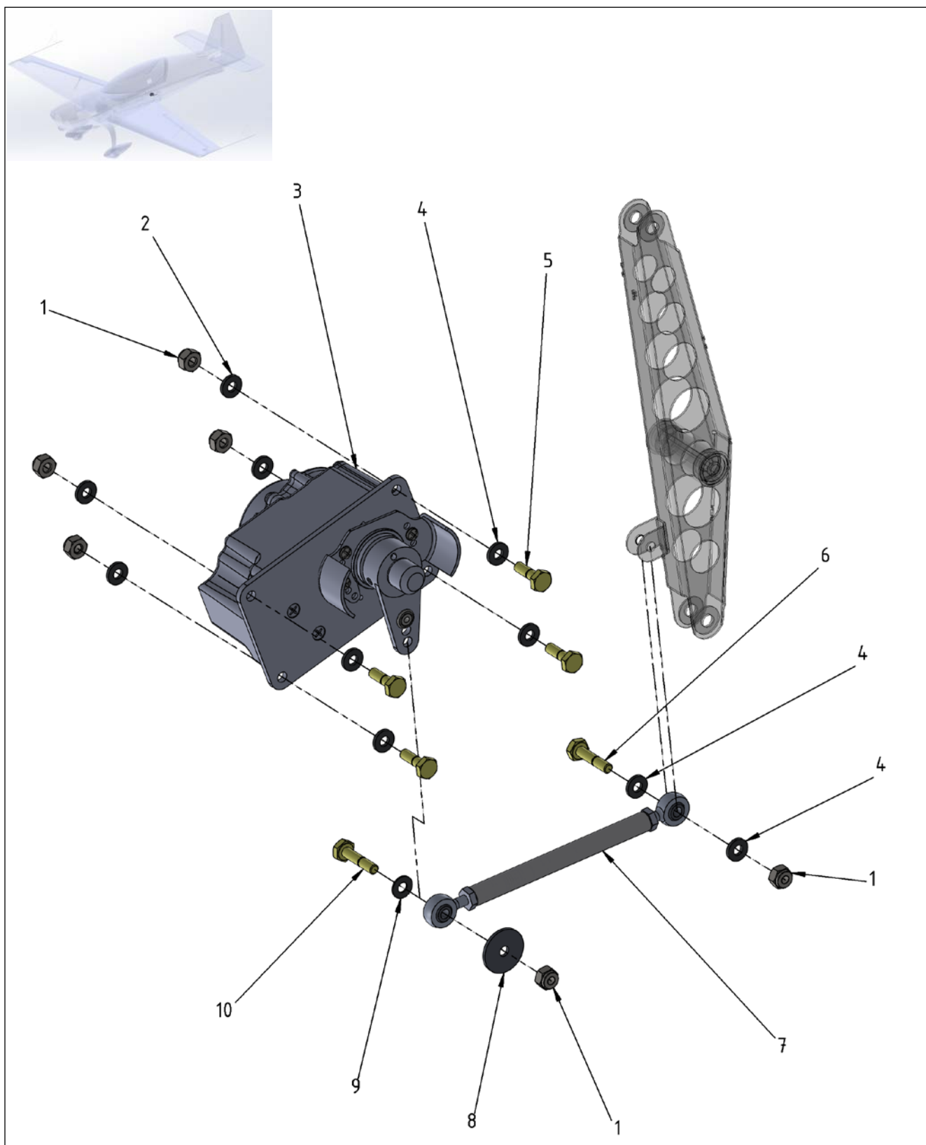
Figure 22-2 Pitch Servo
