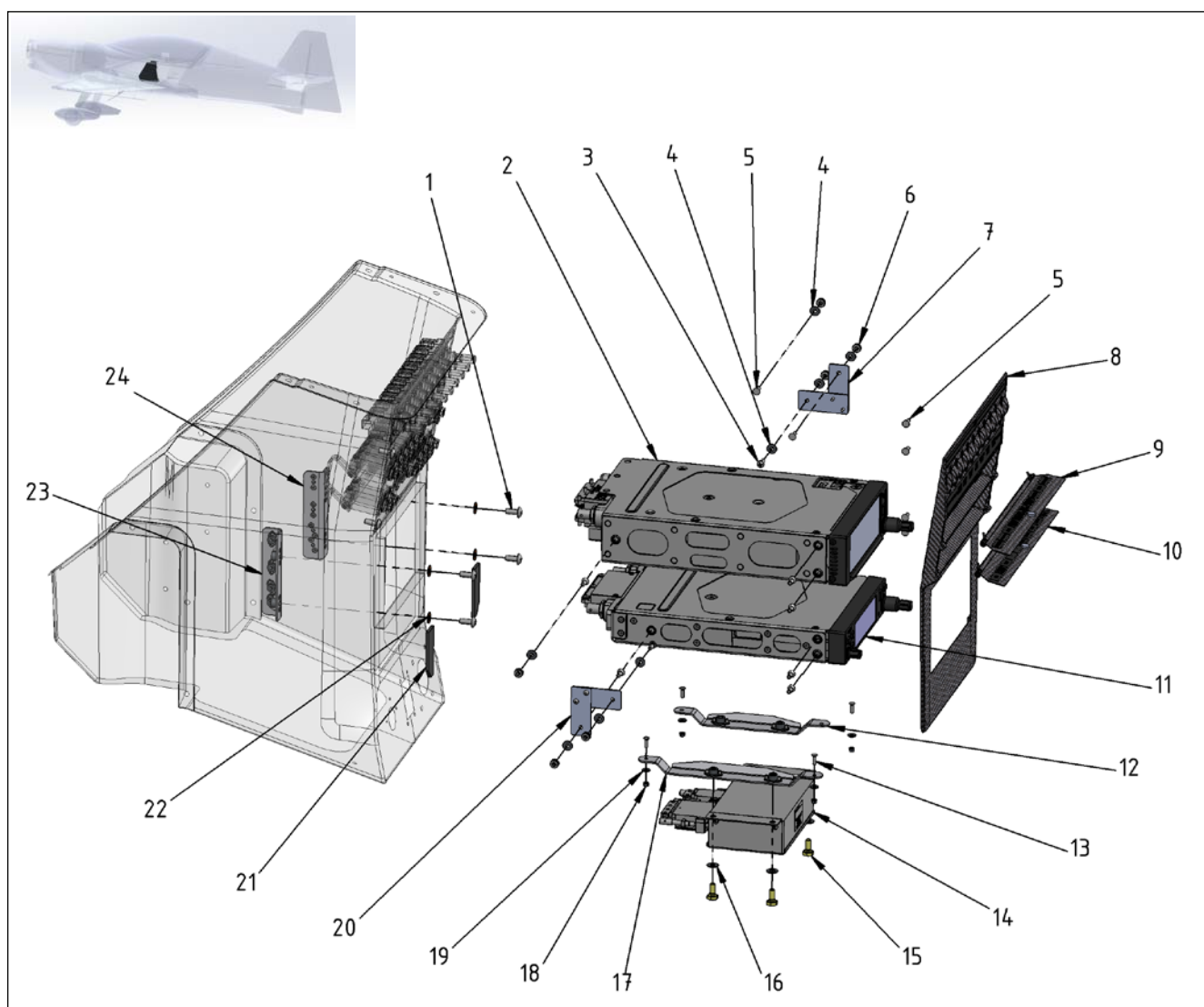
Figure 31-7 Center Console Options – GNX 375 + GTR 205A
