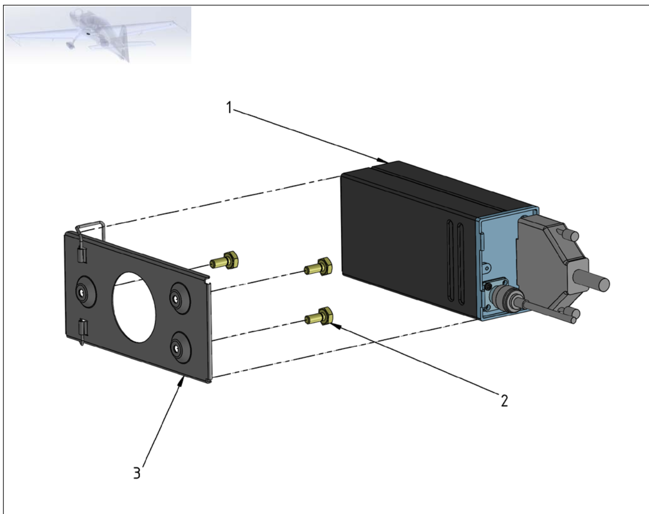
Figure 34-4 Dependent Position Determining - Transponder
