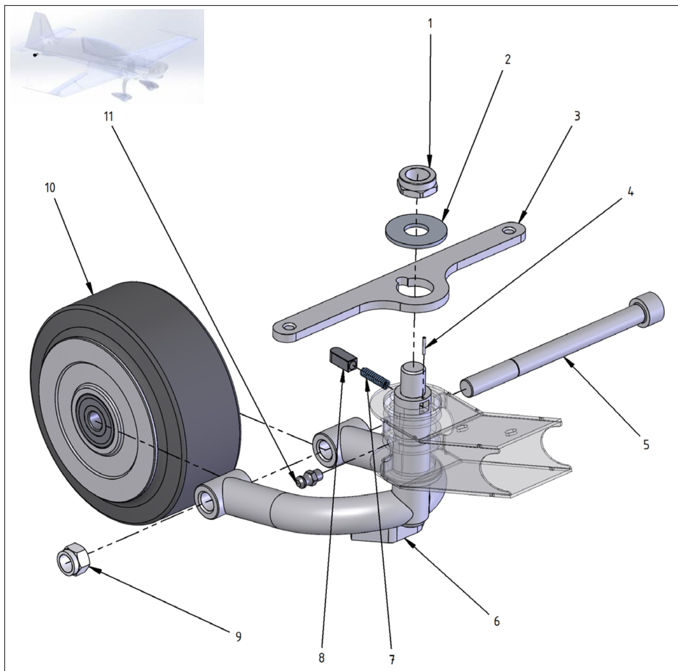
Figure 32-5 Main Gear – Tail Wheel Fork with Wheel
