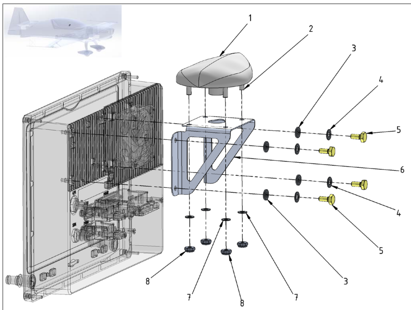
Figure 31-8 Garmin GDU 450 Antenna
