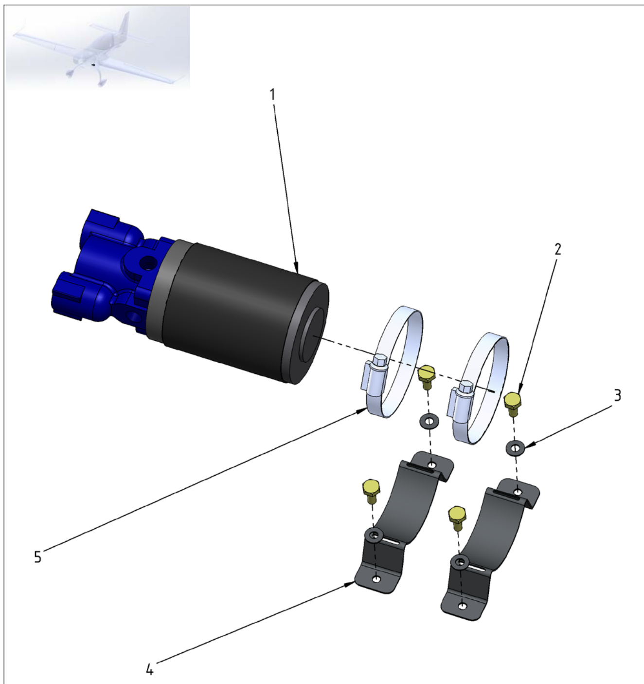
Figure 28-13 Distribution – Boost Pump
