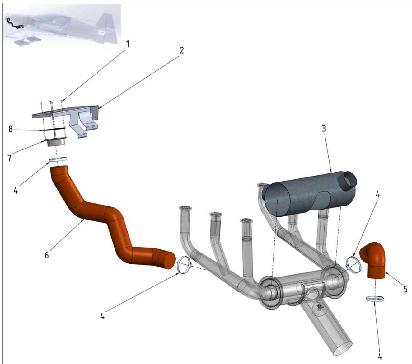
Figure 21-1 Air Routing
