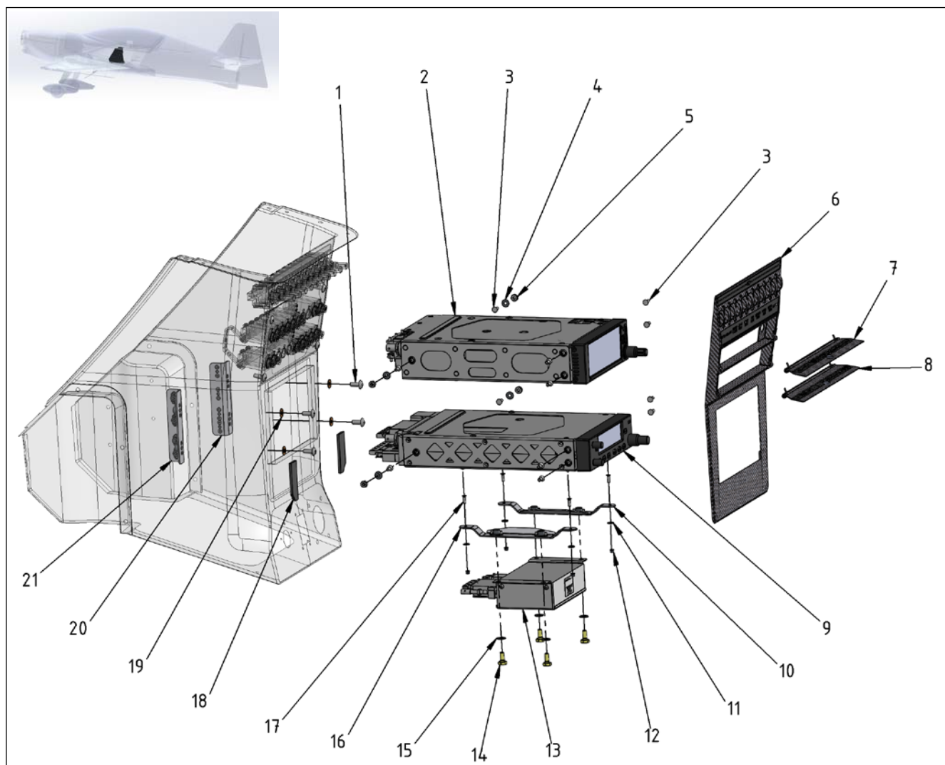
Figure 31-6 Center Console Options – GNX 375 + GTR 225A
