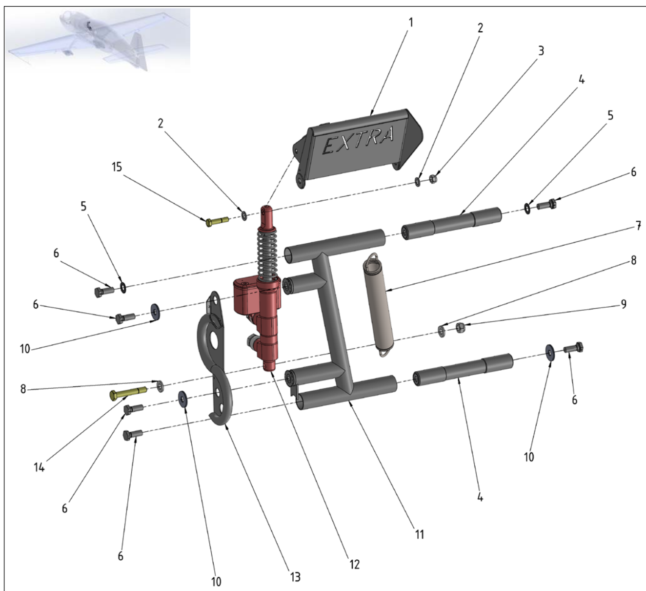
Figure 27-27 Front Pedal RH - Pedal
