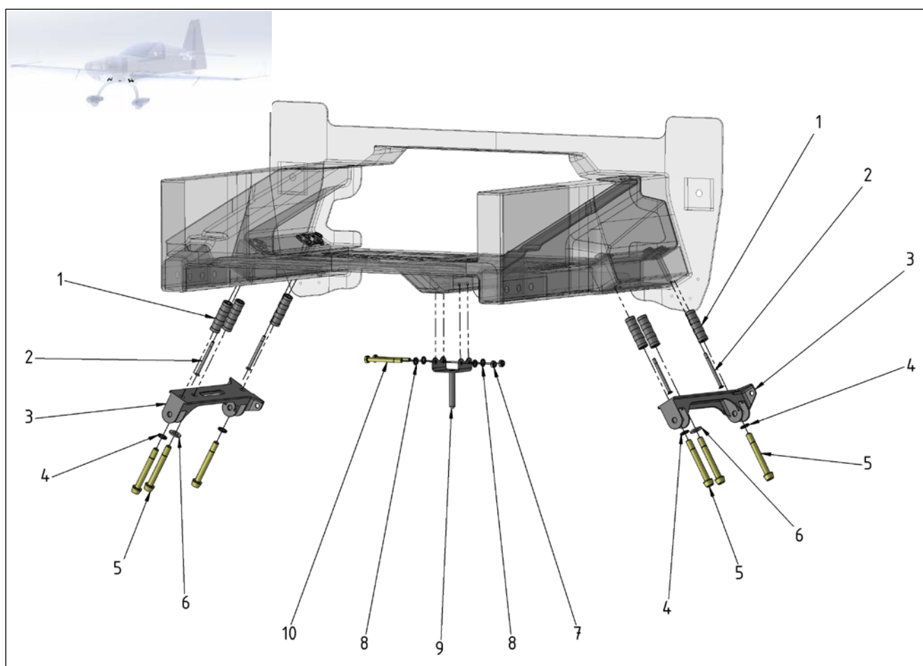
Figure 32-2 Main Gear - Landing Gear Brackets
