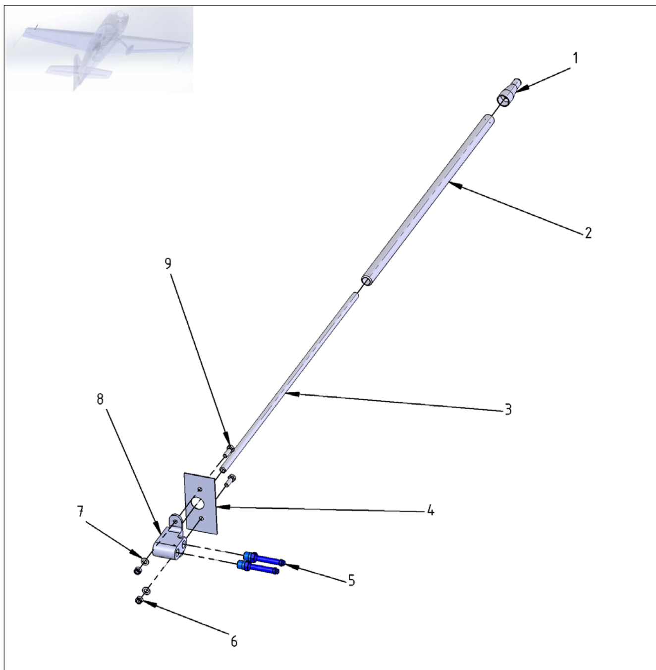
Figure 34-1 Environment Data – Pitot Tube
