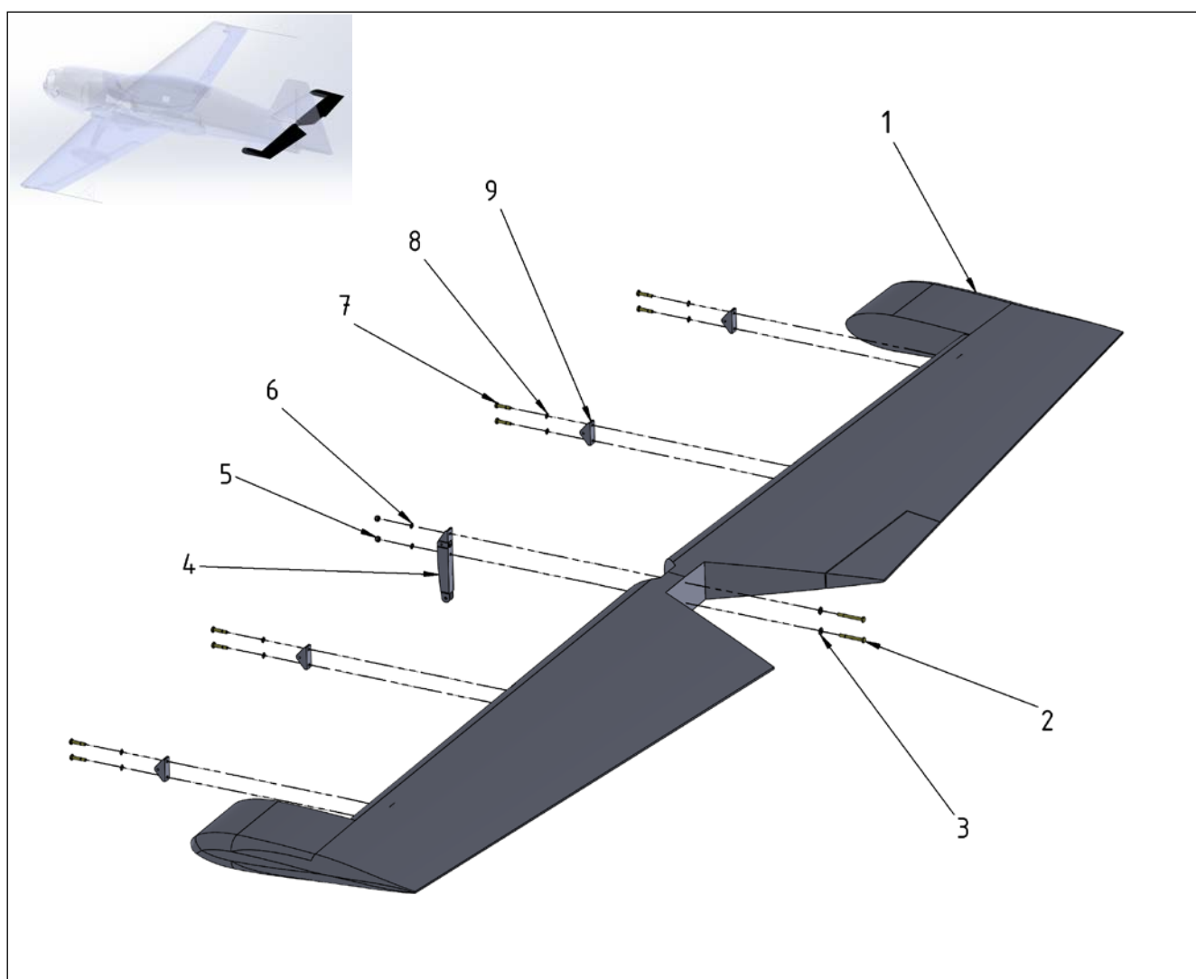
Figure 27-36 Elevator & Tab - Elevator
