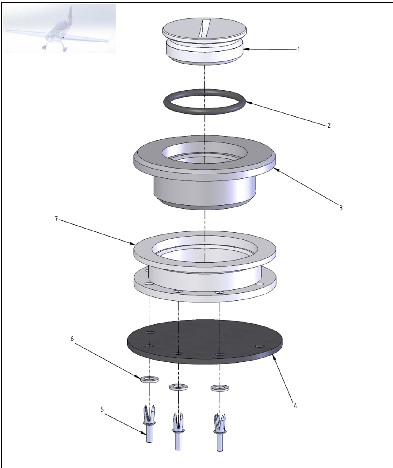
Figure 28-6 Storage – Wing Tank Filler Neck with Sealing Lip
