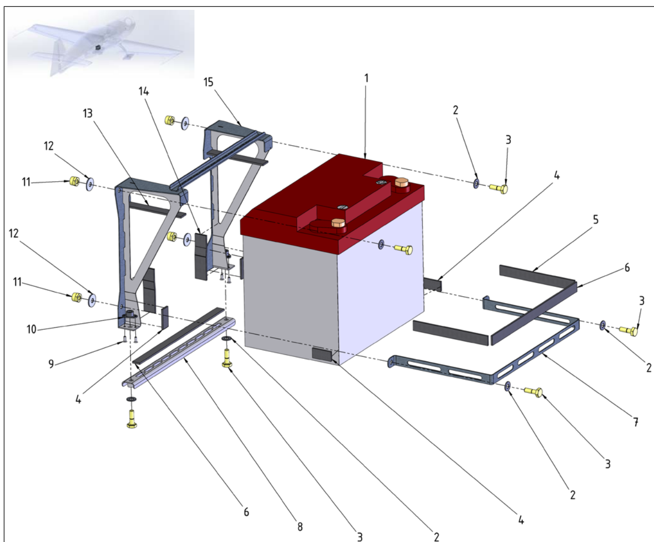
Figure 24-1 Battery System
