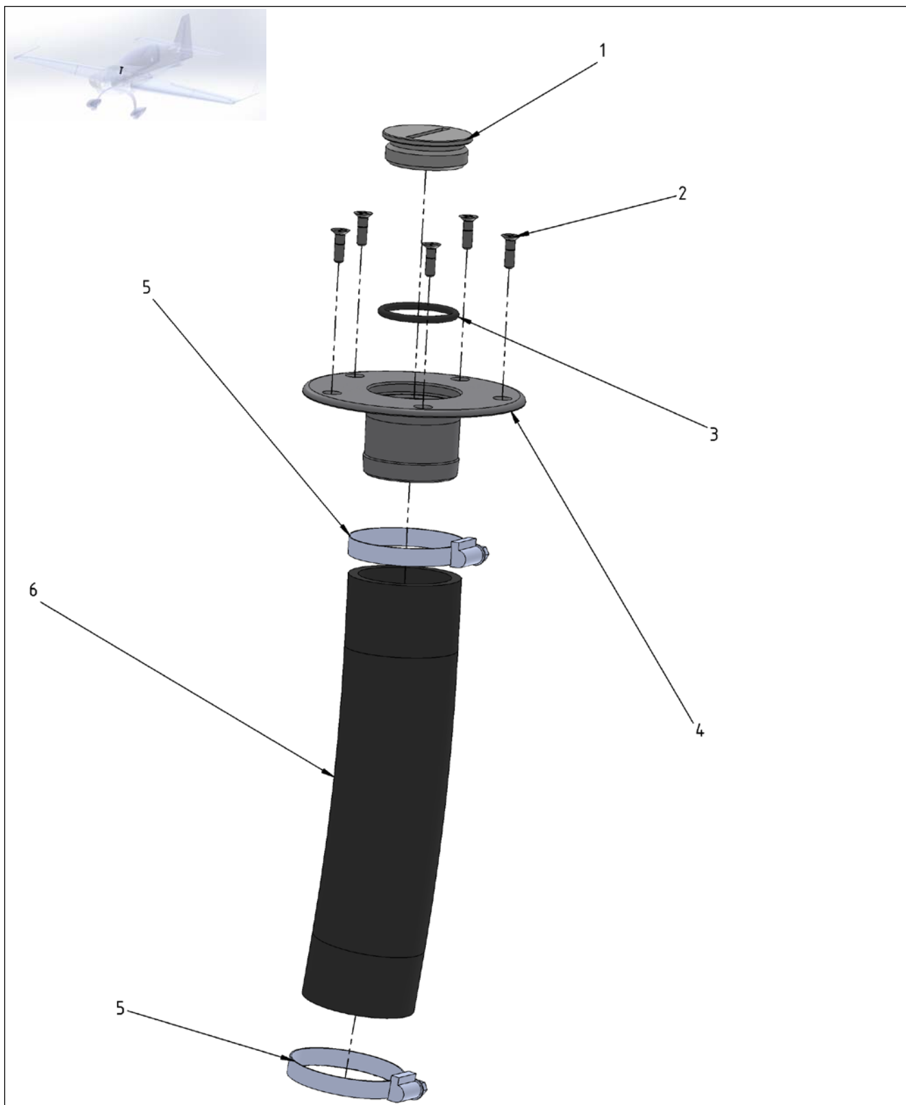
Figure 28-5 Storage – Center Tank Filler Neck
