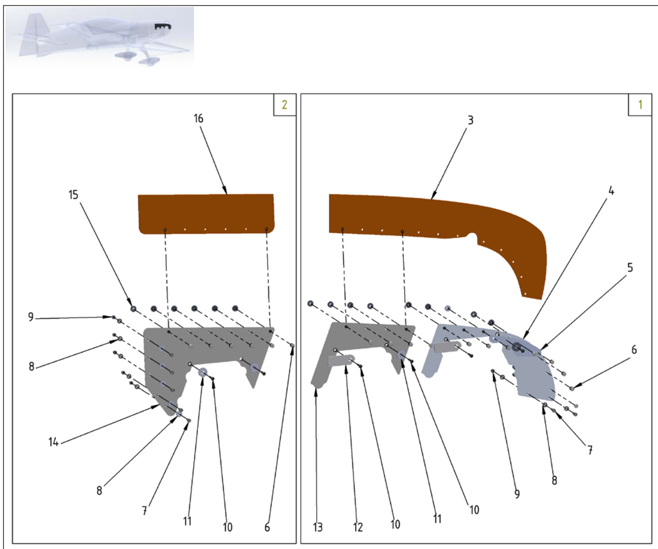
Figure 71-6 Air Baffles – Air Baffles RH
