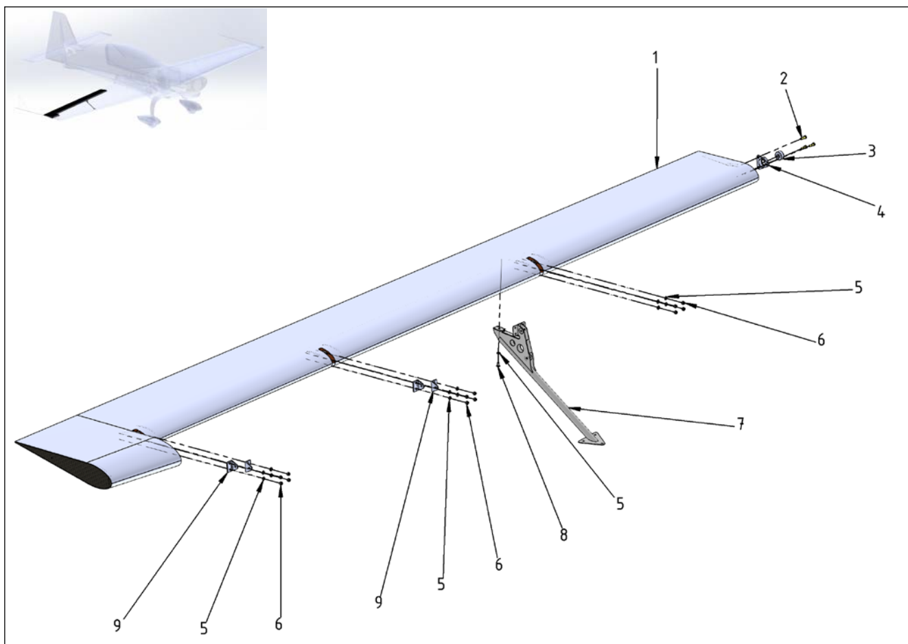
Figure 27-17 Ailerons – Aileron (Standard) RH
