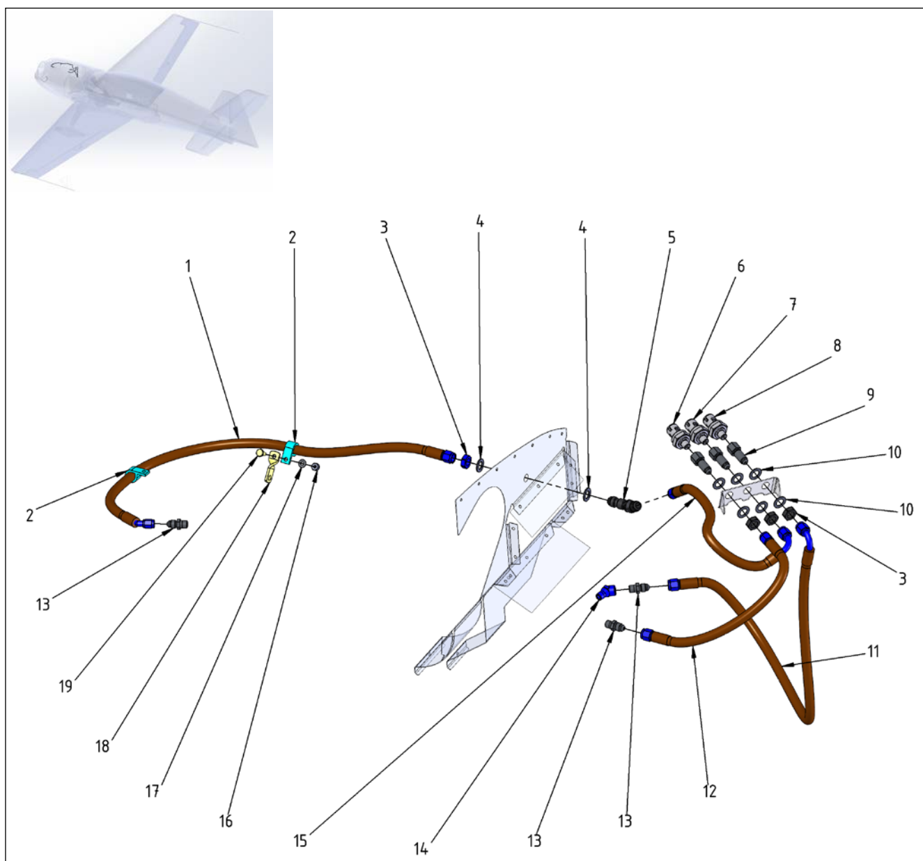
Figure 77-3 Sense Lines Engine Compartment
