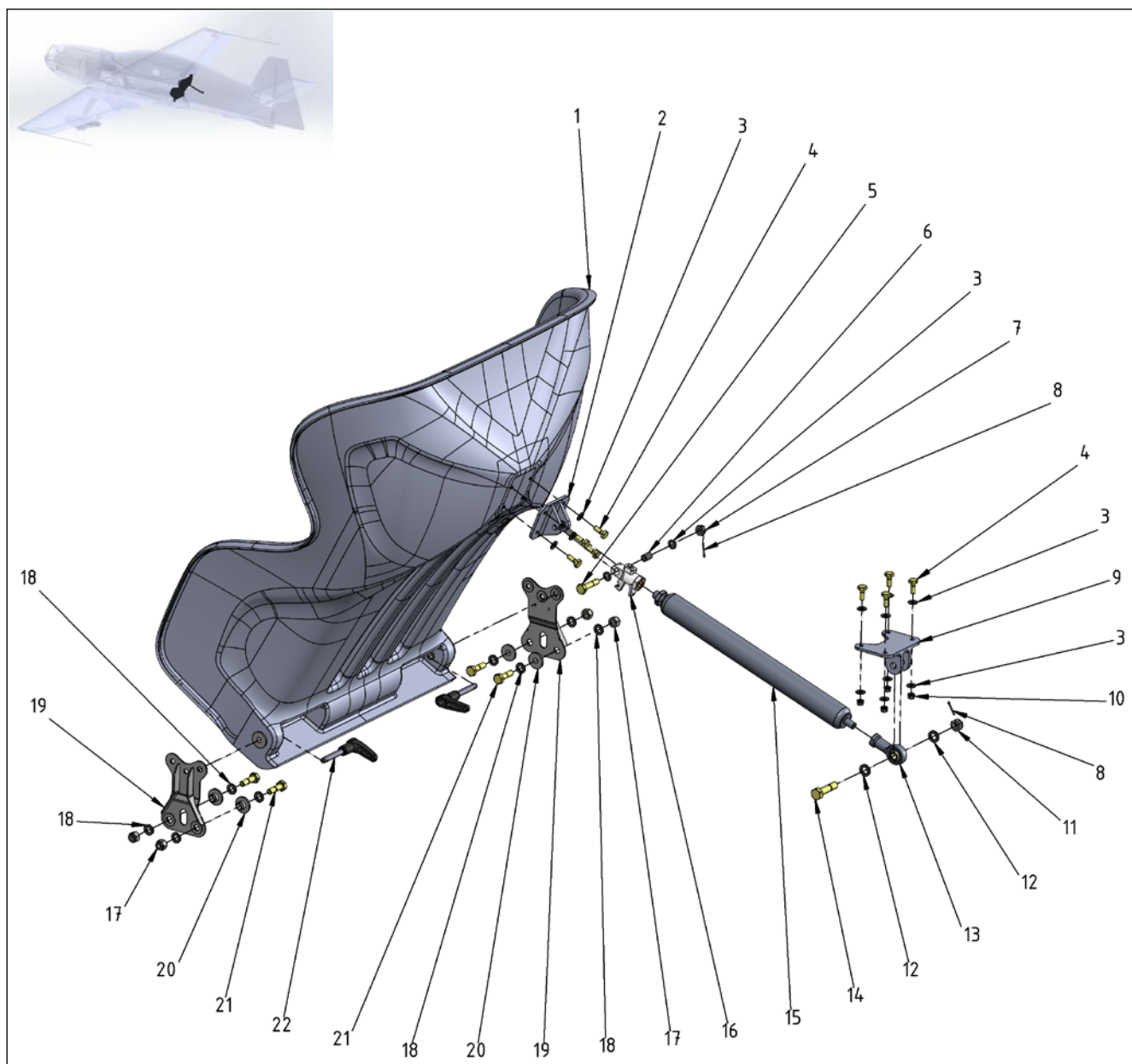
Figure 25-1 Rear Seat Backrest
