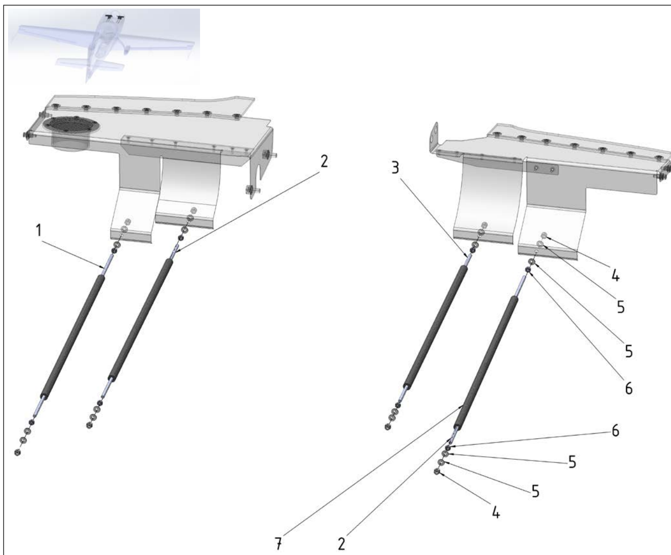
Figure 71-9 Air Baffles – Air Baffle Rods
