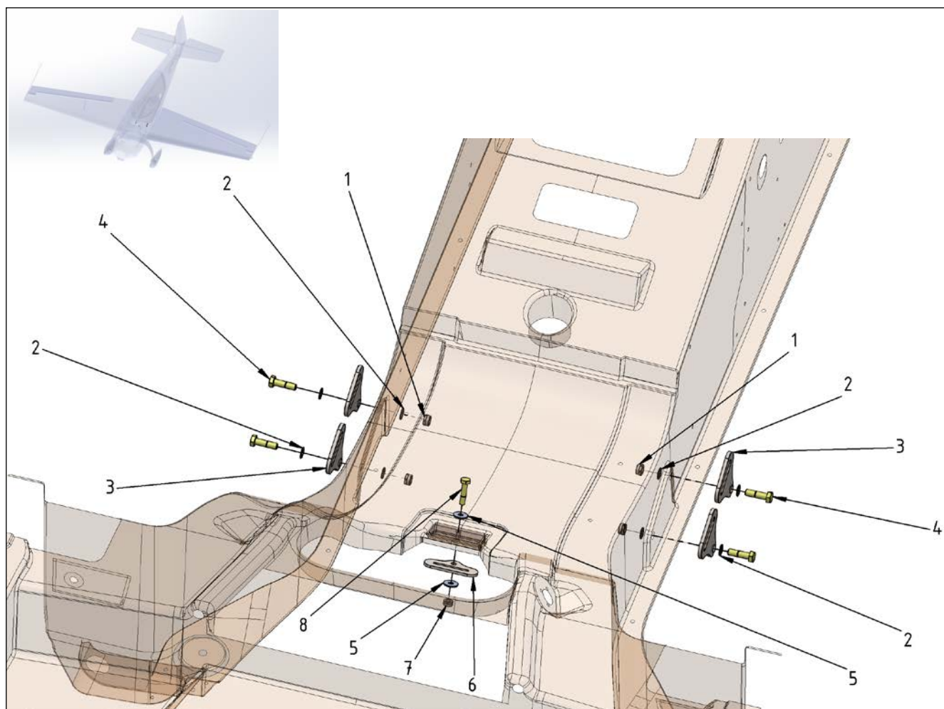
Figure 25-14 Copilot Seat and Crotch Belt Attachment
