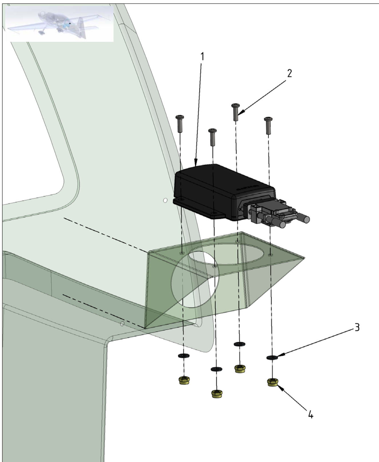
Figure 34-3 Attitude and Direction – Garmin GMU 11 Magnetometer
