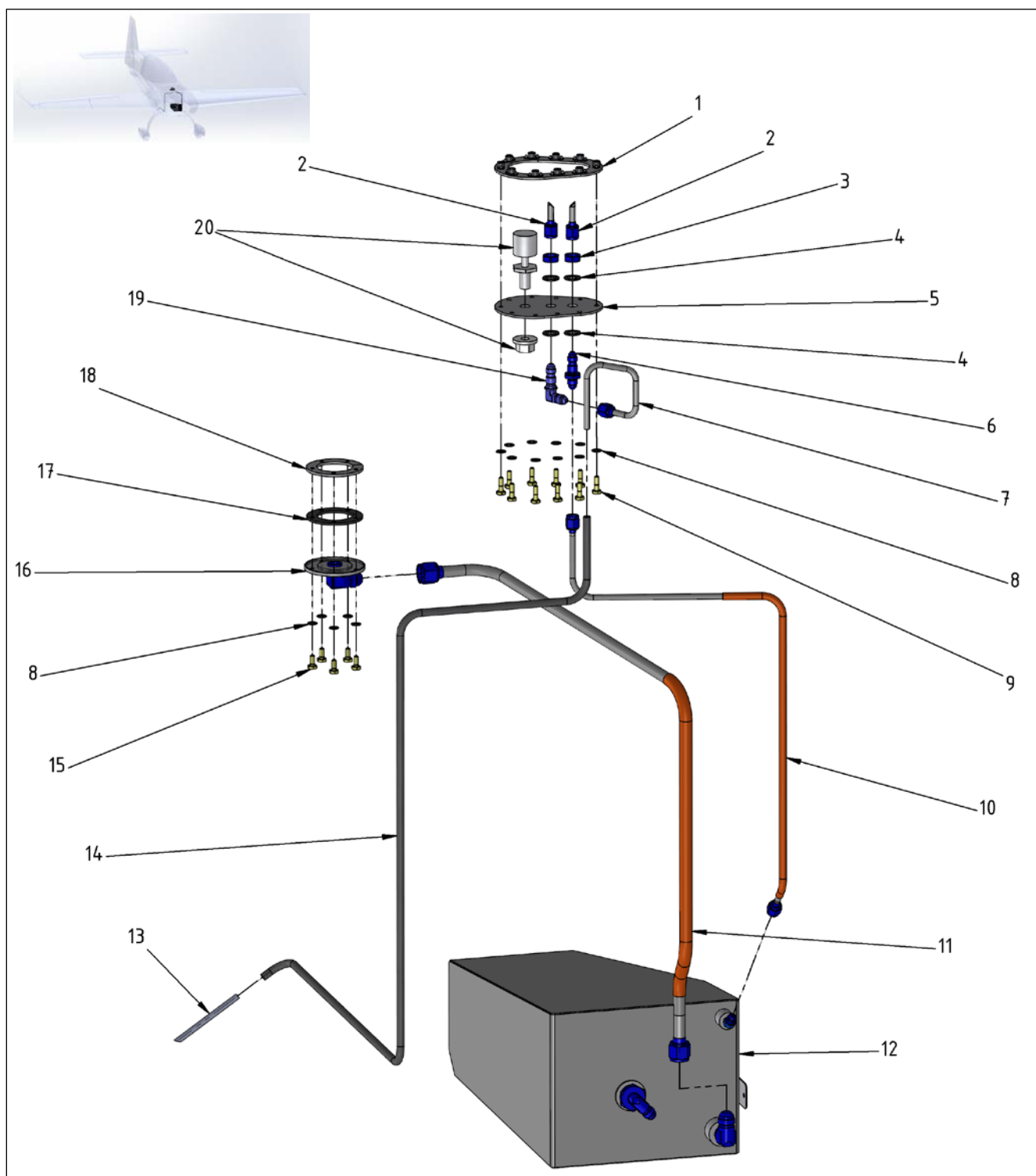
Figure 87-1 Smoke - Storage
