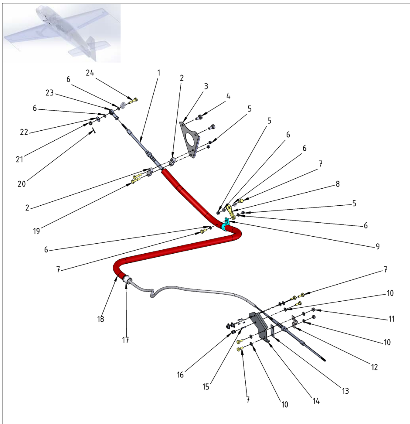
Figure 73-1 Controlling – Throttle Control Cable
