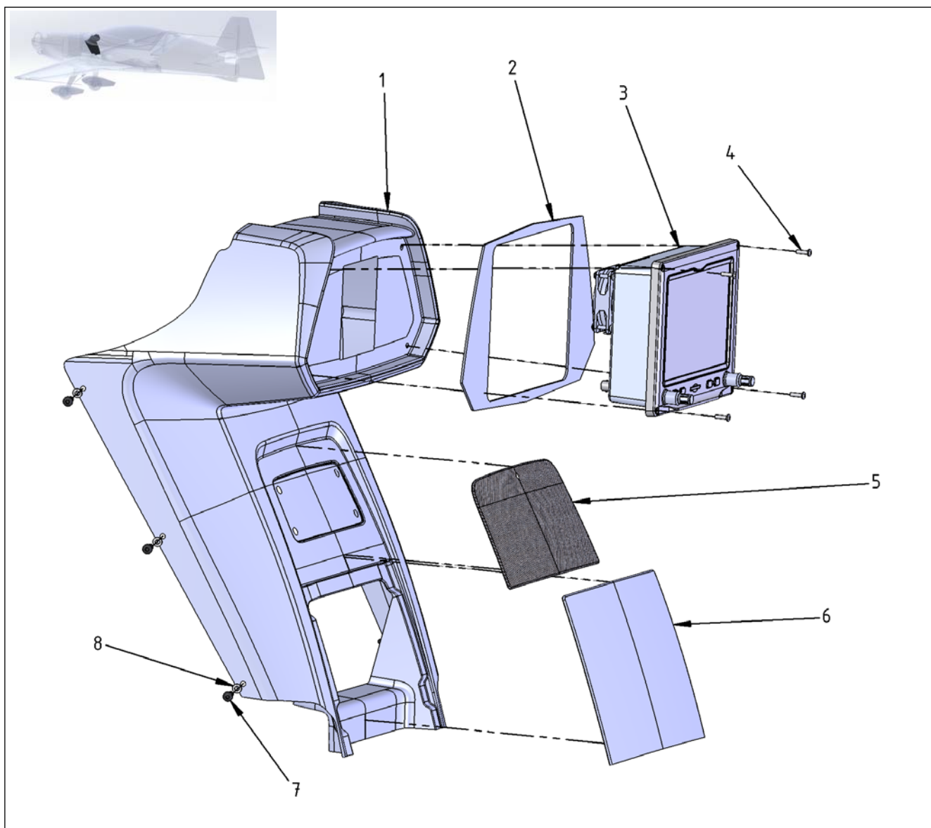
Figure 31-2 Instrument and Control Panels – Front Instrument Panel with GDU 450
