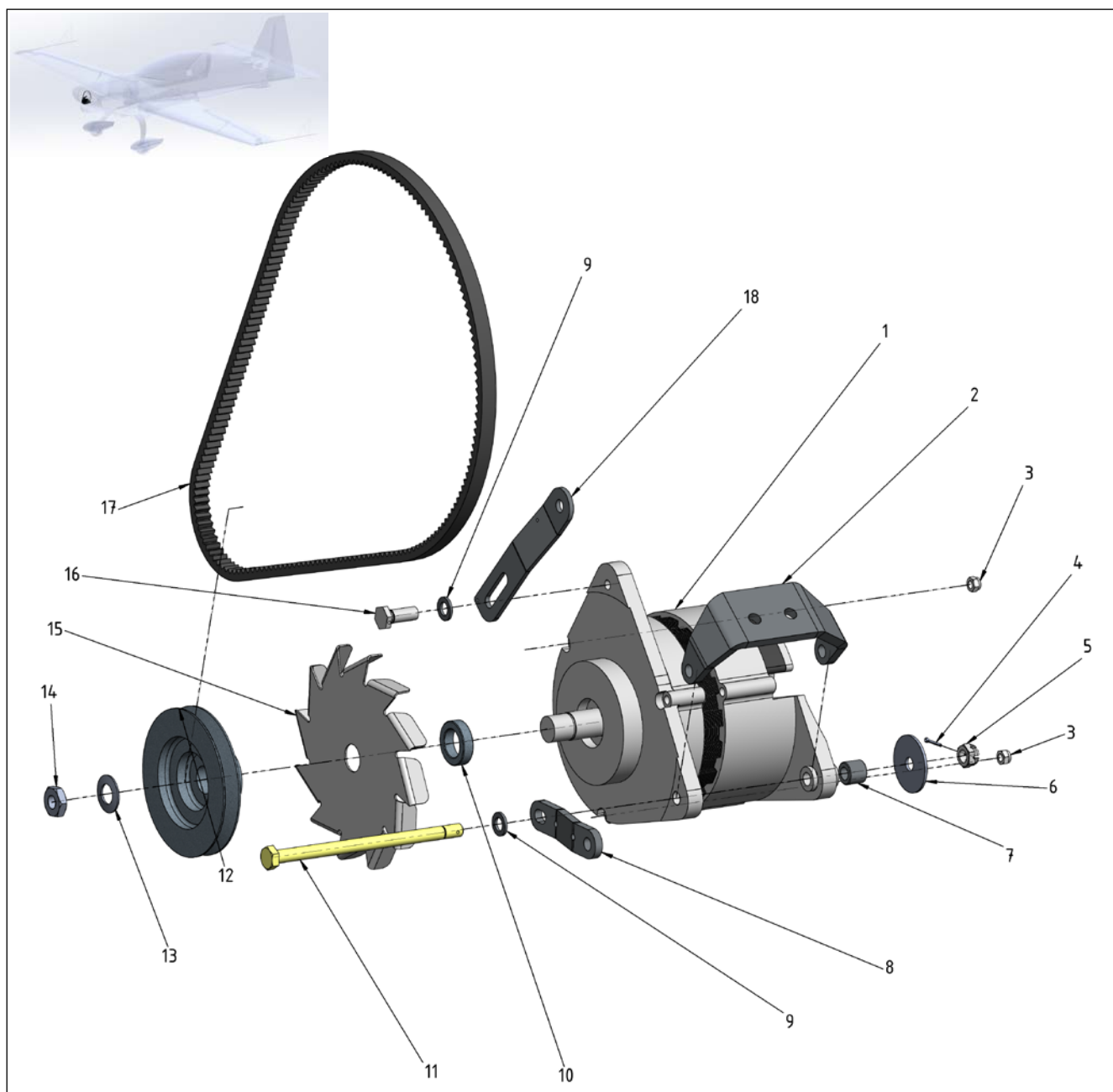
Figure 24-3 Alternator System 65A
