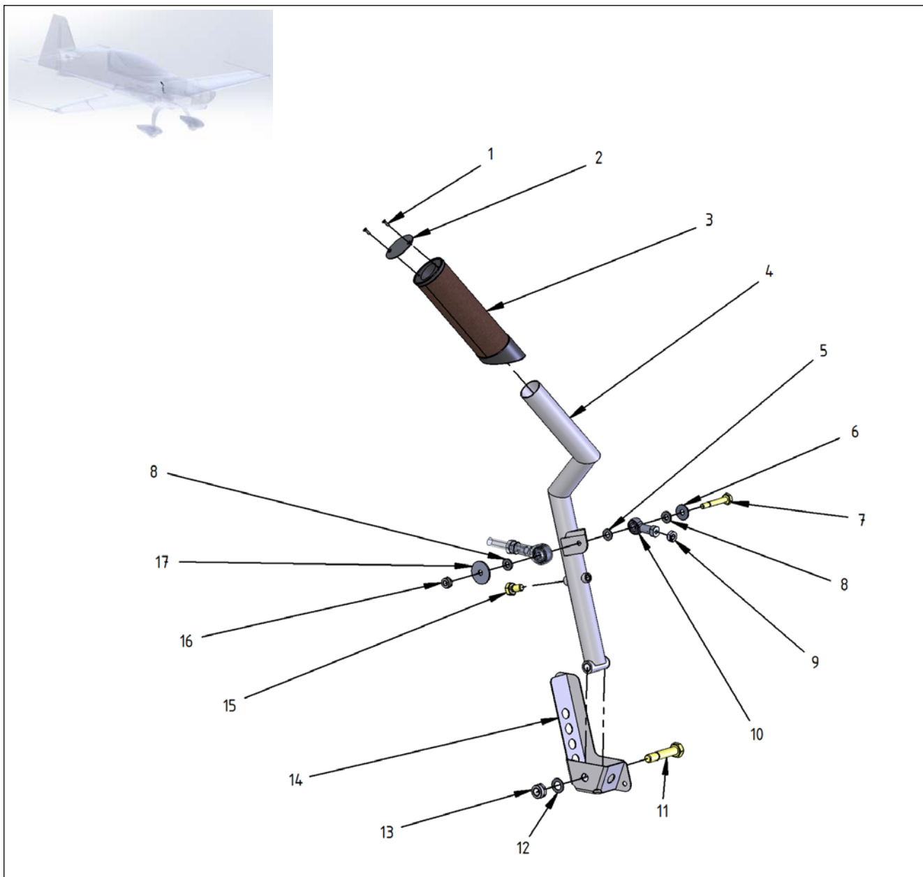
Figure 73-2 Throttle Control Lever – Control Lever FWD
