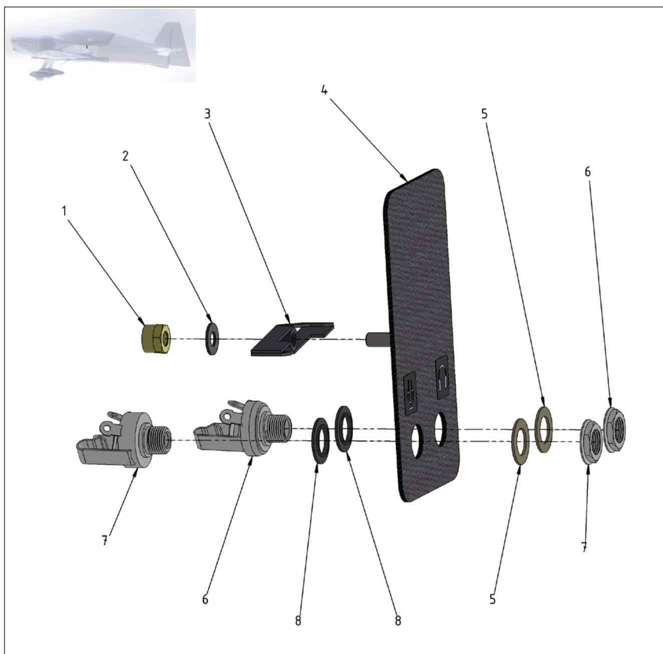
Figure 25-5 Control Panel (Pilot) - Standard
