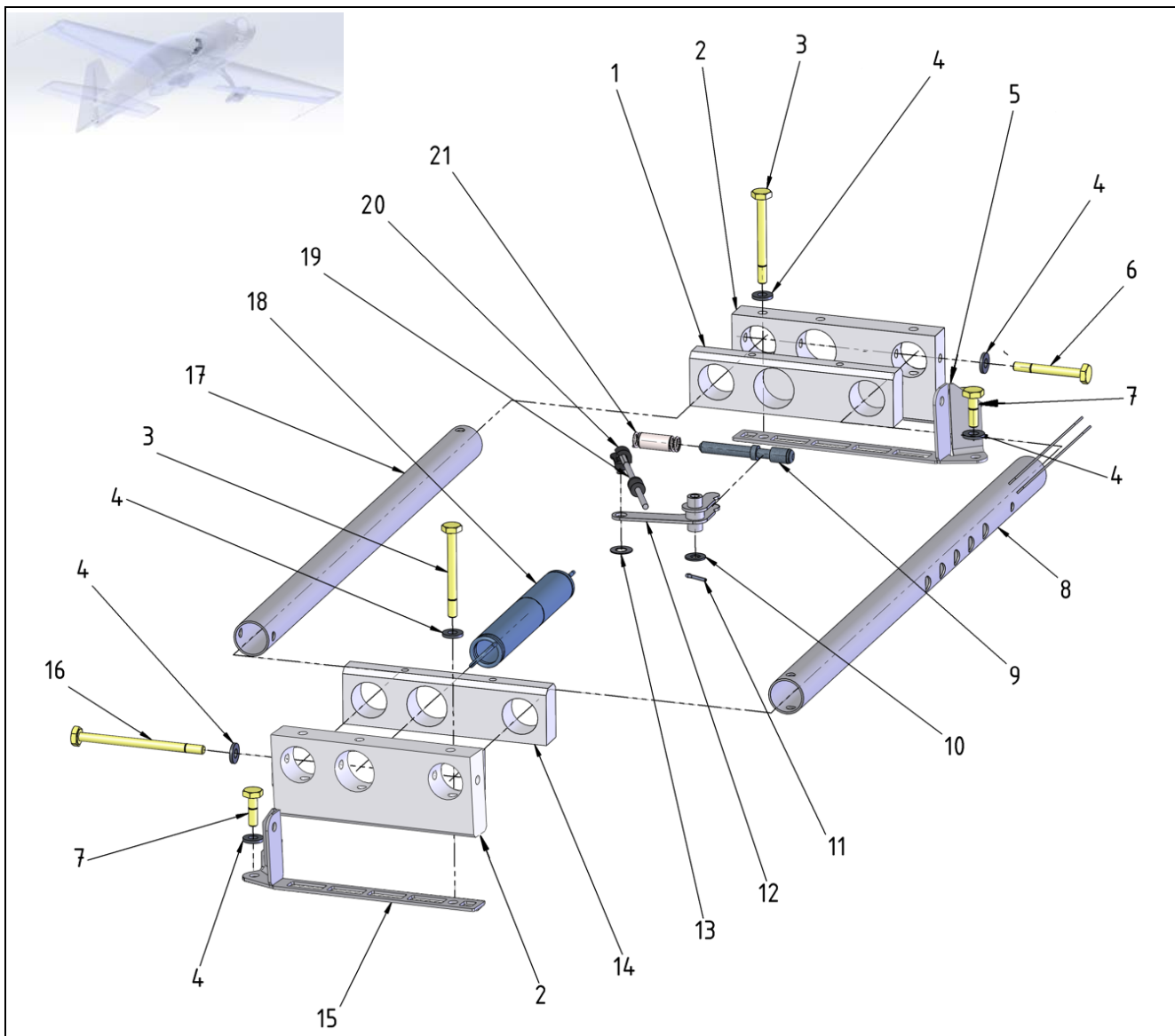
Figure 27-27 Front Pedal LH - Raised Base
