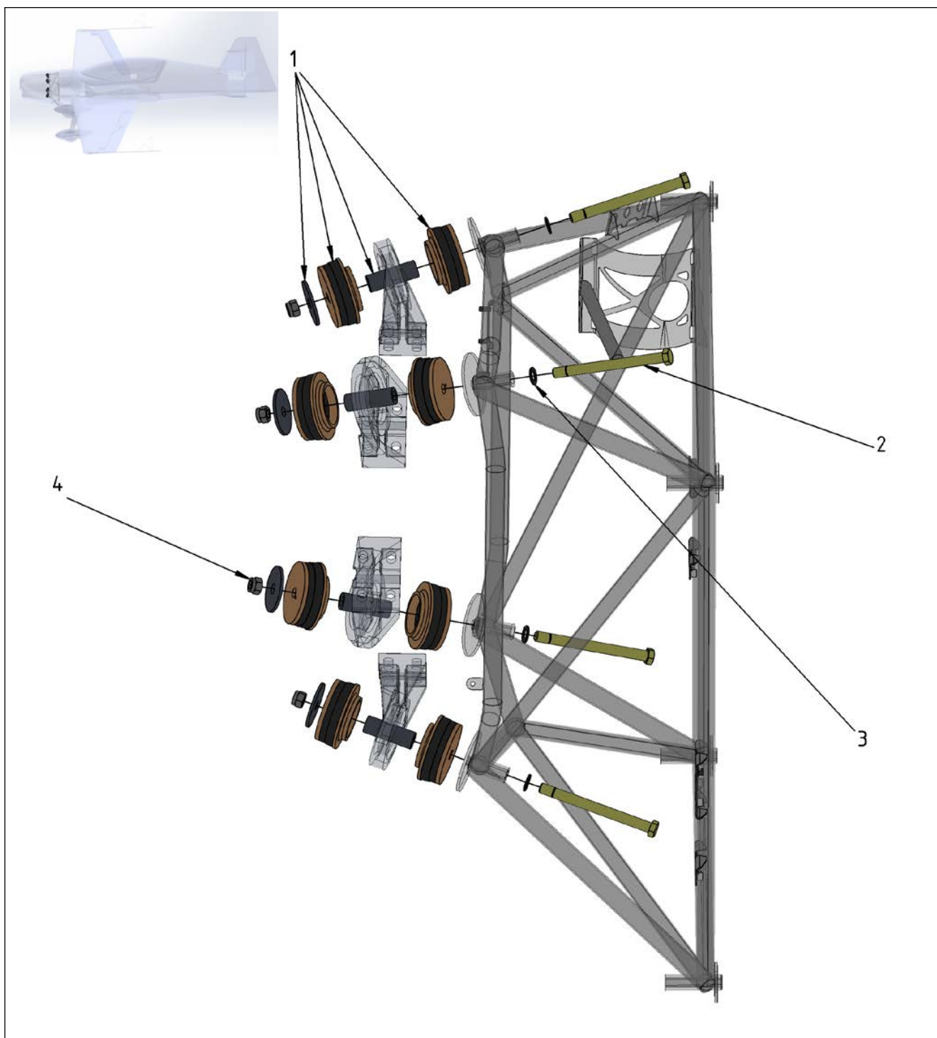
Figure 71-3 Shock Mounts
