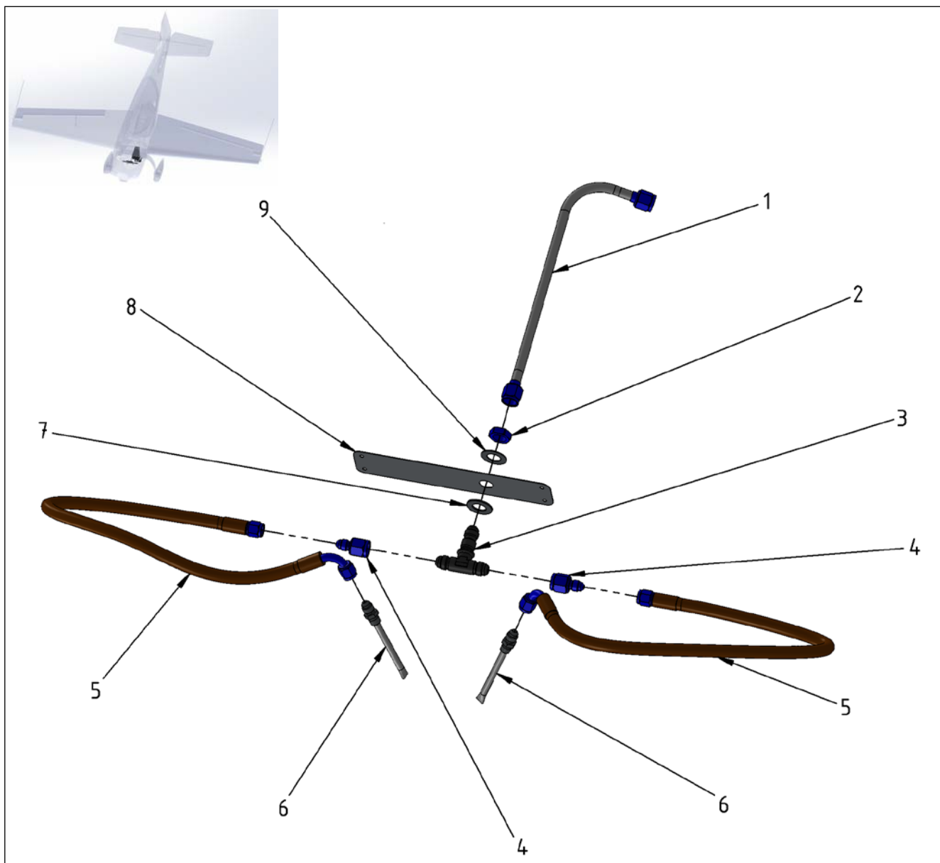
Figure 87-4 Smoke - Injection Chabord
