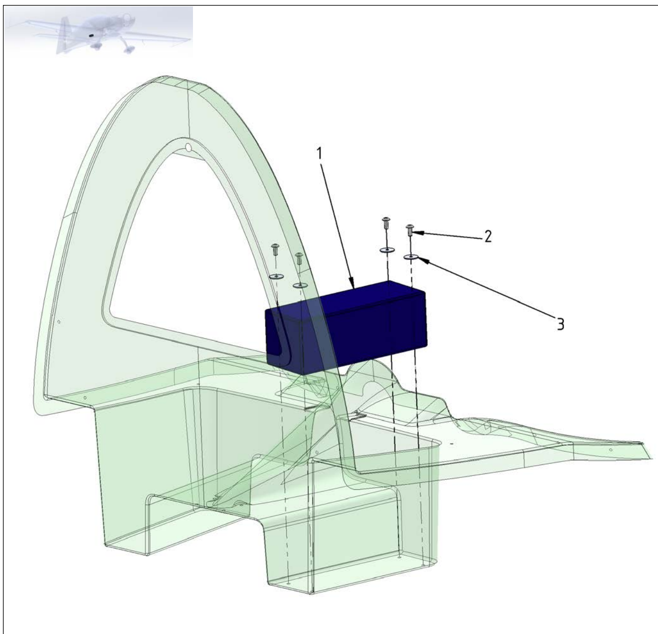
Figure 25-18 First Aid Kit
