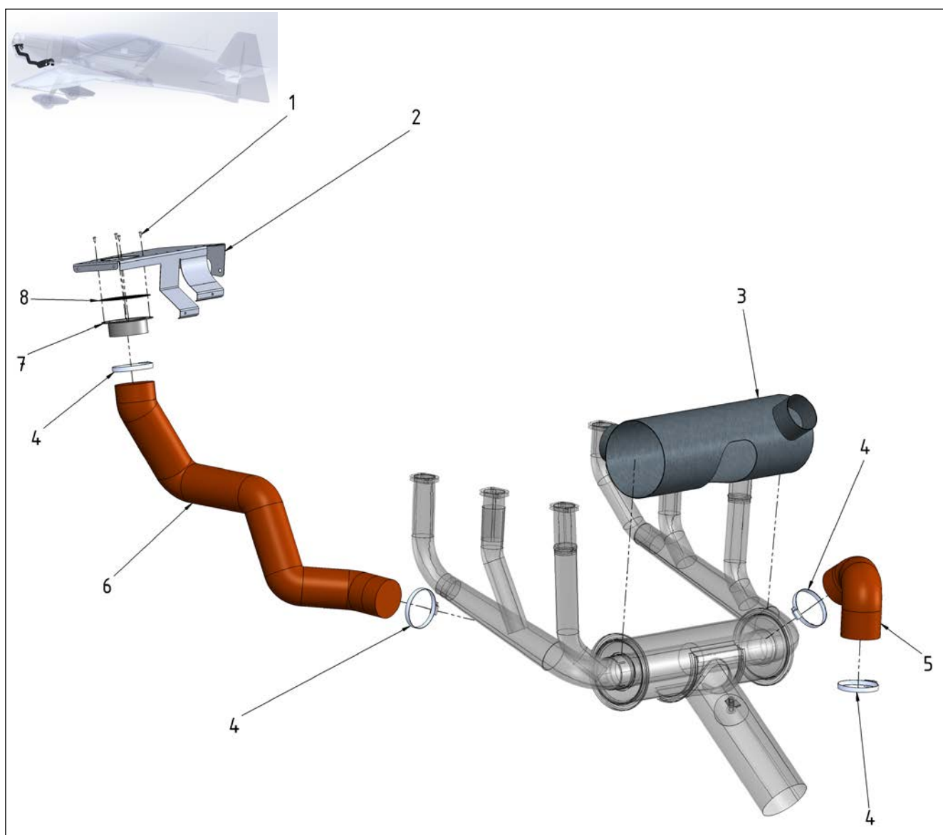
Figure 21-1 Air Routing
