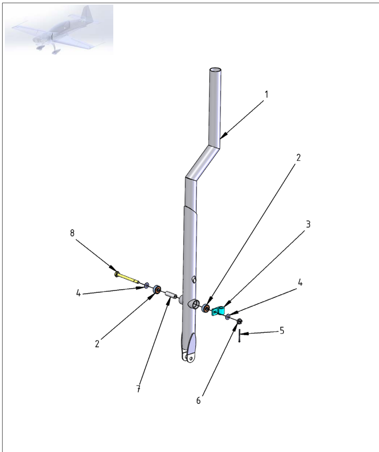
Figure 27-5 Front Control Stick
