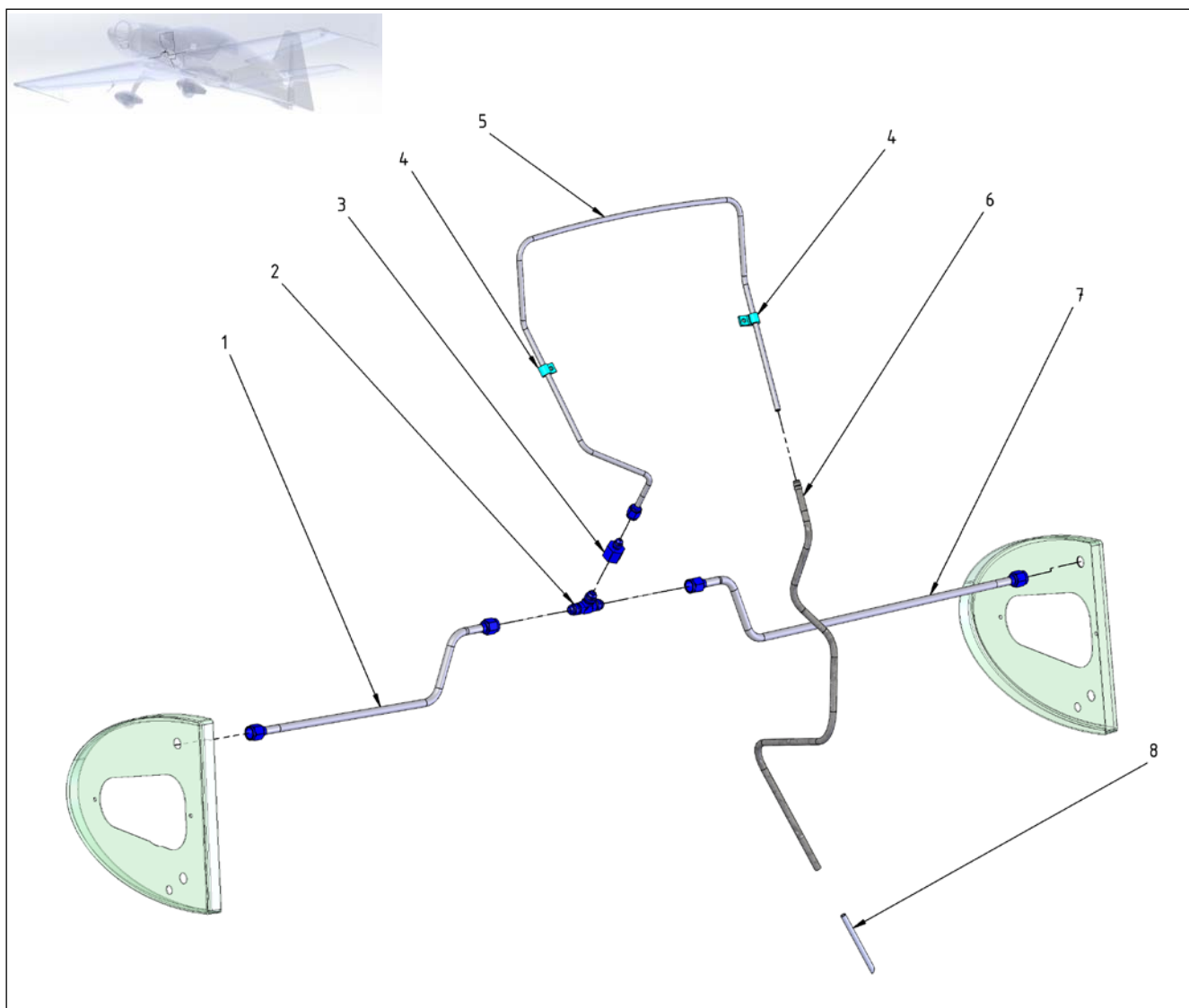
Figure 28-8 Ventilation Line – Wing Tanks
