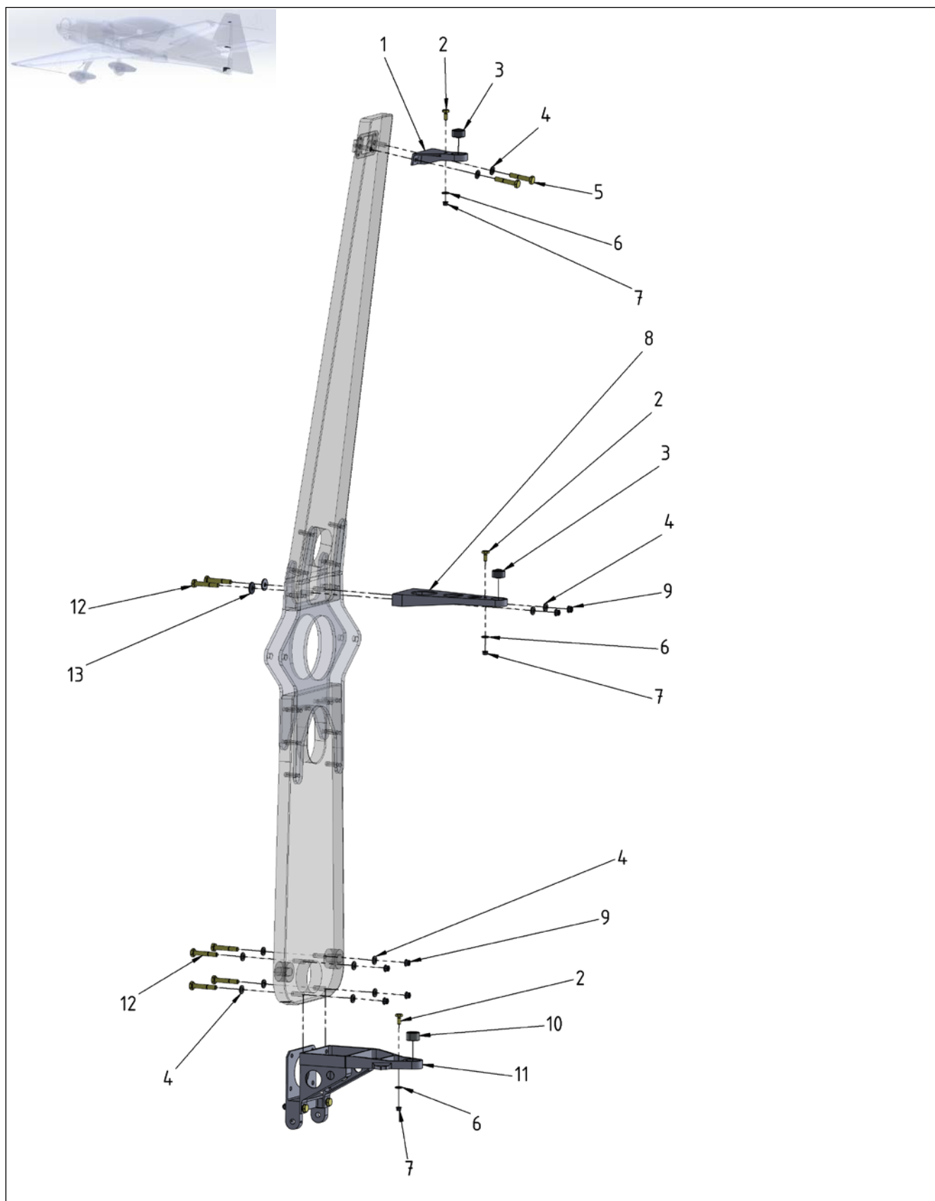
Figure 27-21 Rudder Control – Rudder Bearing
