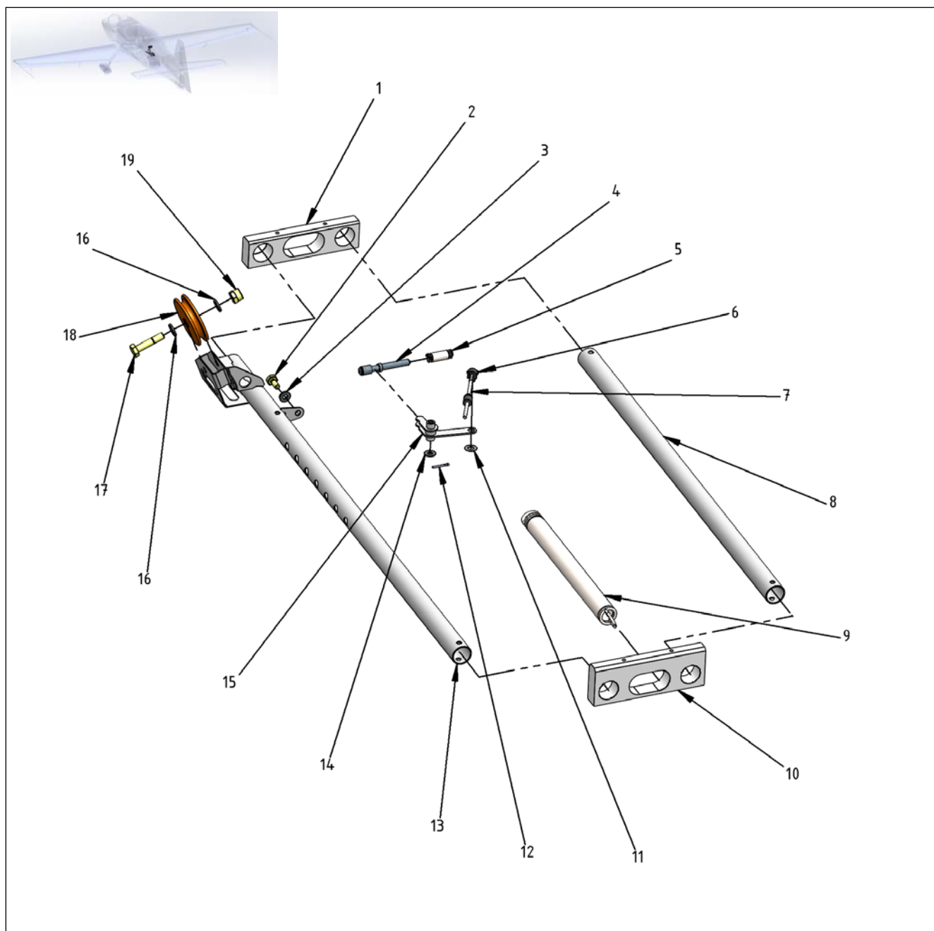
Figure 27-37 Rear Pedal RH - Base
