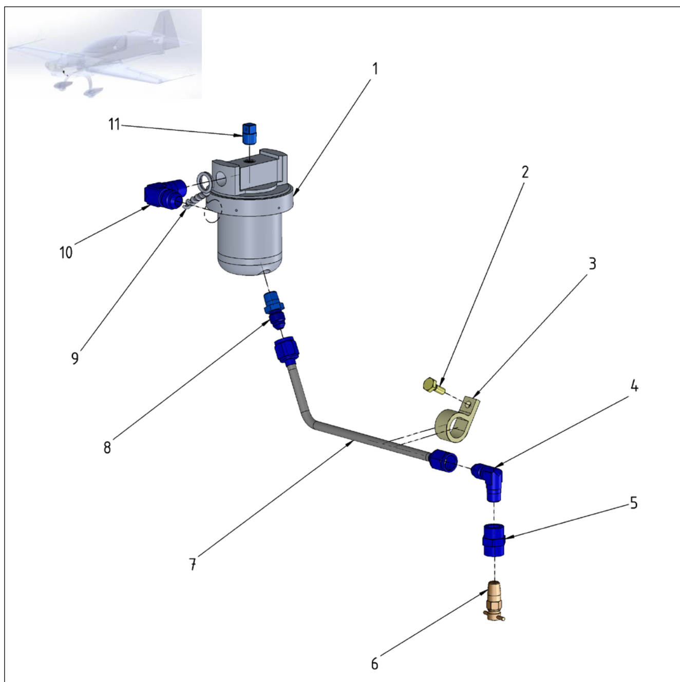
Figure 28-12 Distribution - Gascolator
