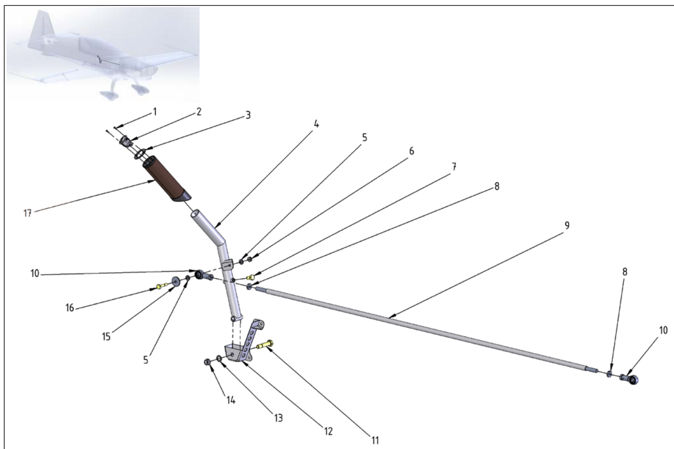
Figure 73-3 Throttle Control AFT with Coupling
