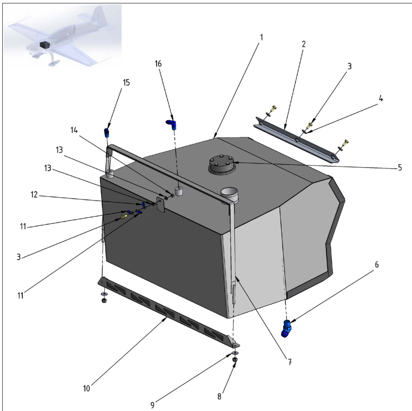
Figure 28-1 Storage – Center Tank
