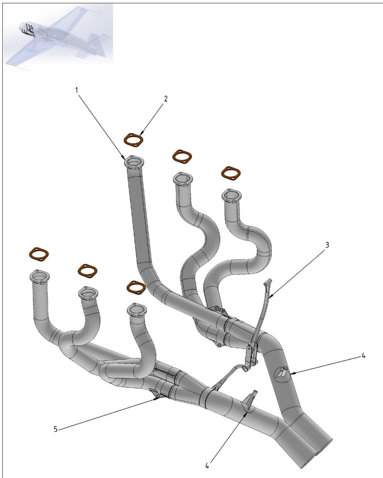
Figure 78-2 Chabord 6 in 2
