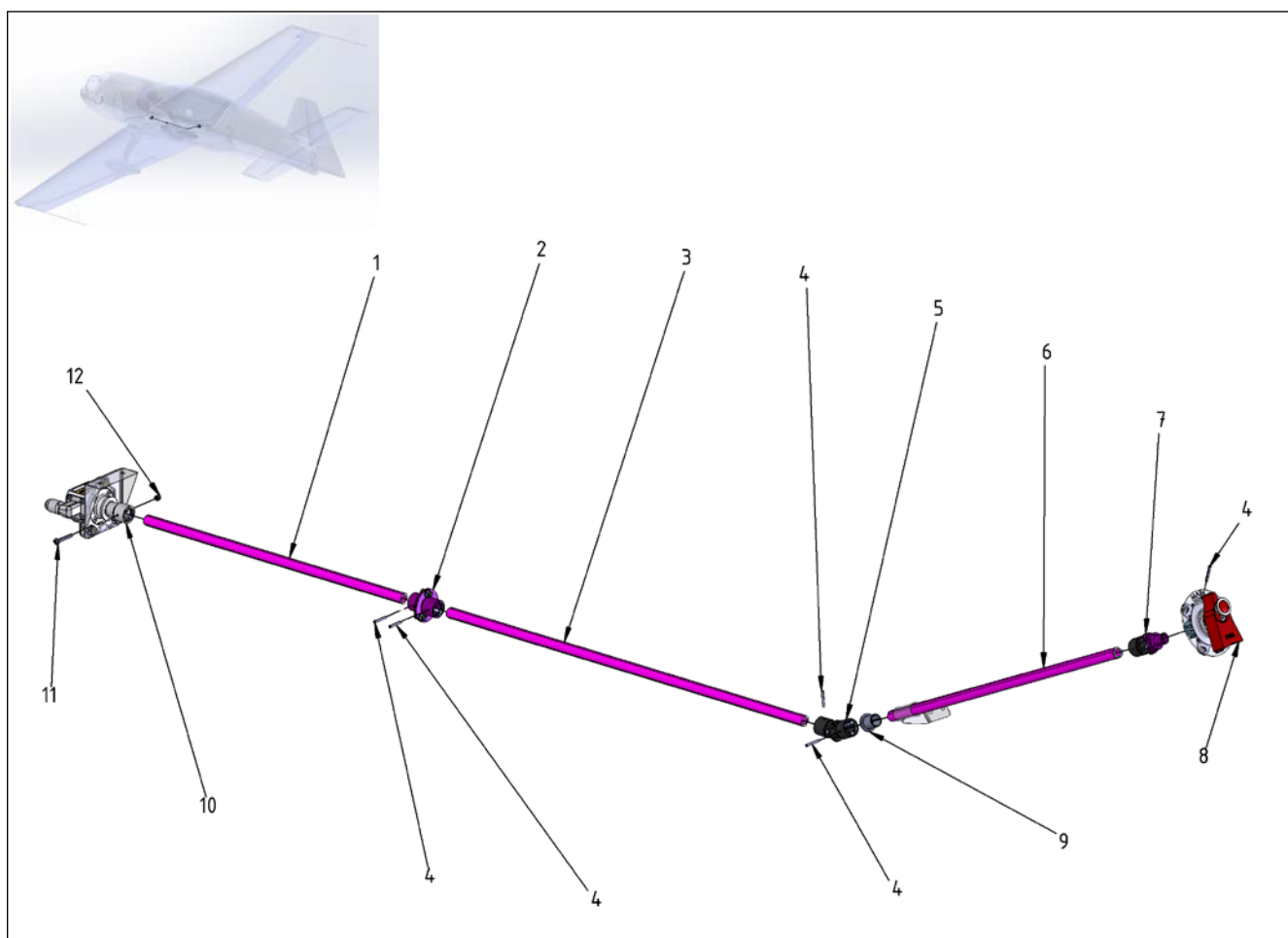
Figure 28-10 Distribution – Fuel Selector Valve/ Control Rods
