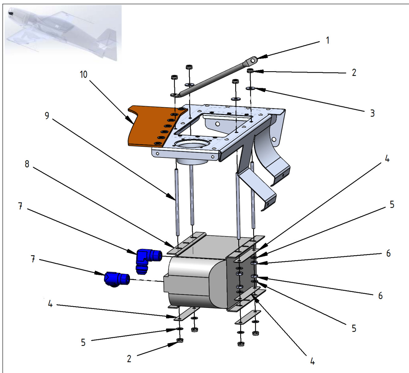
Figure 79-3 Additional Oil Cooler
