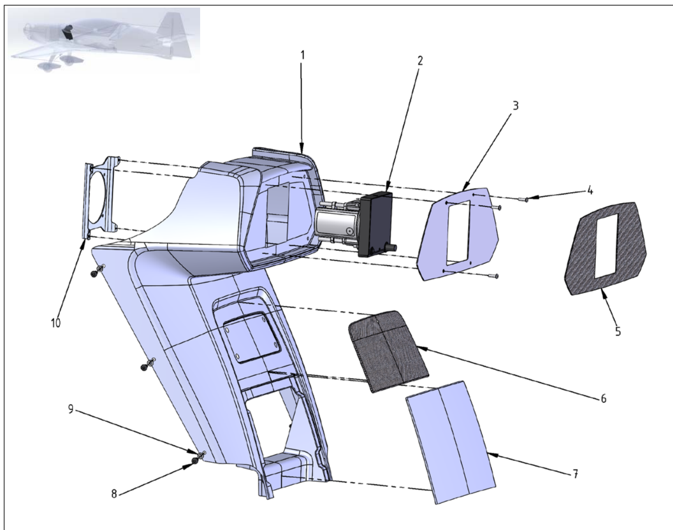
Figure 31-1 Instrument and Control Panels – Front Instrument Panel
