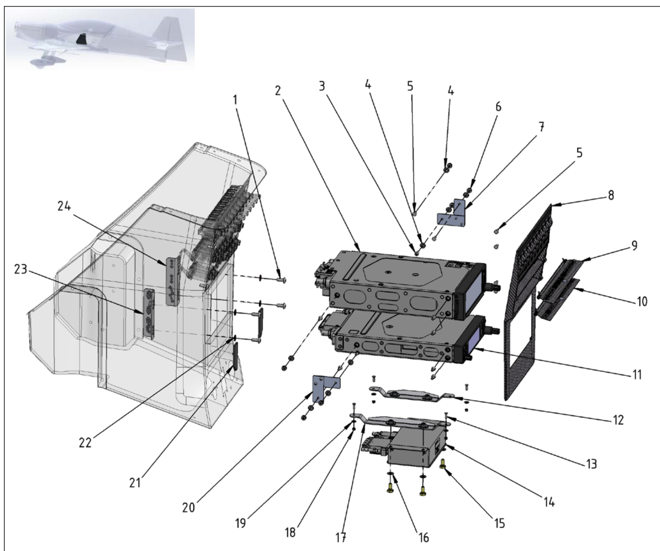
Figure 31-7, Sheet 1 Center Console Options – GNX 375 + GTR 205 + GAD 29 (<089)
