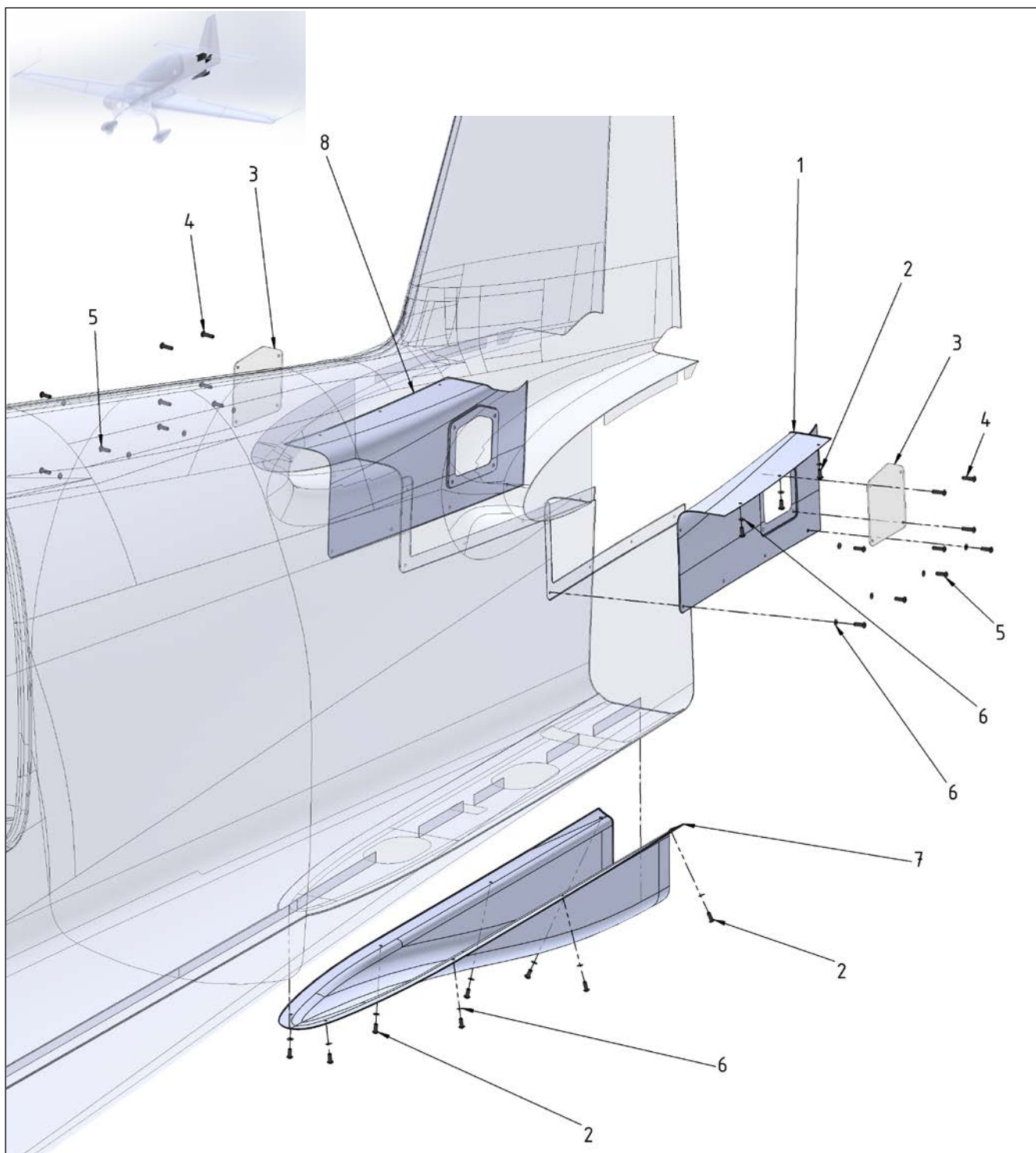
Figure 51-2 Access Panels Tail
