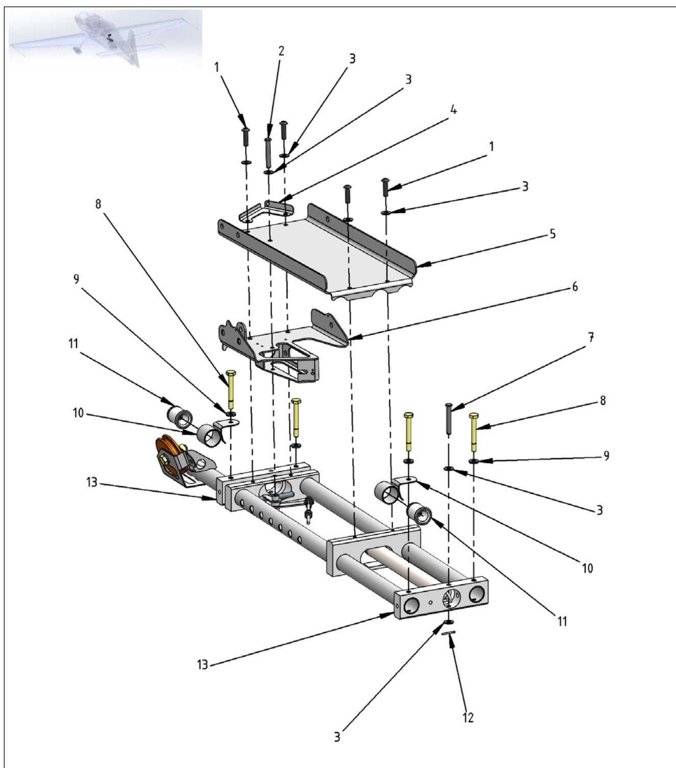
Figure 27-36 Rear Pedal RH - Footrest
