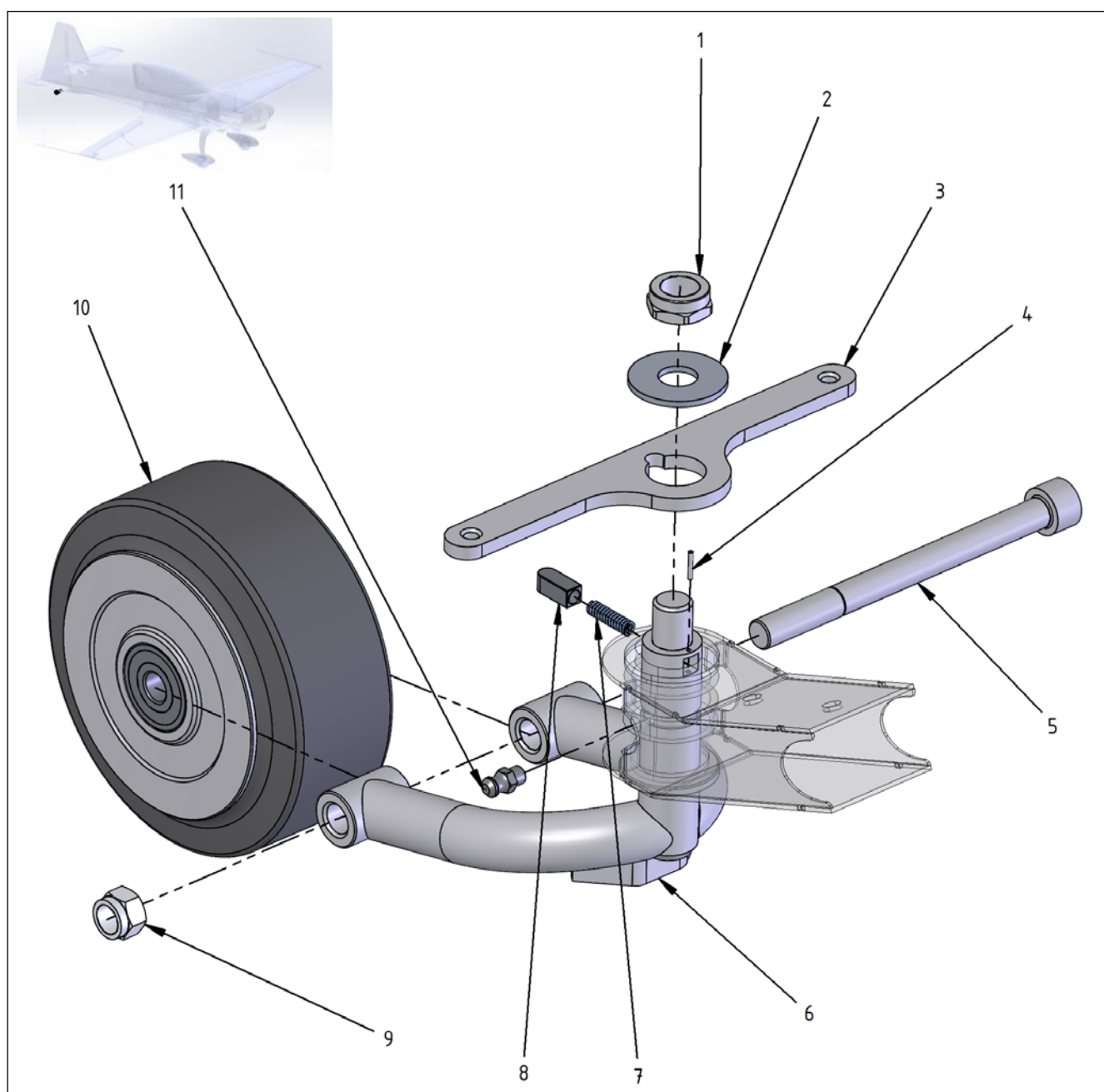
Figure 32-6 Main Gear – Tail Wheel Fork with Wheel
