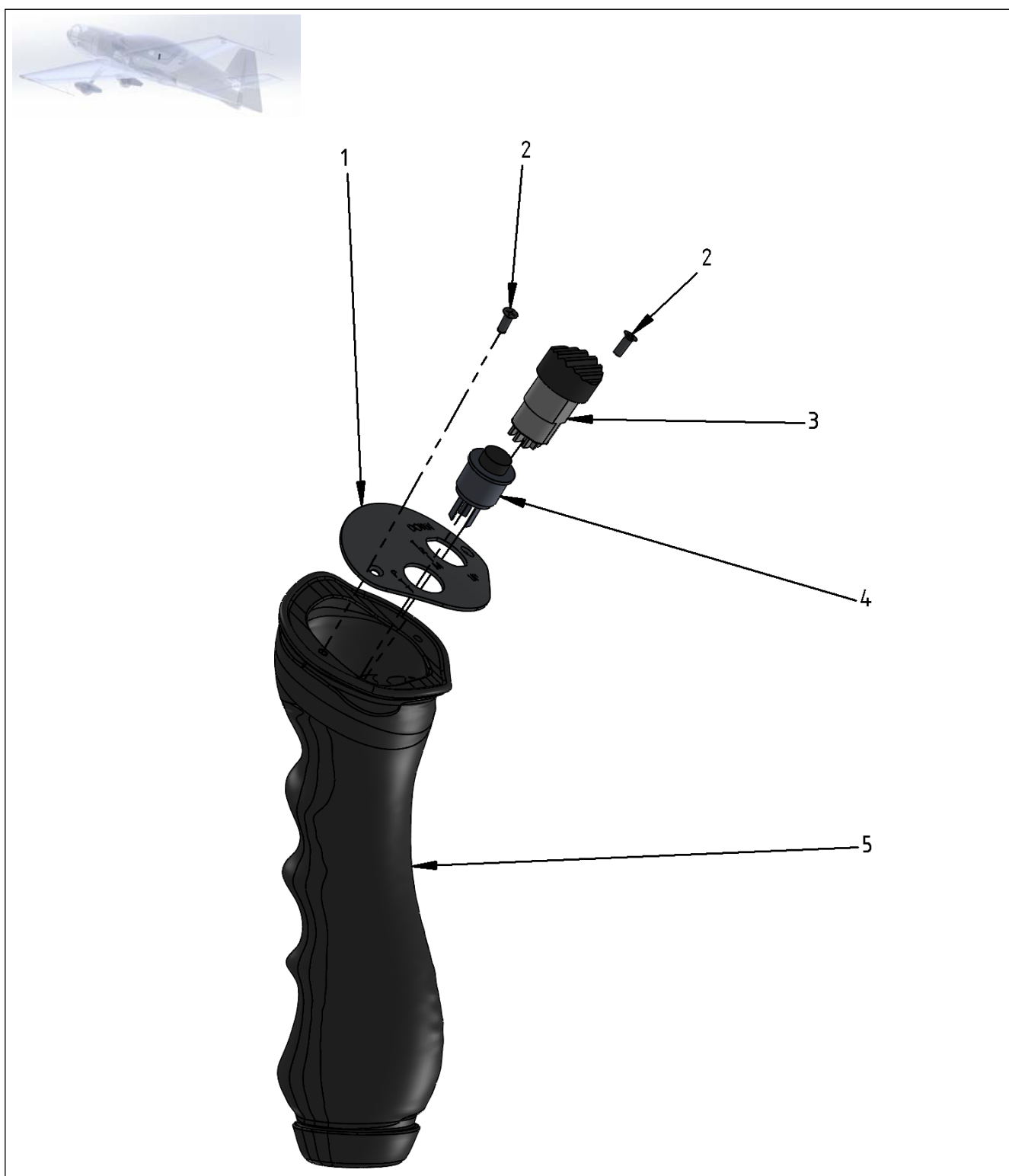
Figure 27-7 Control Stick Covers – Pilot Standard Configuration
