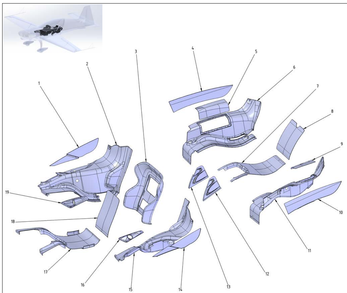
Figure 25- 3 Panels
