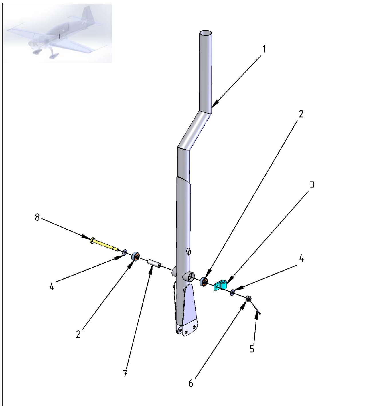
Figure 27-6 Rear Control Stick
