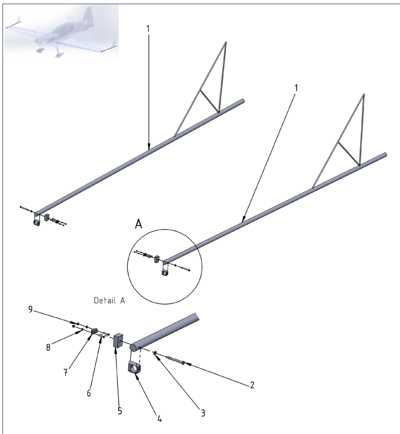
Figure 57-2 Sighting Device for Standard Ailerons
