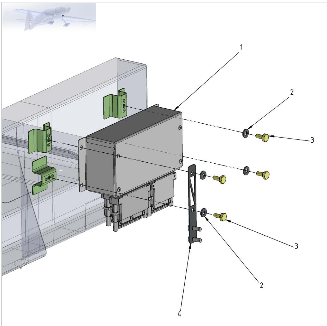
Figure 77-1 Integrated Engine Instrument Systems – Garmin GEA-24B EIS
