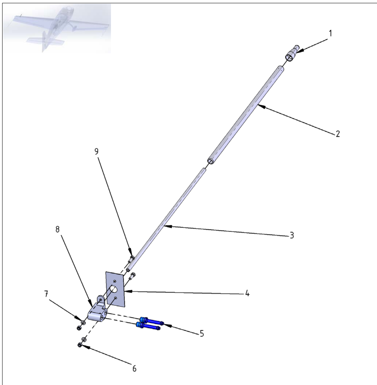
Figure 34-1 Environment Data – Pitot Tube
