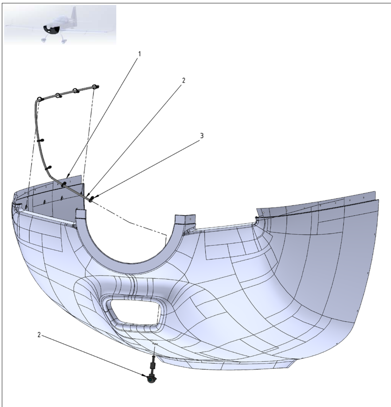
Figure 34-4 Taxi-Cam
