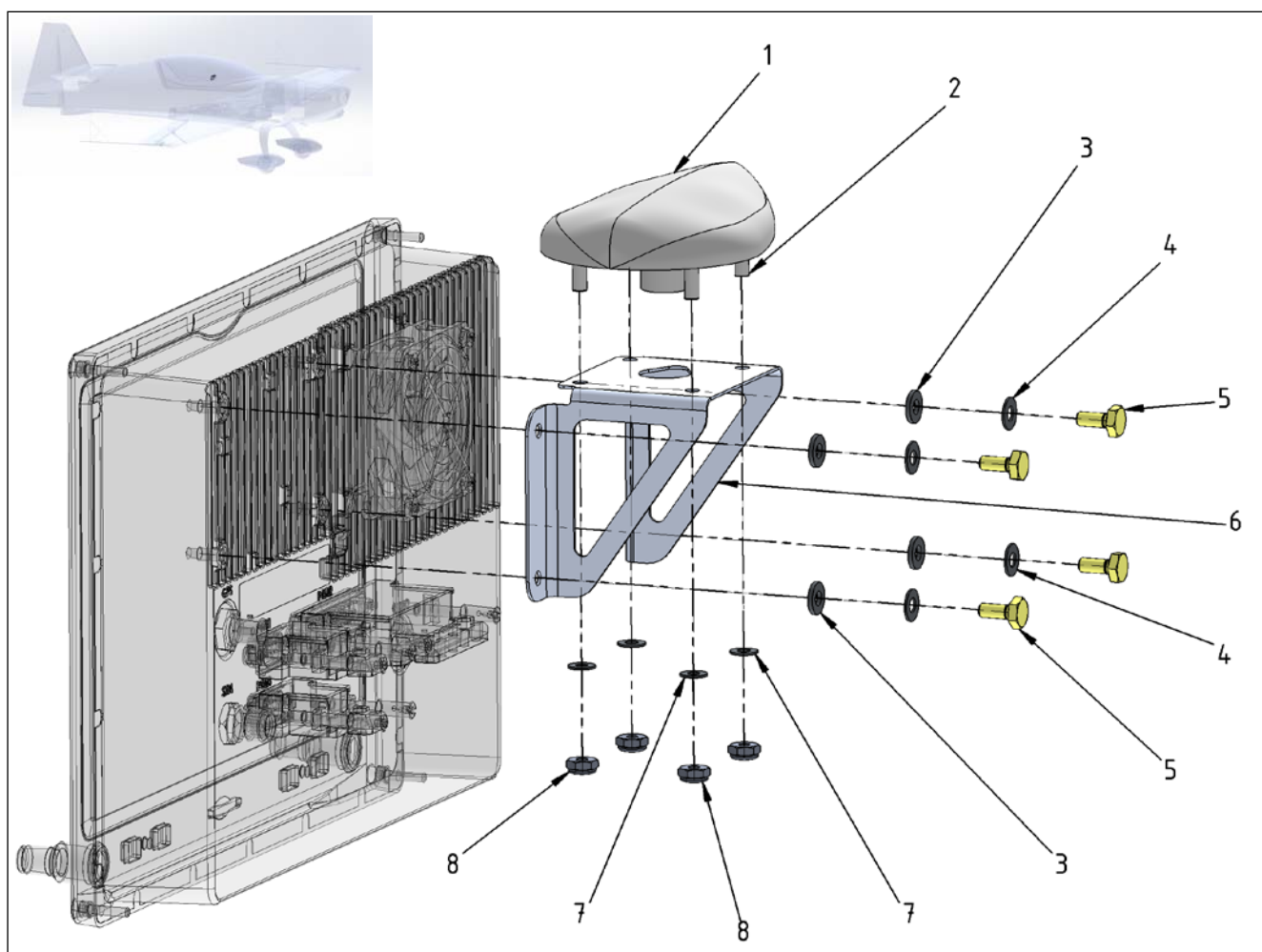
Figure 31-9 Garmin GDU 450 Antenna
