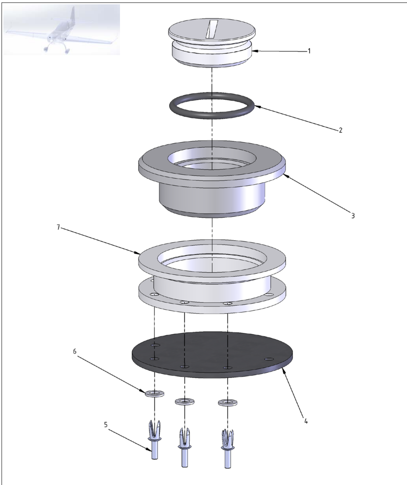
Figure 28-6 Storage – Wing Tank Filler Neck with Sealing Lip
