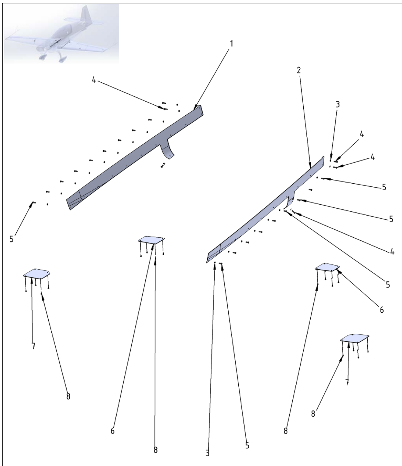
Figure 51-3 Access Panels Wings
