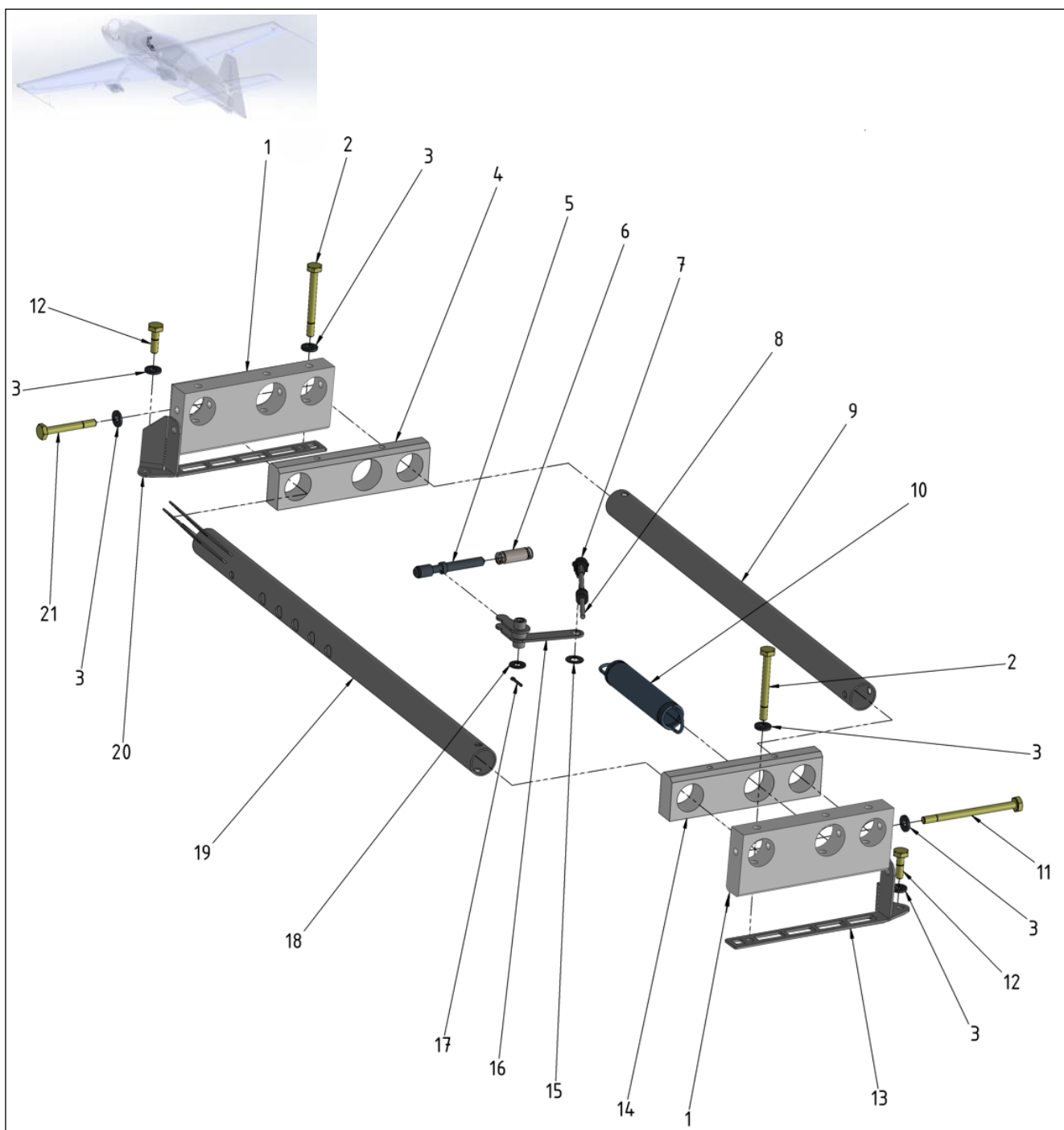
Figure 27-31 Front Pedal RH -Base Raised
