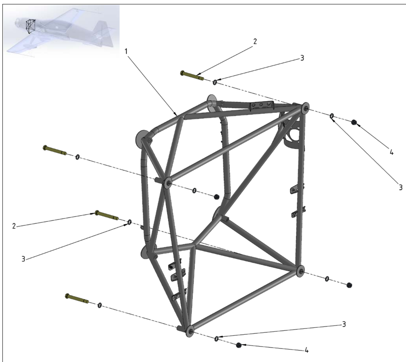
Figure 71-1 Engine Mount
