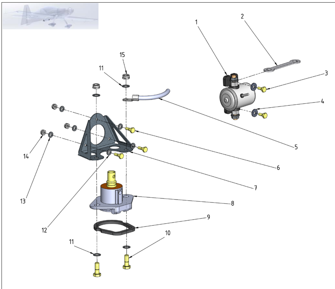
Figure 24-8 External Power
