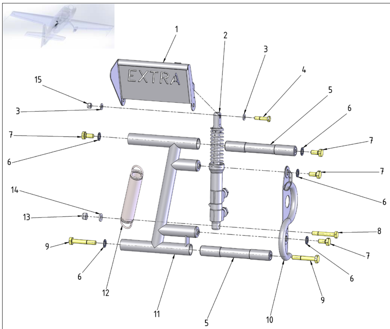
Figure 27-32 Rear Pedal LH - Pedal
