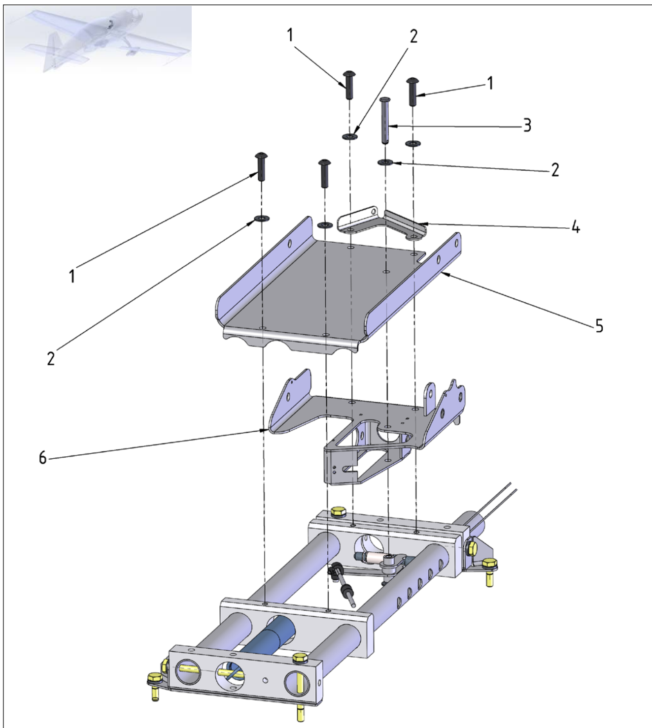
Figure 27-25 Front Pedal LH - Footrest
