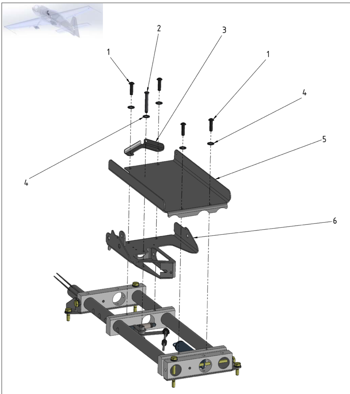
Figure 27-29 Front Pedal RH - Footrest
