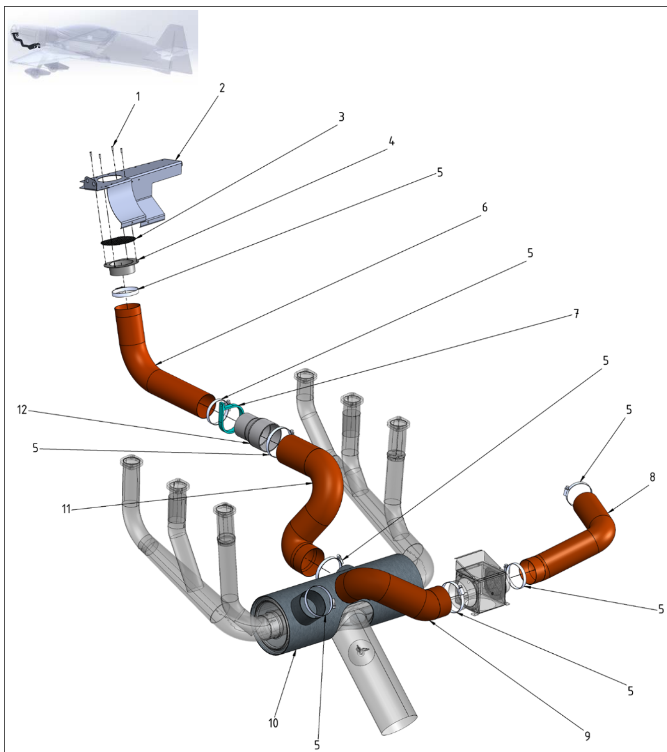
Figure 21-3 Cabin Ventilation System – Air Routing
