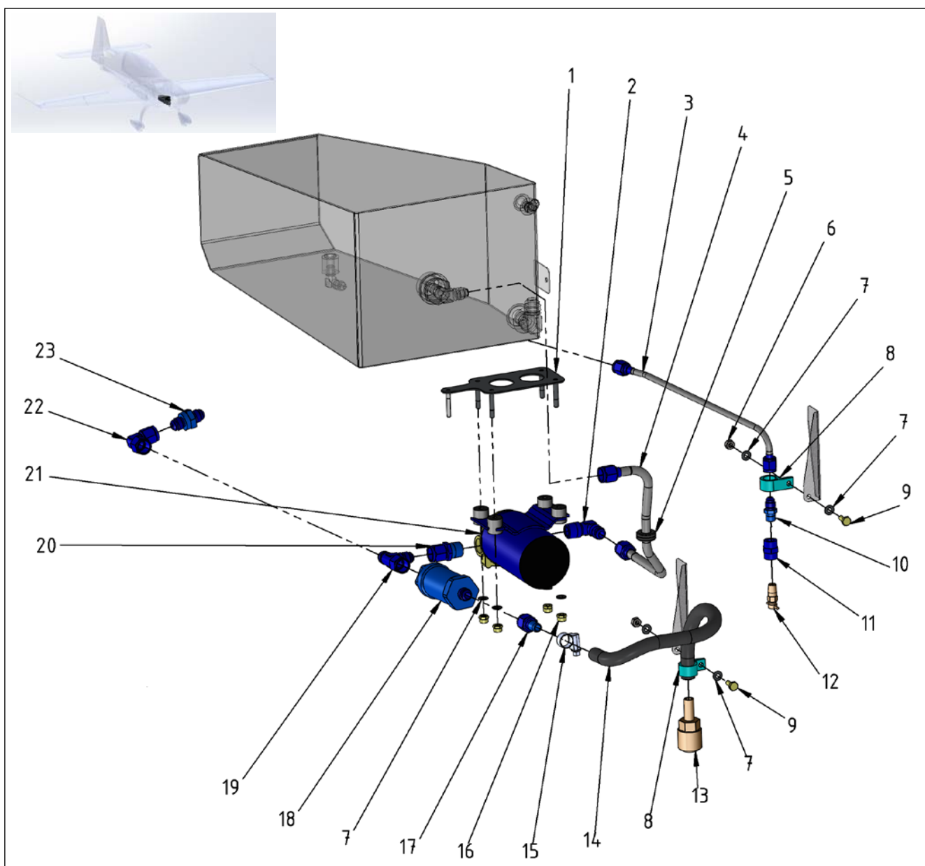
Figure 87-2 Smoke - Distribution
