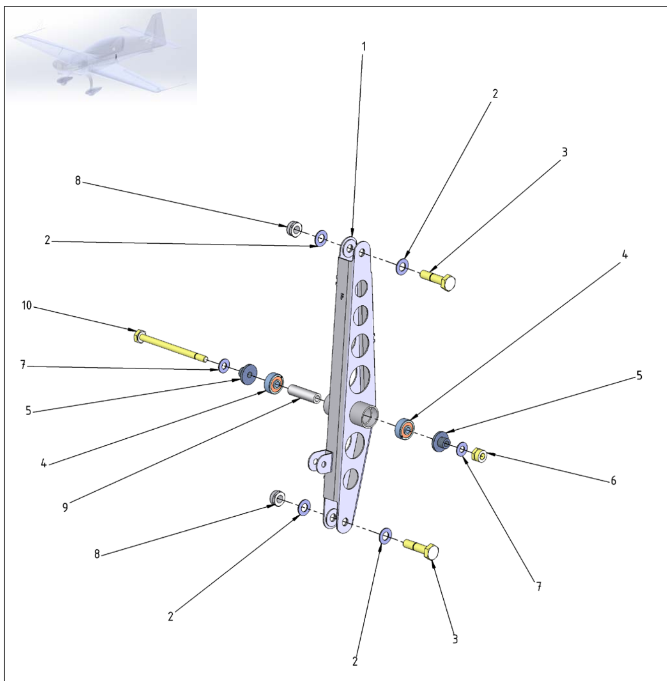
Figure 27-4 Elevator Bell Crank
