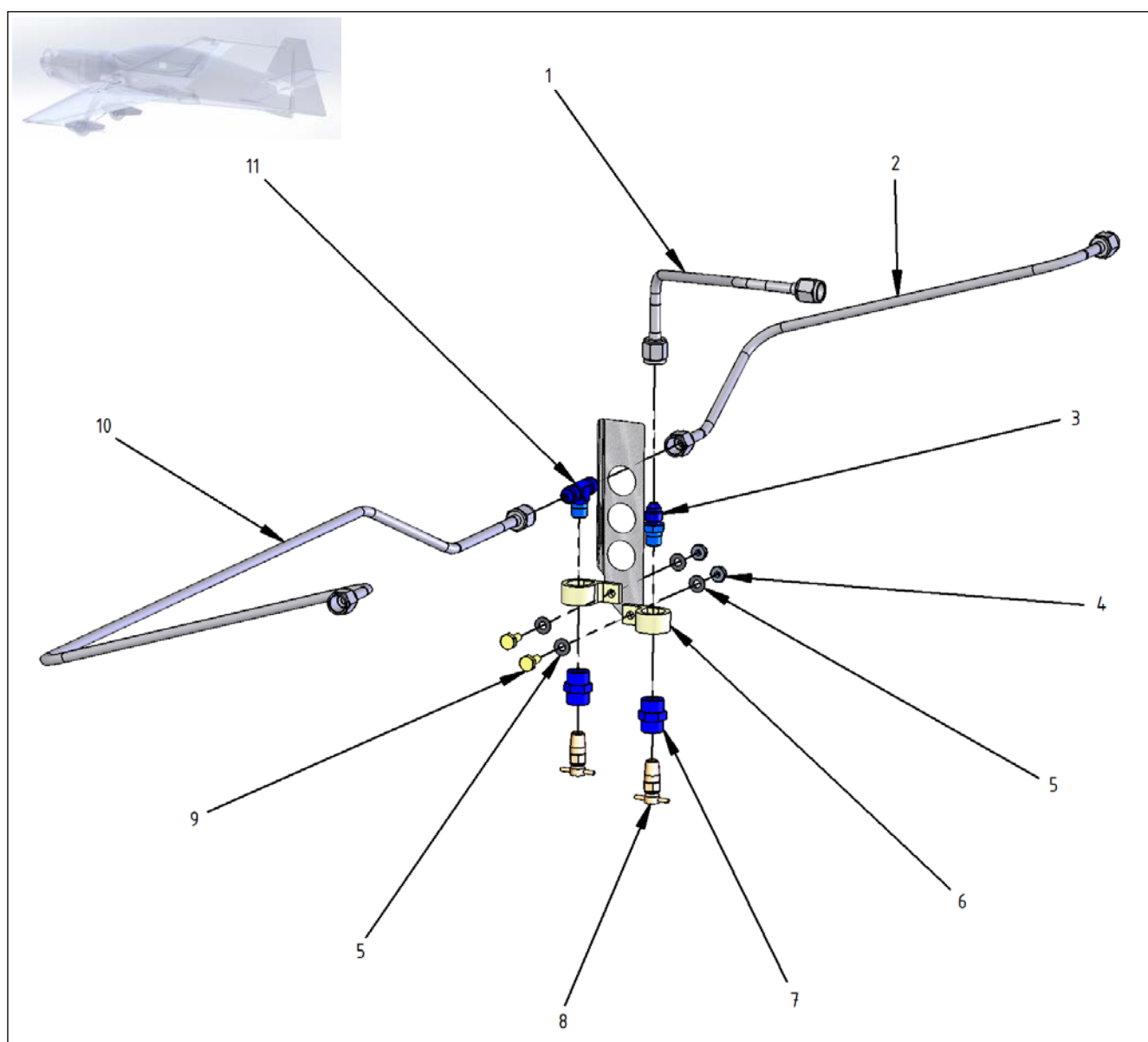
Figure 28-16 Fuel & Drain Lines – Drain Lines
