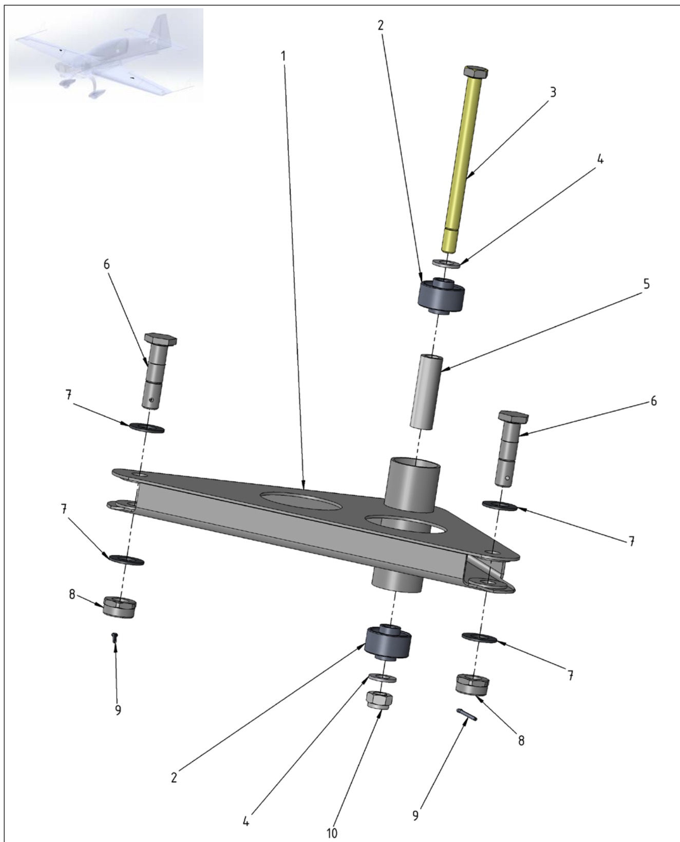
Figure 27-3 Outer Aileron Bell Crank
