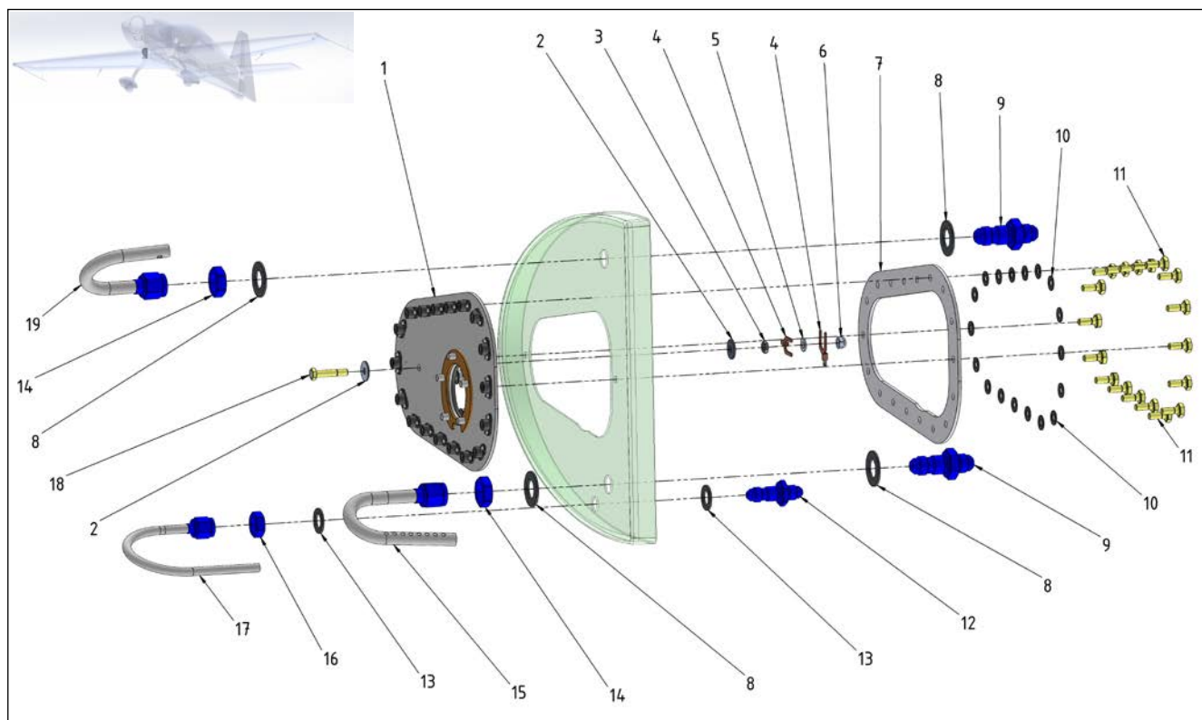
Figure 28-3 Storage - Wing Tank Inspection Door with Outlets - LH
