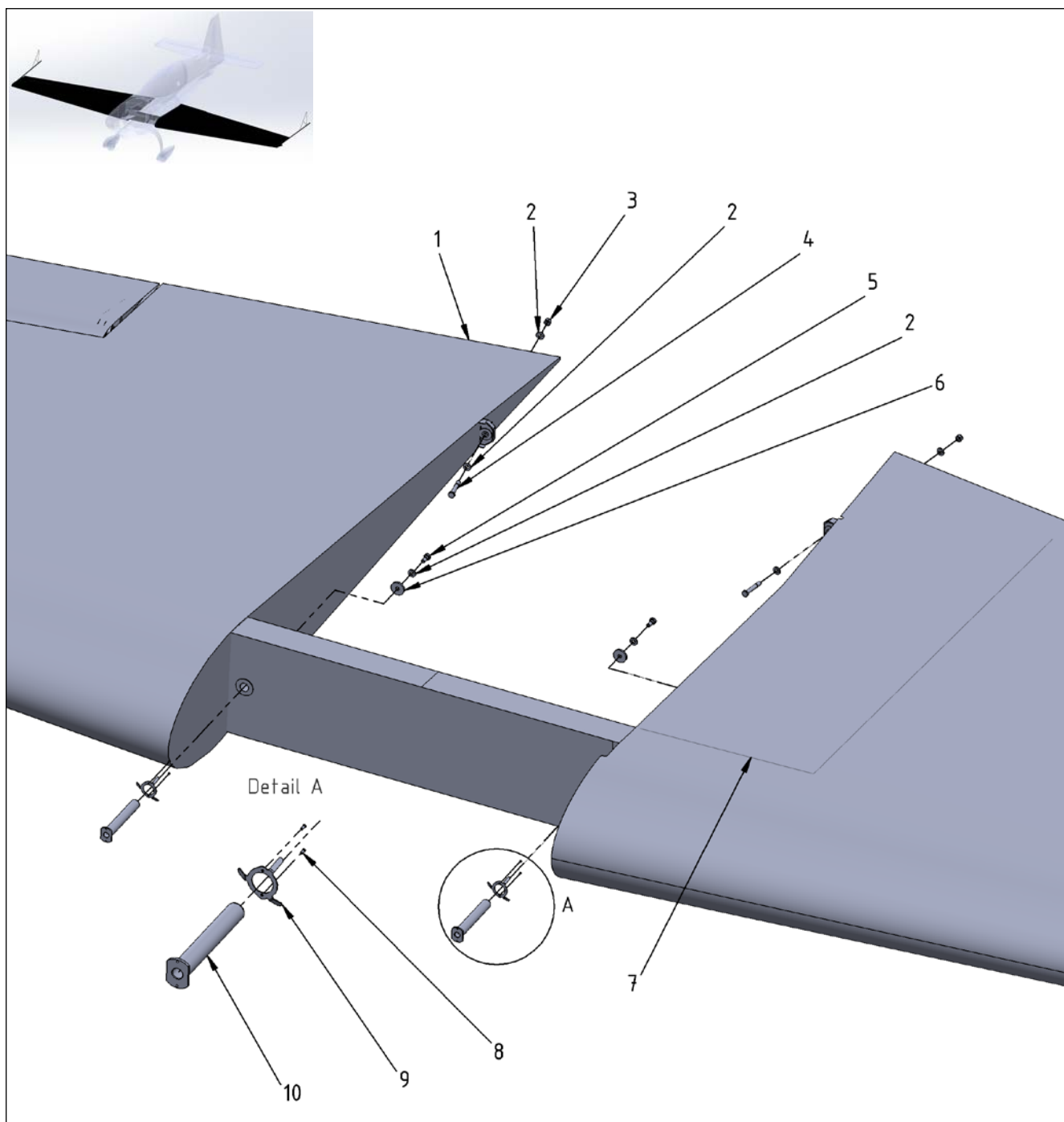
Figure 57-1 Wing & Main Wing Bolt
