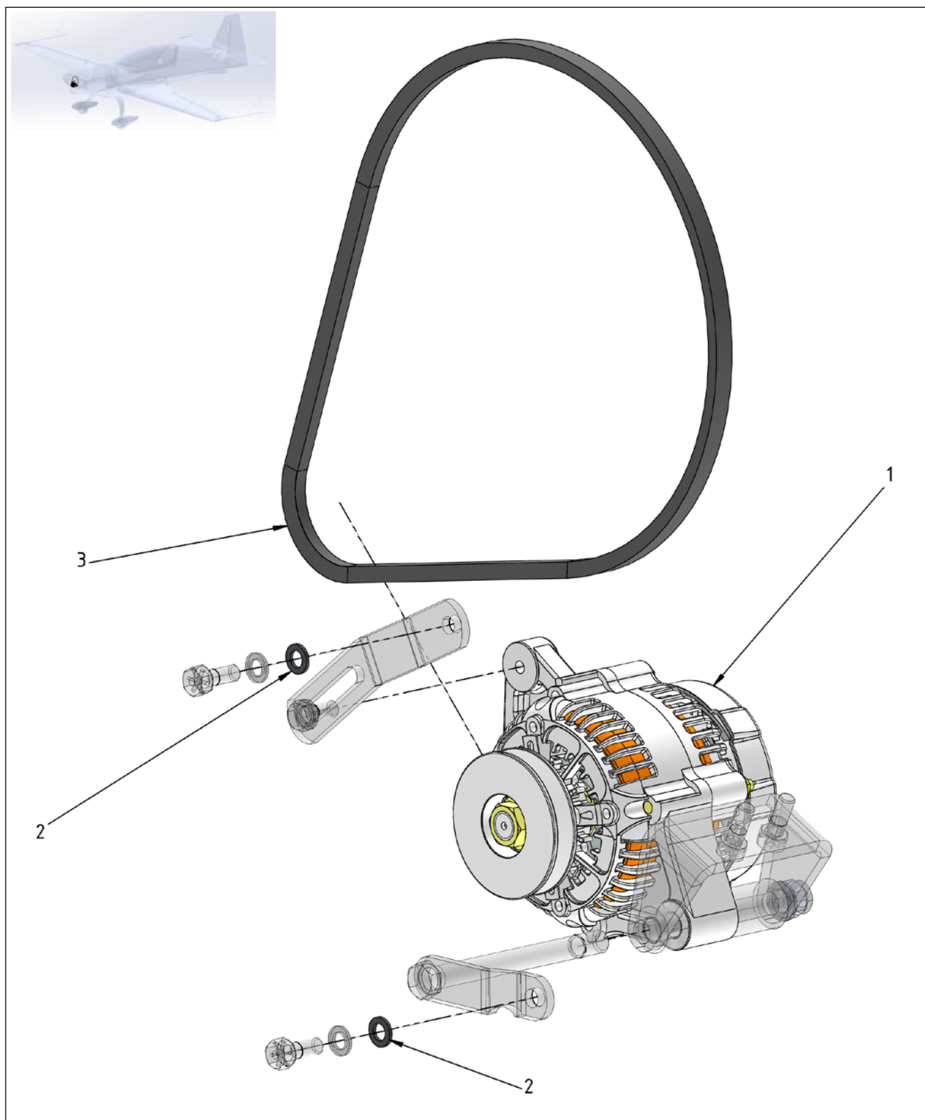
Figure 24-4 Alternator System 60A
