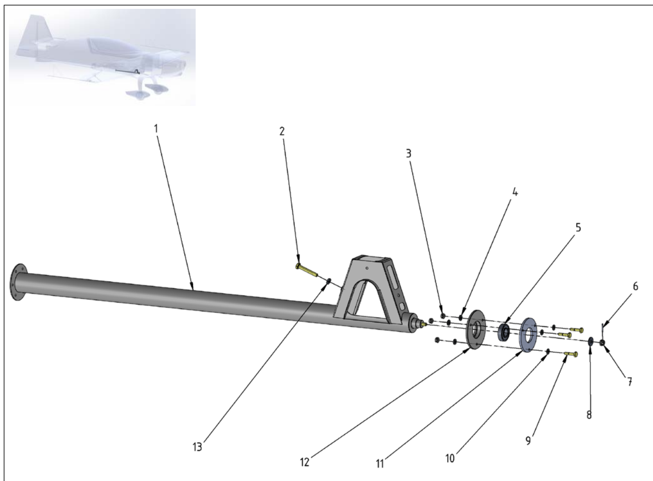
Figure 27-10 Torque Tube – Front Part
