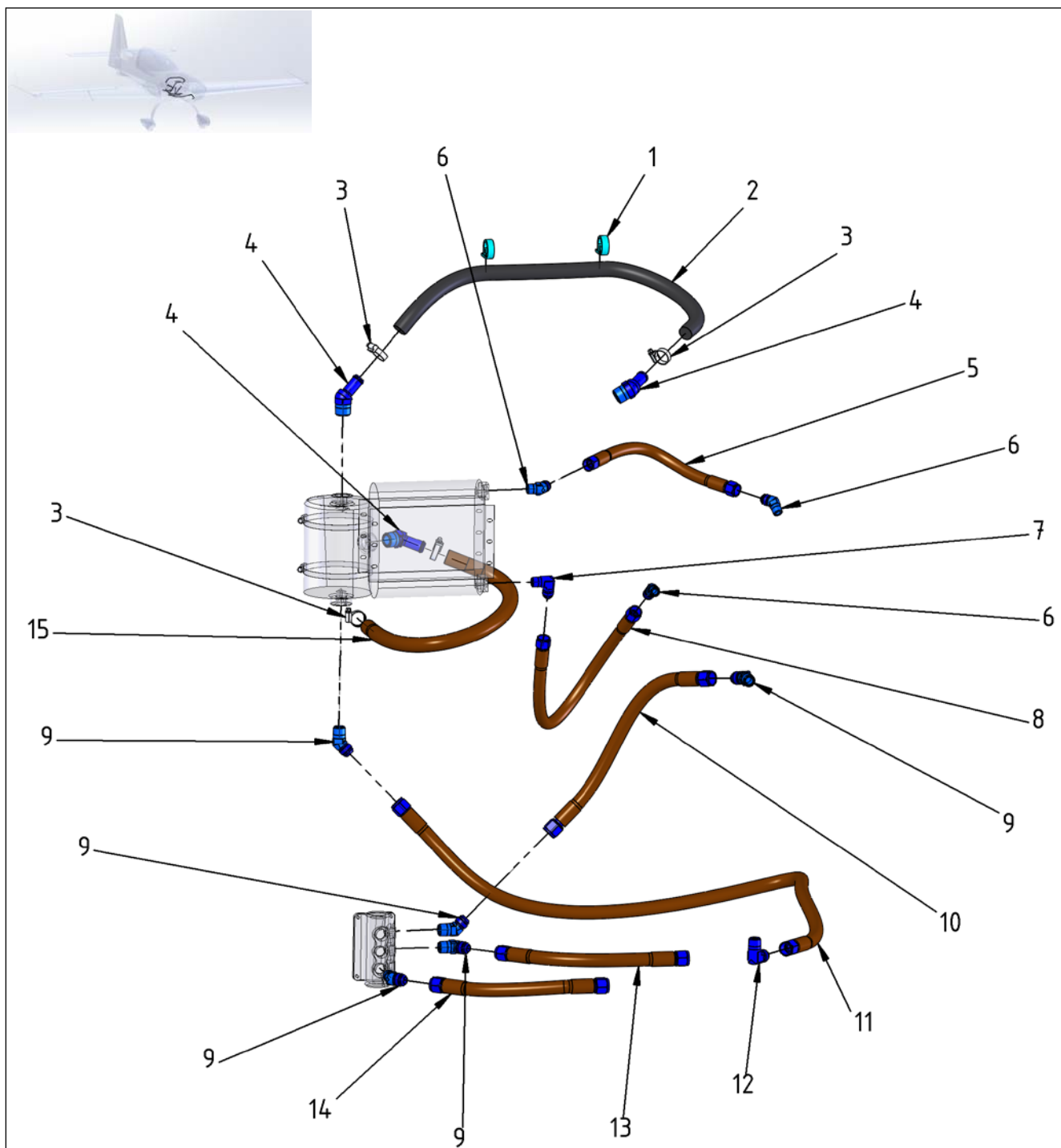
Figure 79-5 Fittings and Hoses (Oil)
