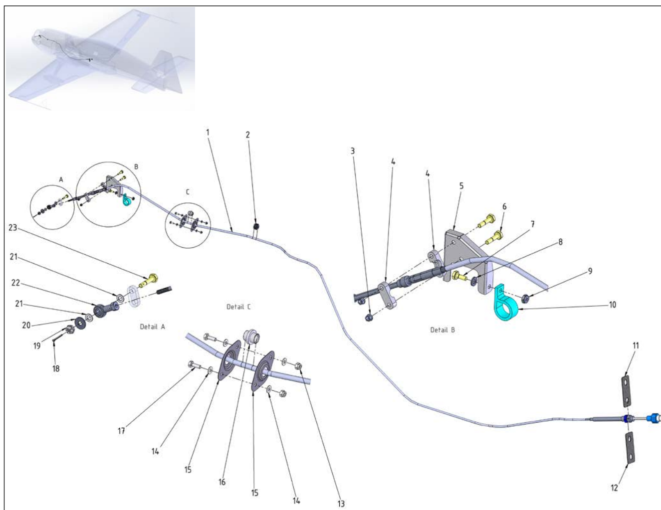
Figure 61-3 Propeller - Controlling
