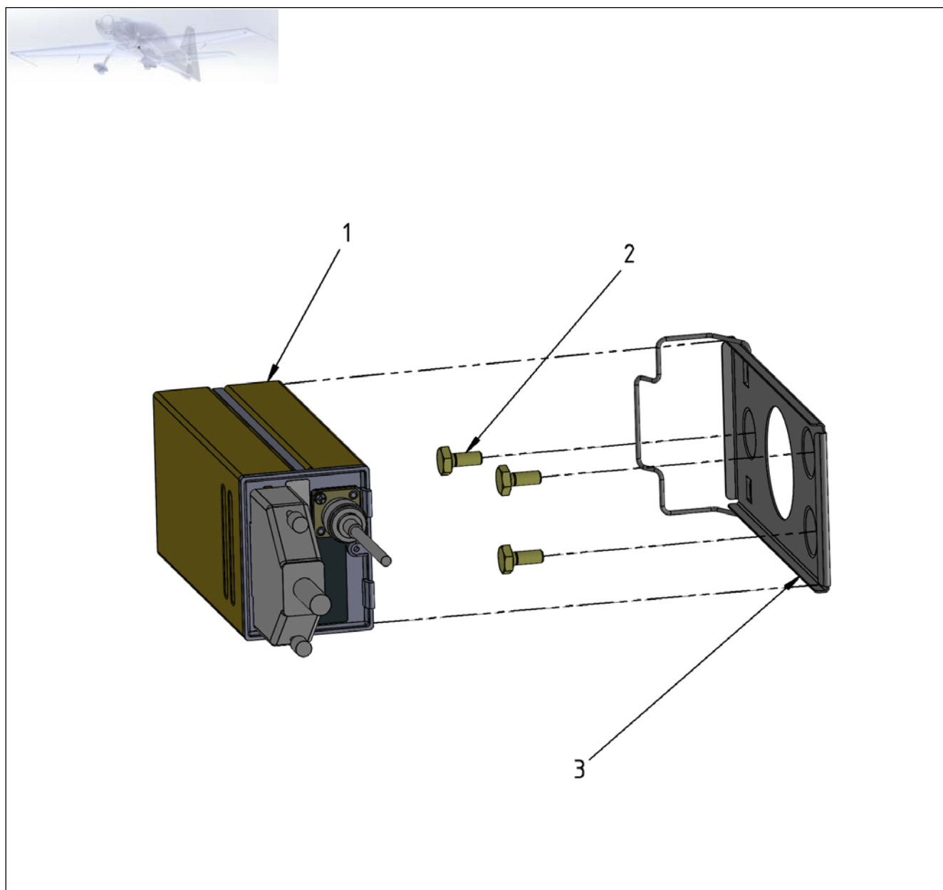
Figure 23-3 VHF Radio
