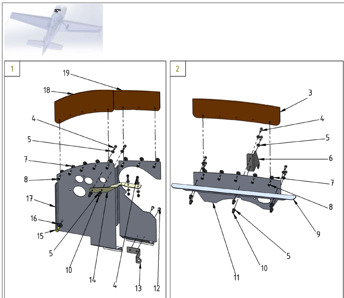
Figure 71-7 Air Baffles – Air Baffles AFT LH & MID
