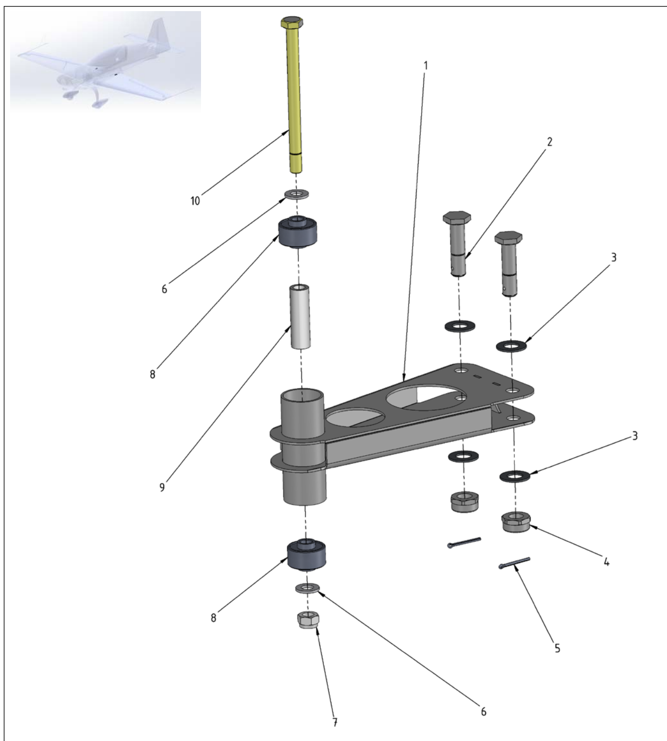
Figure 27-2 Inner Aileron Bell Crank
