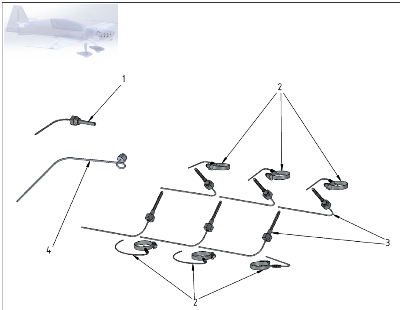
Figure 77-2 Engine Sensors
