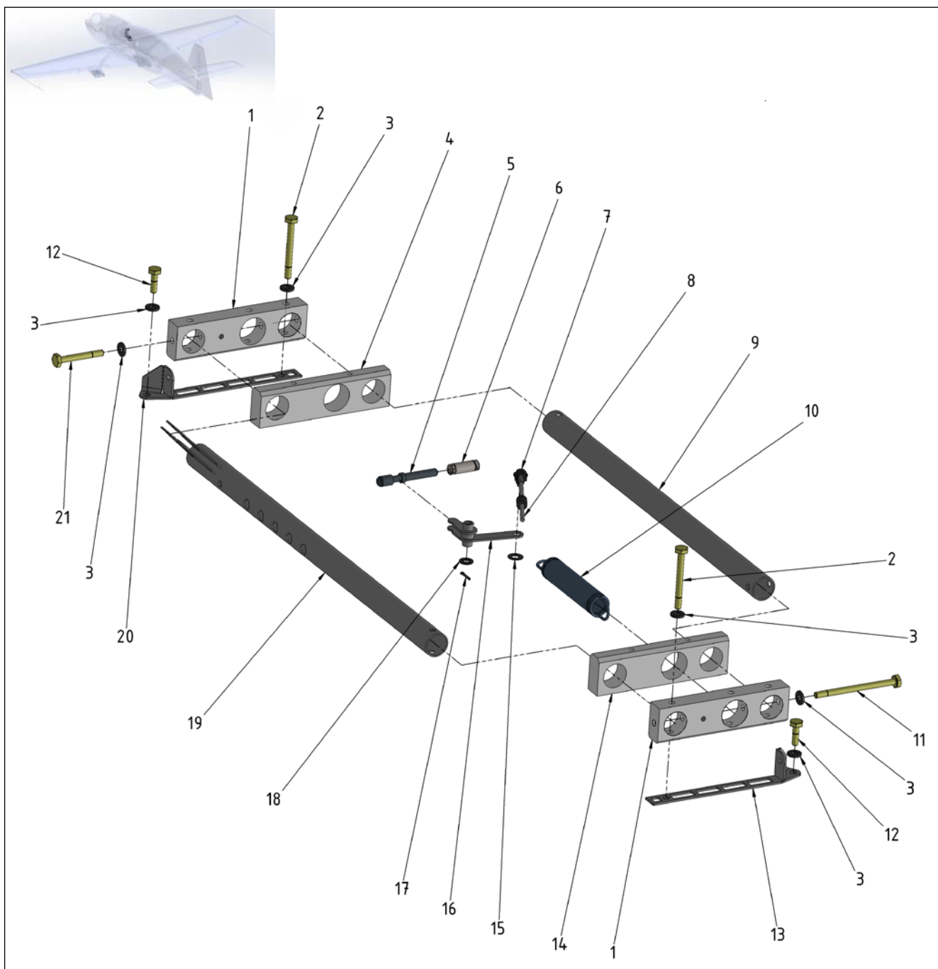
Figure 27-30 Front Pedal RH - Base
