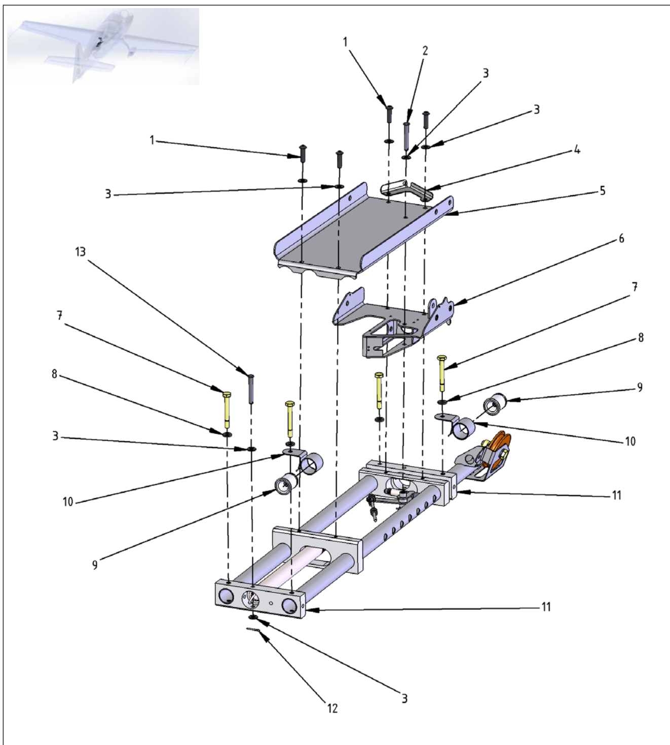
Figure 27-33 Rear Pedal LH - Footrest
