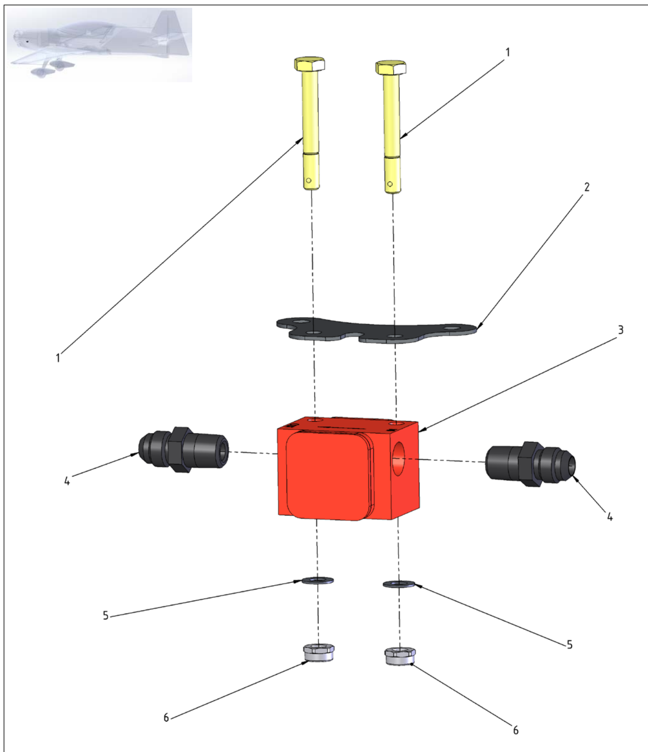
Figure 77-4 Fuel Flow Transducer
