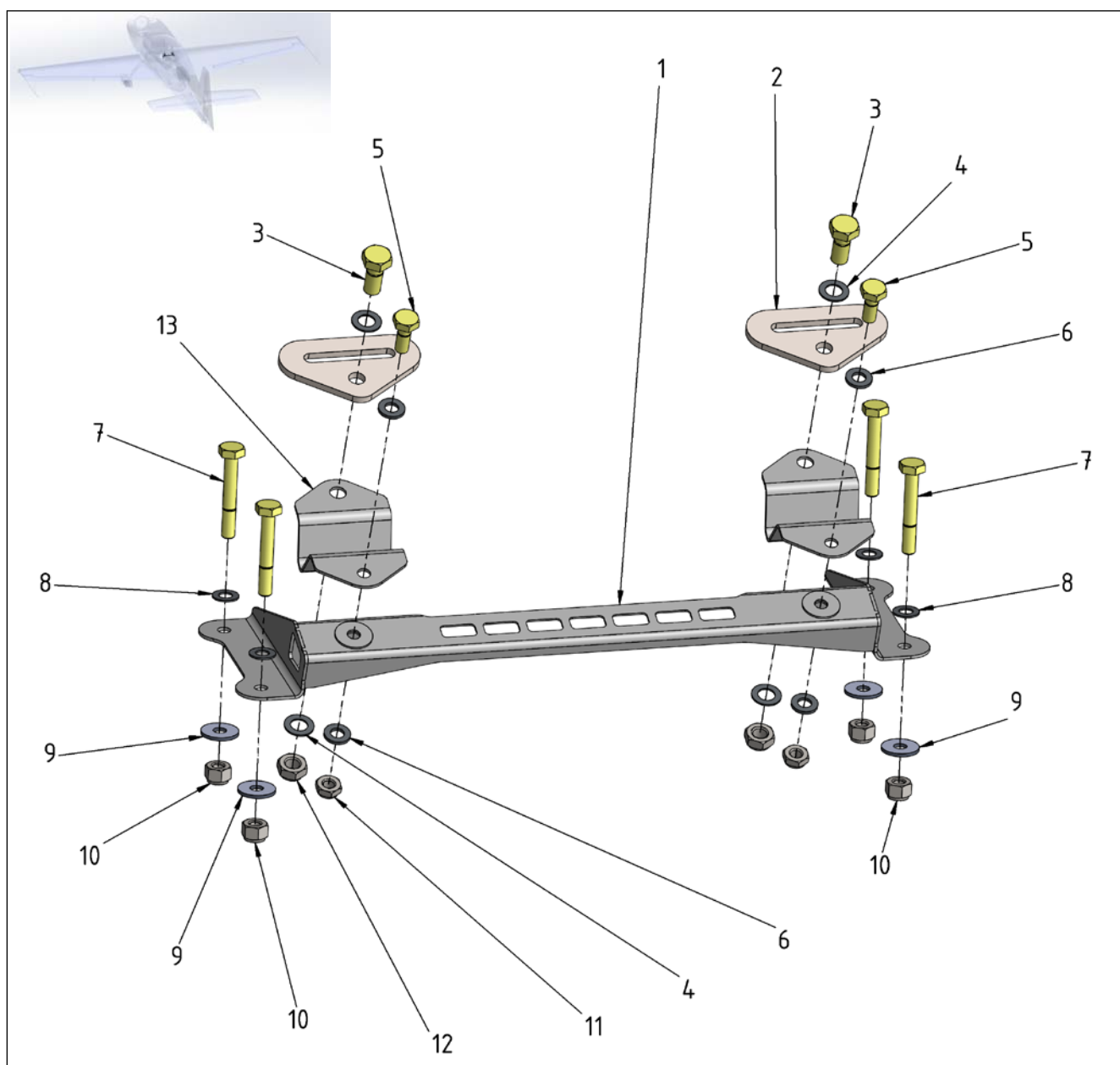
Figure 25-13 Copilot Shoulder Harness
