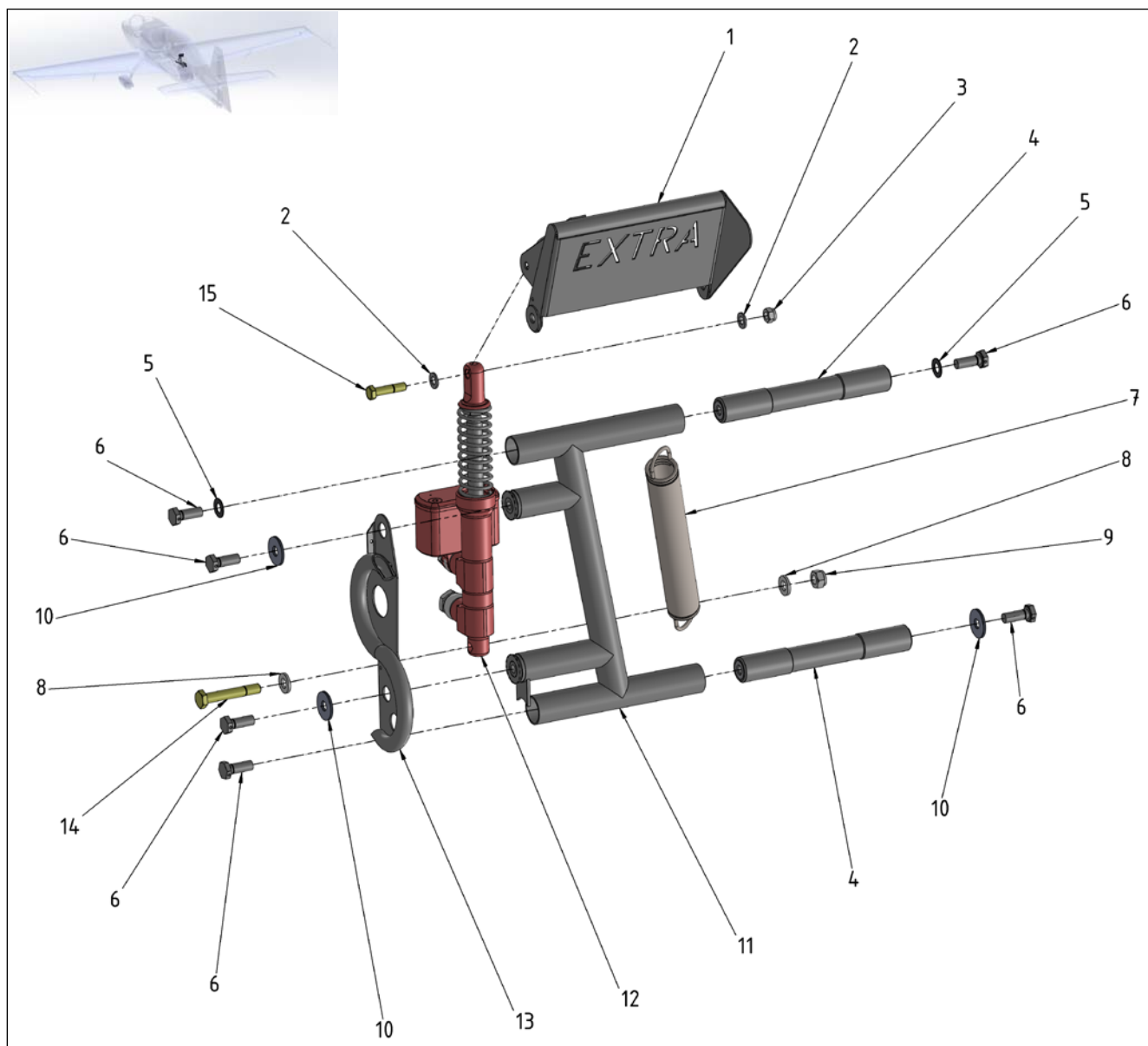
Figure 27-35 Rear Pedal RH - Pedal
