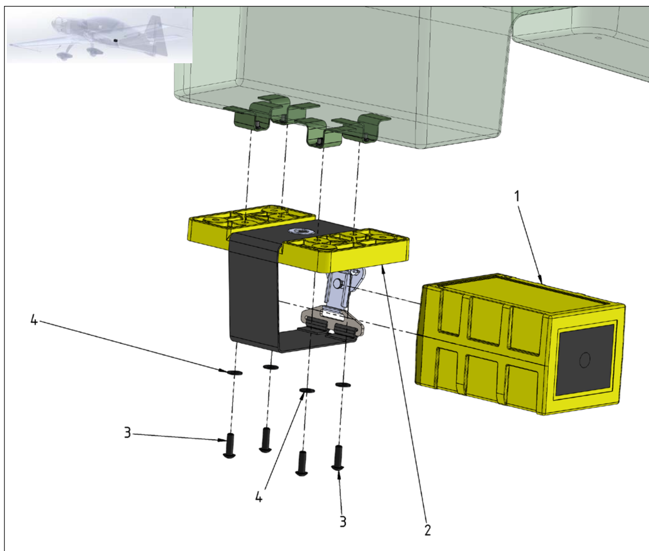
Figure 23-1 Emergency Locator Transmitter
