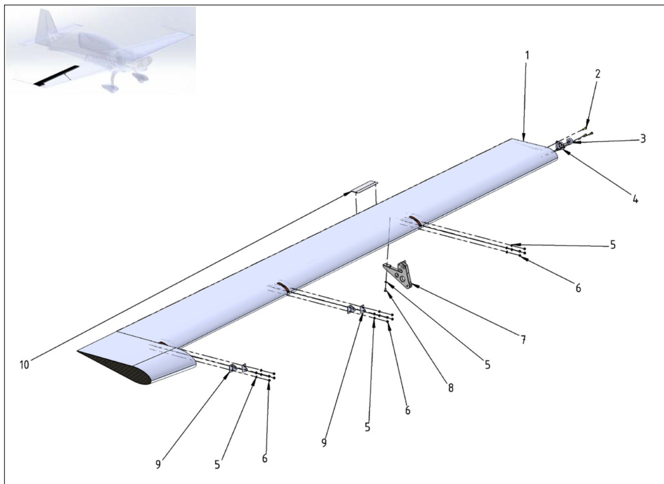
Figure 27-15 Ailerons – Aileron (improved) RH
