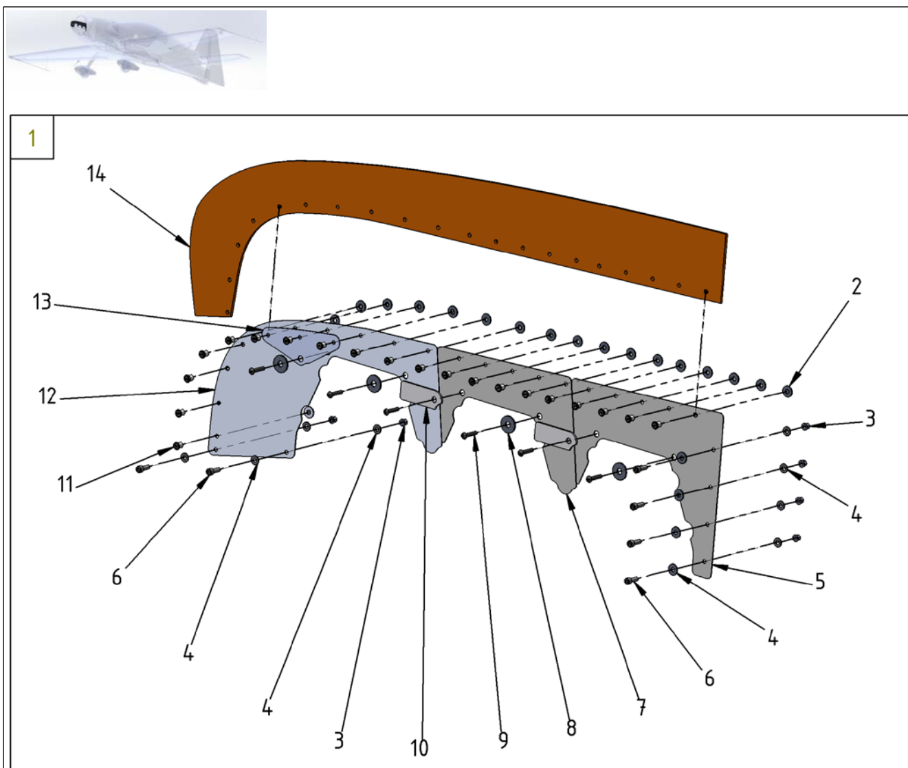
Figure 71-5 Air Baffles – Air Baffles LH
