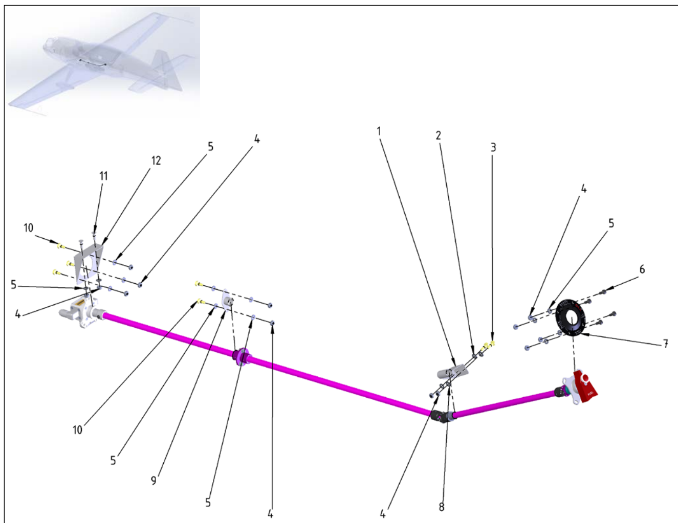
Figure 28-11 Distribution – Fuel Selector Valve Brackets
