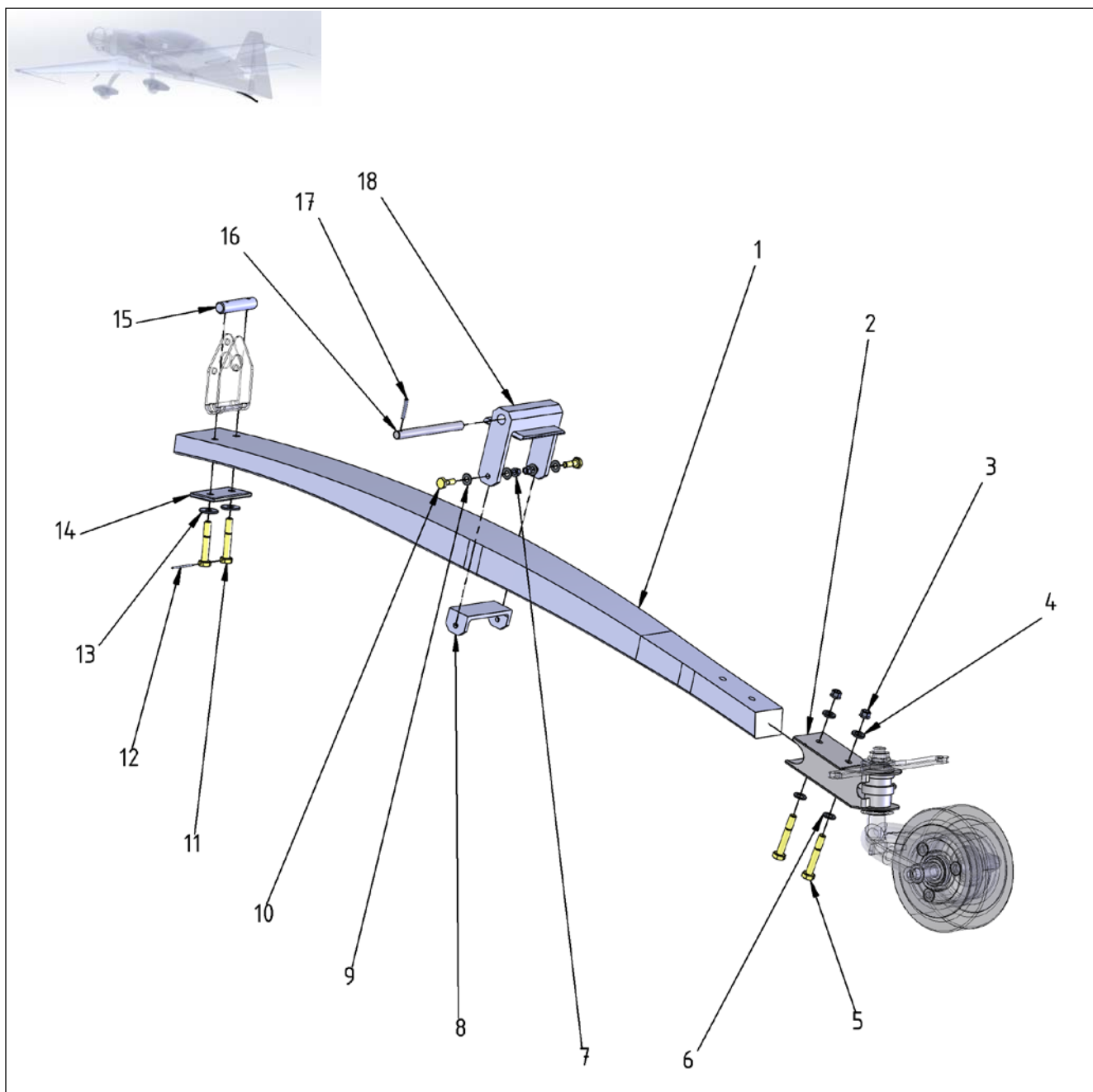
Figure 32-5 Main Gear – Tail Spring
