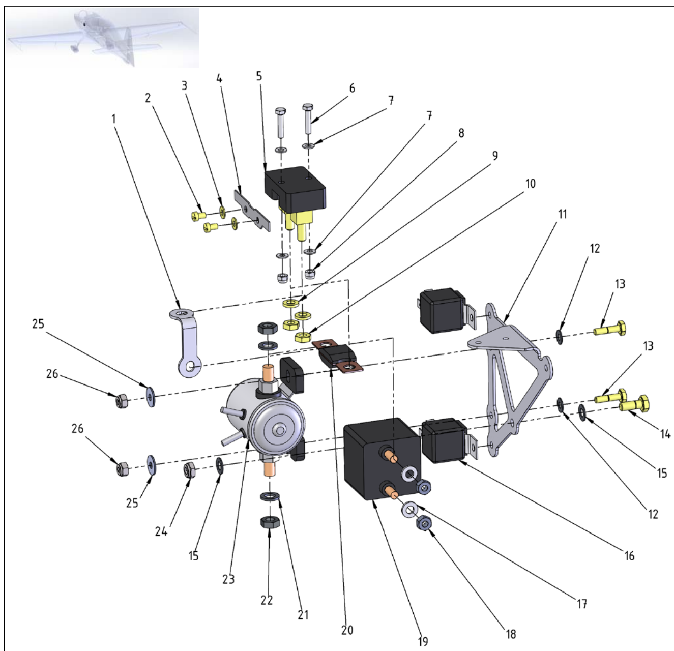
Figure 24-7 Relay Rack Assembly
