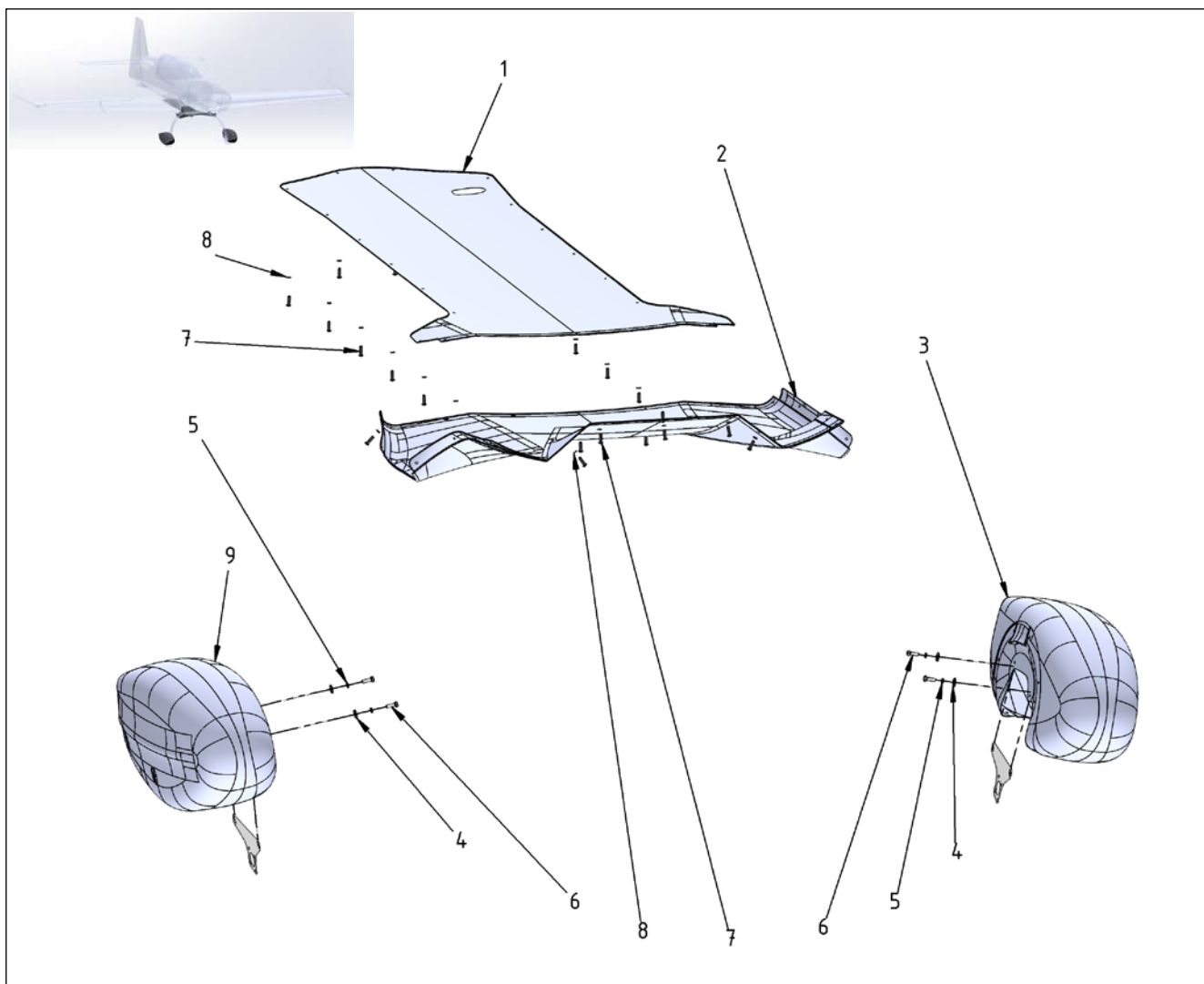
Figure 51-1 Access Panels Fuselage
