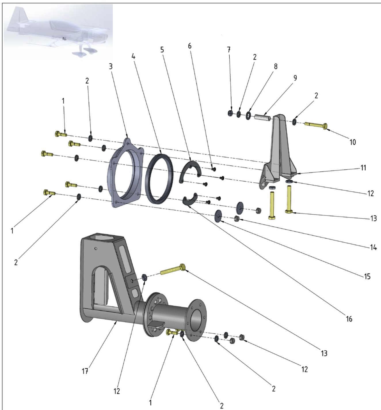
Figure 27-11 Torque Tube – Rear Part
