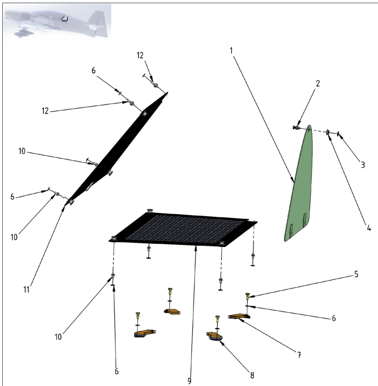
Figure 25-17 Baggage Compartment
