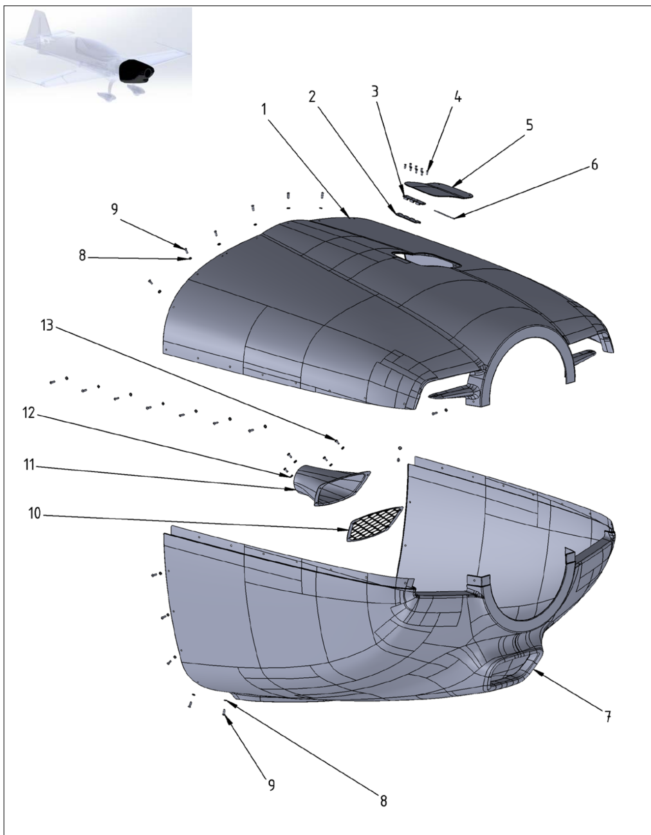
Figure 51-4 Access Panels Engine Compartment
