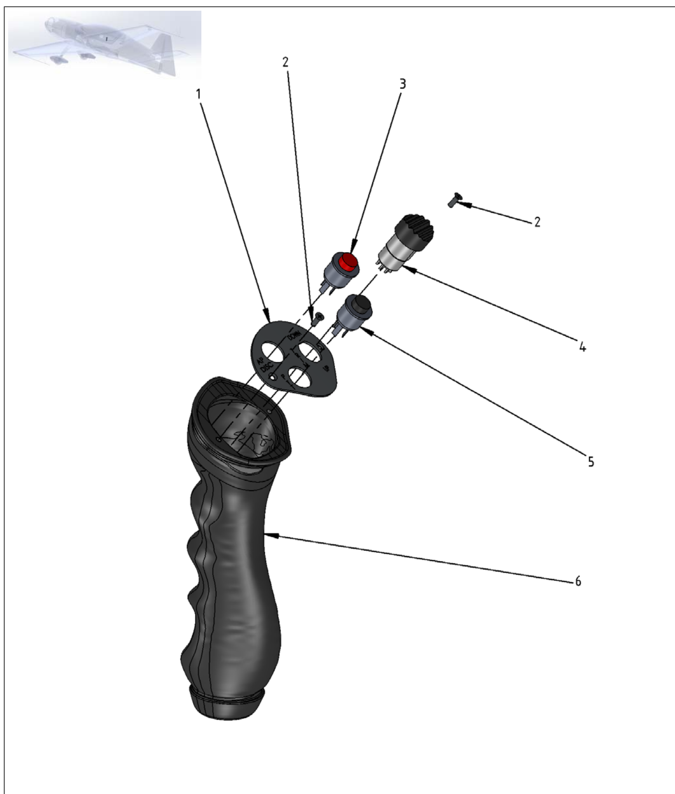
Figure 27-8 Control Stick Covers - Pilot Option Autopilot
