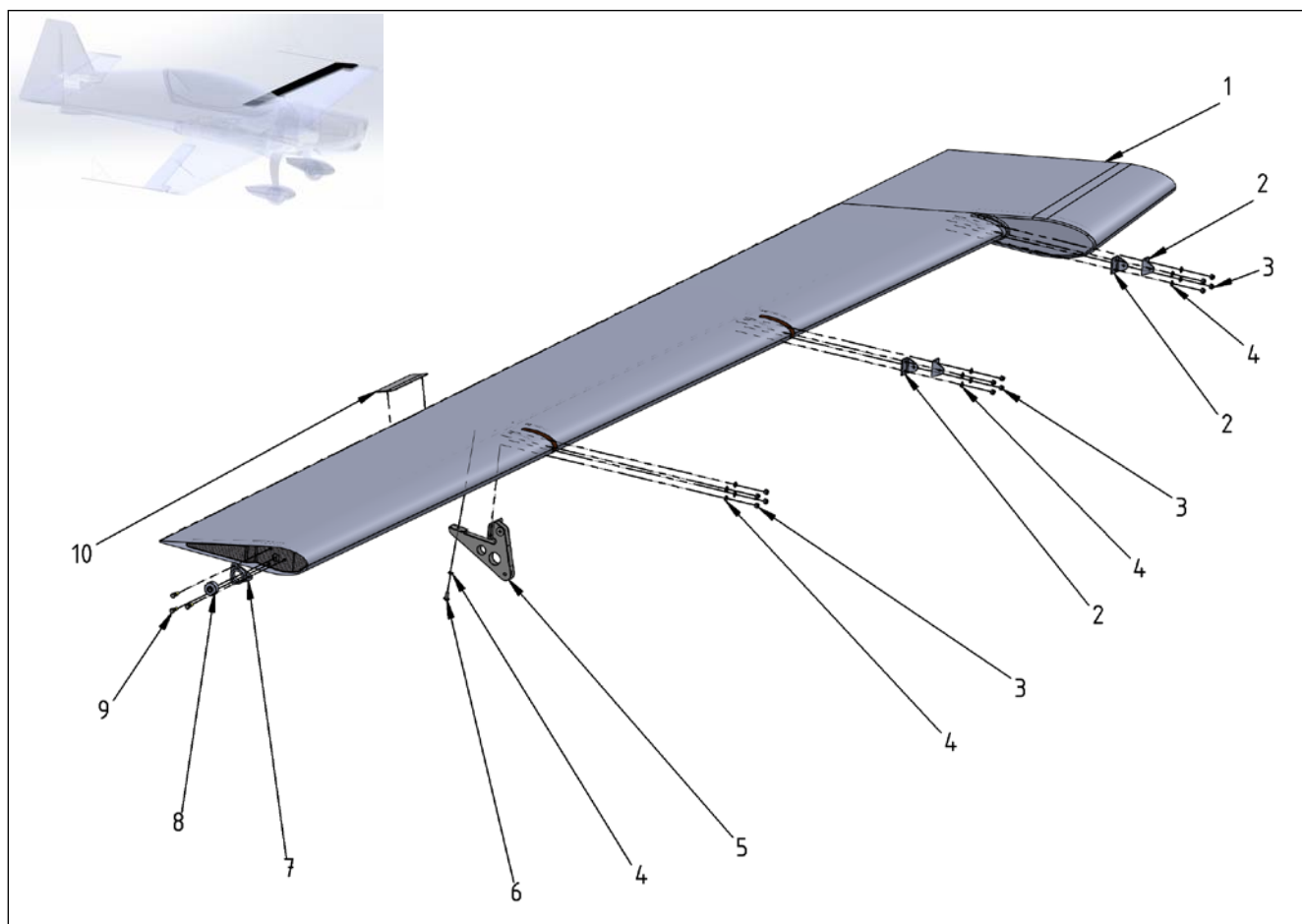
Figure 27-14 Ailerons – Aileron (improved) LH
