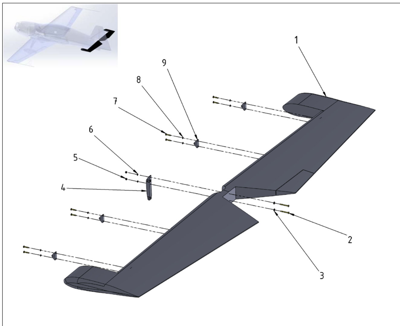
Figure 27-38 Elevator & Tab - Elevator
