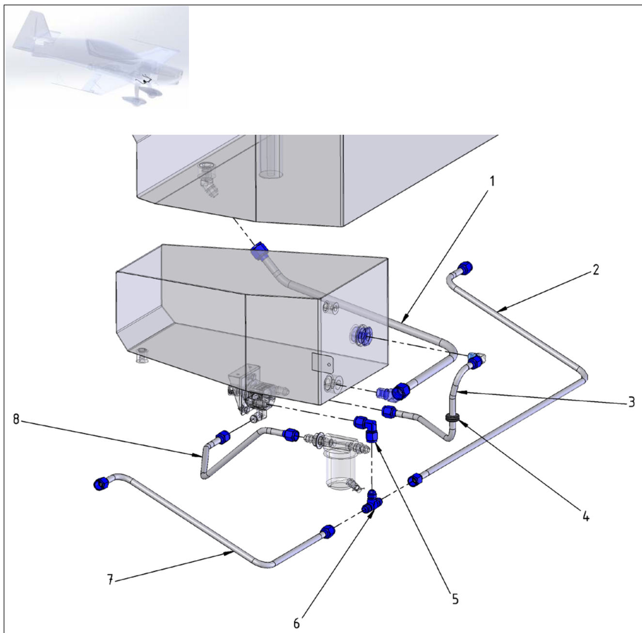
Figure 28-14 Fuel & Drain Lines - Fuselage
