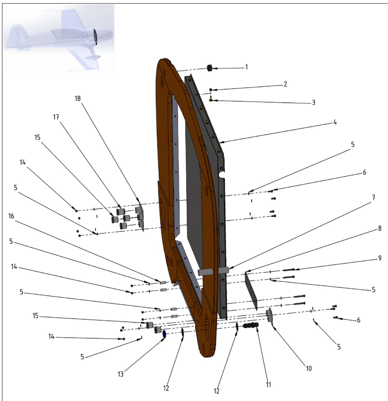
Figure 53-1 Firewall
