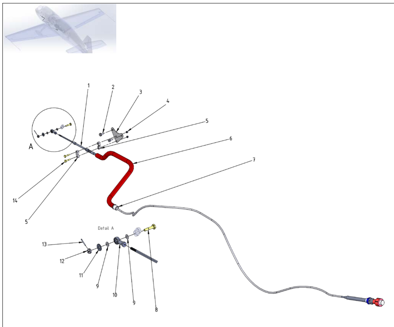
Figure 73-4 Mixture Control
