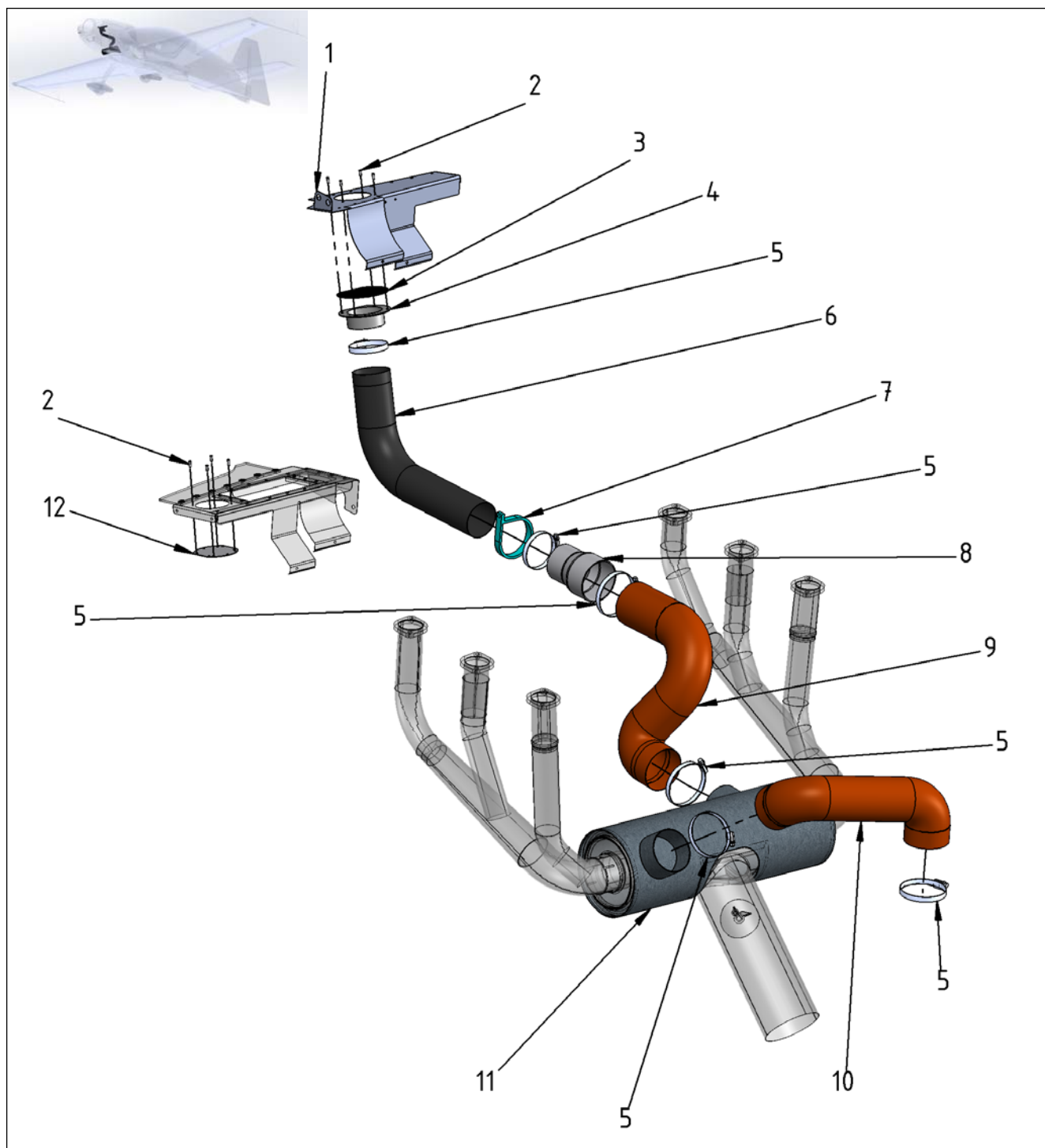
Figure 21-6 With Additional Oil Cooler
