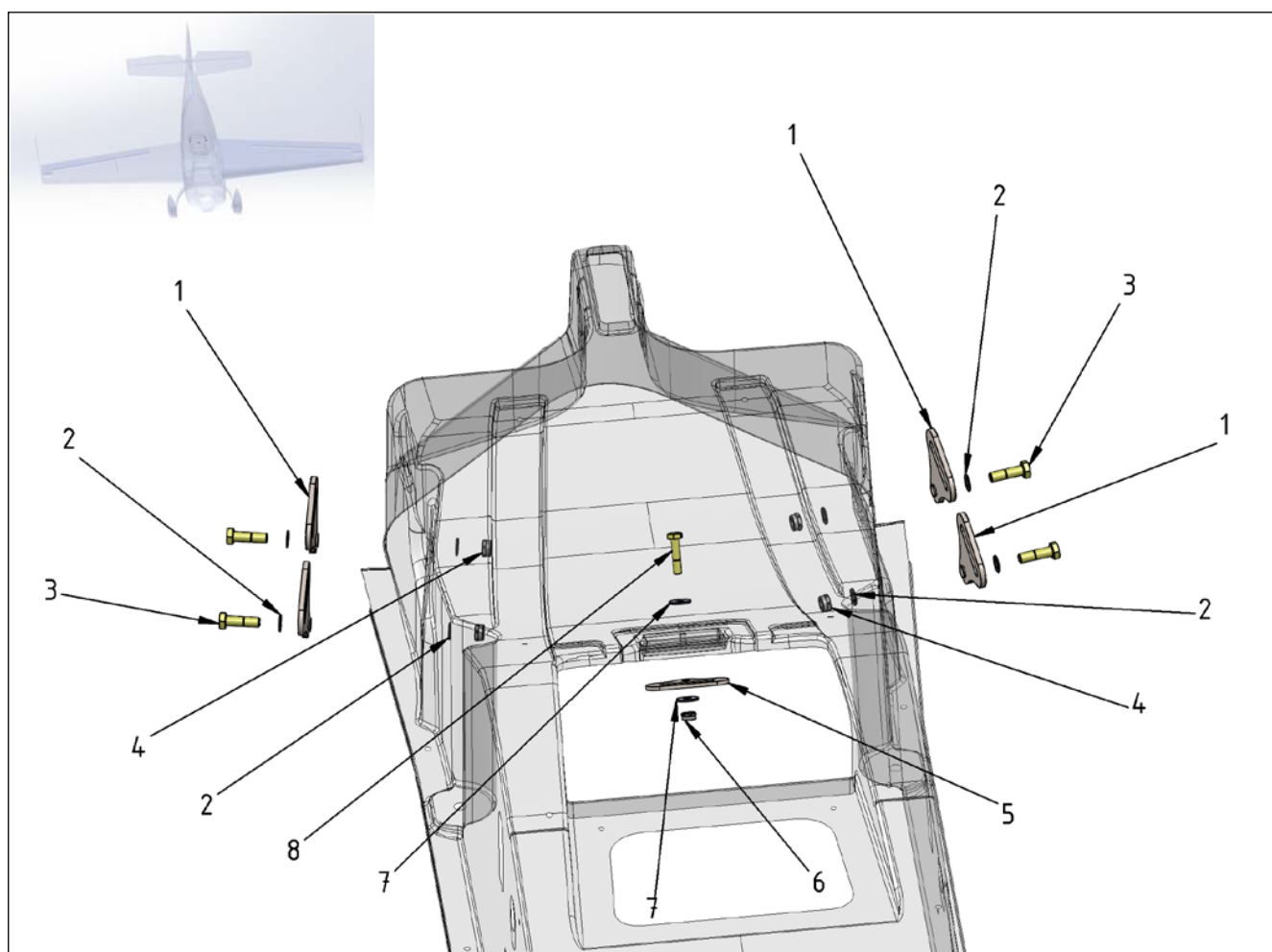
Figure 25-16 Pilot Seat and Crotch Attachments
