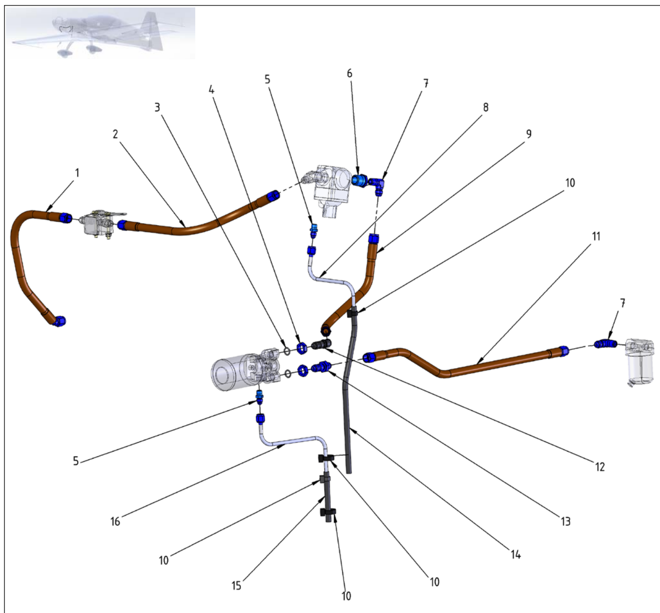
Figure 28-15 Fuel & Drain Lines – Engine Compartment
