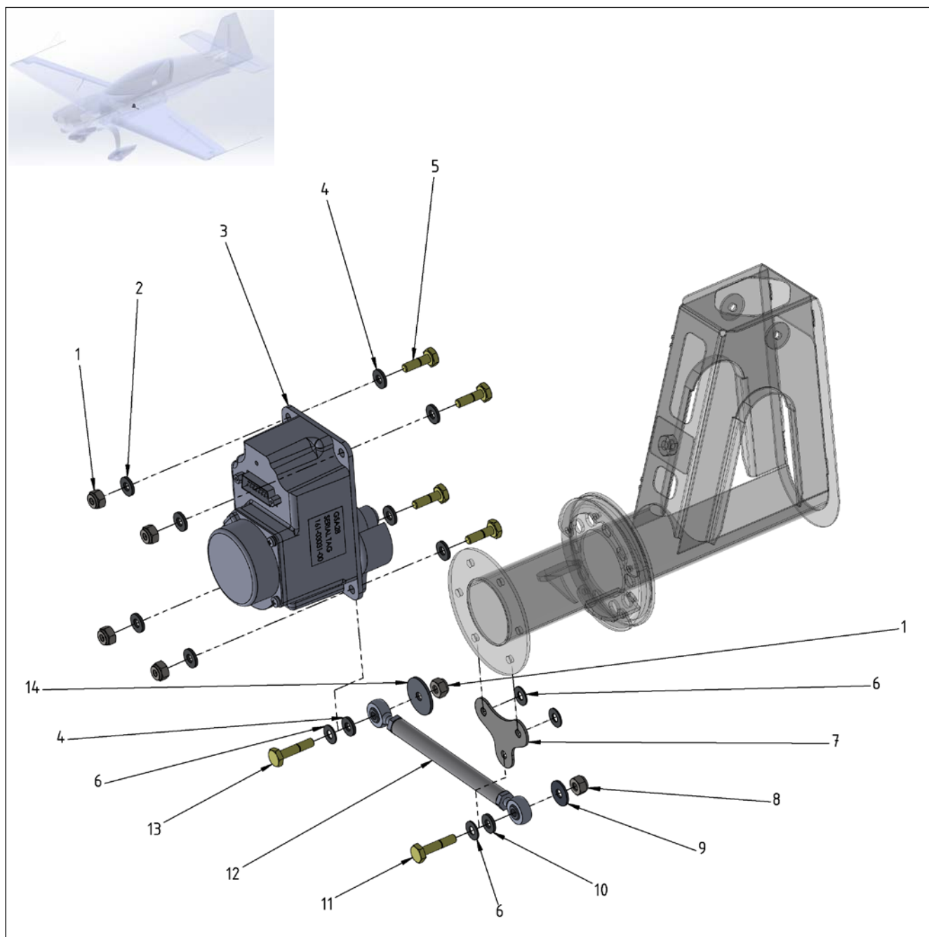
Figure 22-1 Roll Servo
