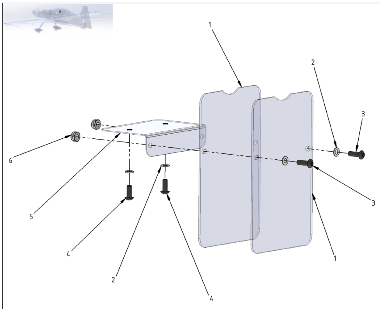
Figure 31-4 Aresti-Cardholder
