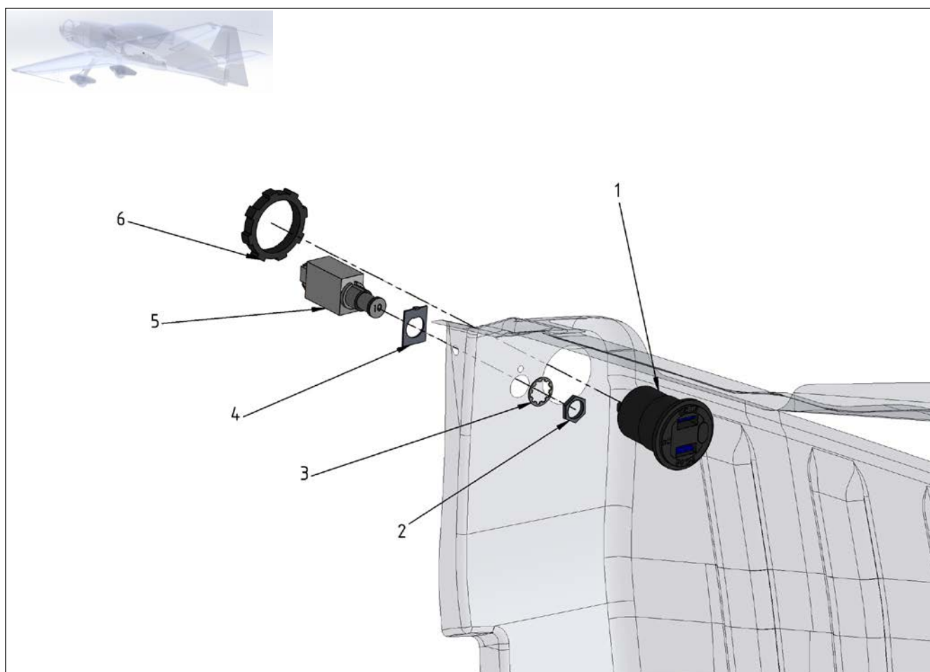
Figure 25-10 Power Sockets – Pilot USB
