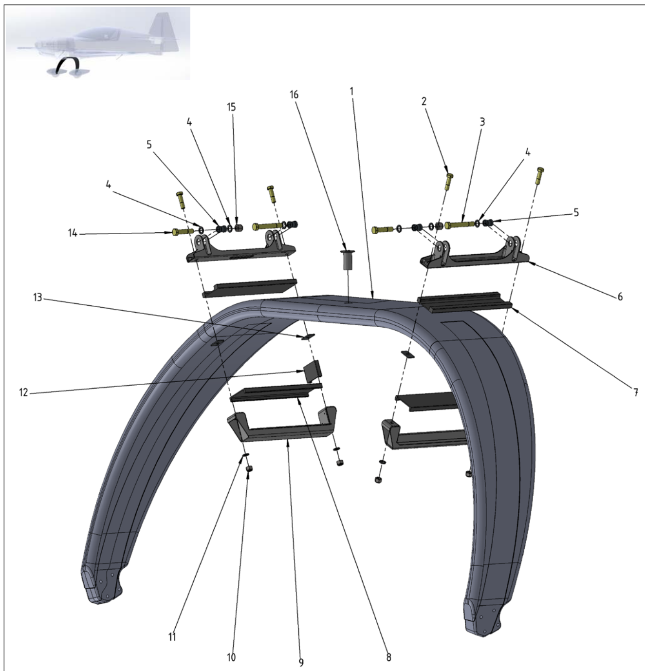
Figure 32-1 Main Gear - Main Landing Gear
