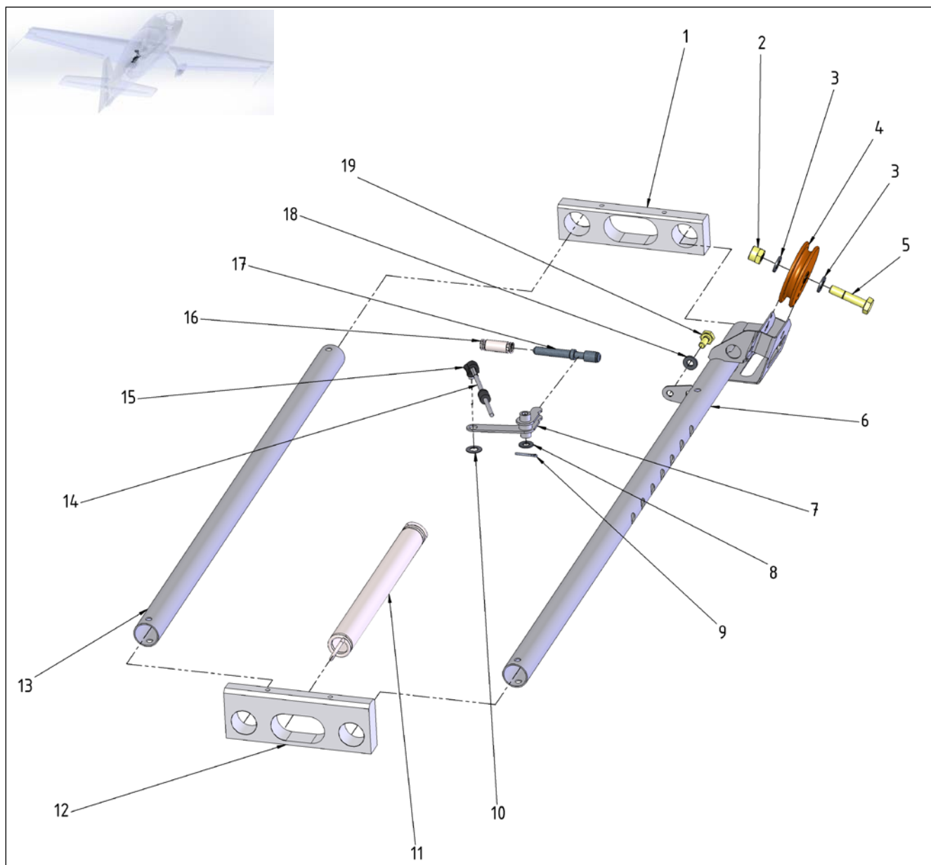
Figure 27-34 Rear Pedal LH - Base
