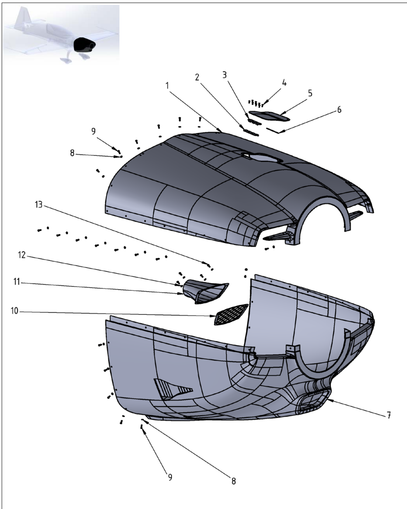
Figure 51-5 Access Panels Engine Compartment (NACA)
