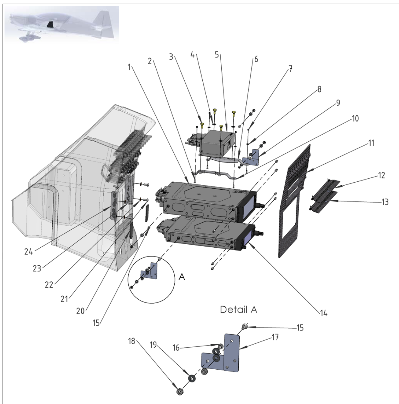
Figure 31-7, Sheet 2 Center Console Options – GNX 375 + GTR 205 + GAD 29 (≥089)
