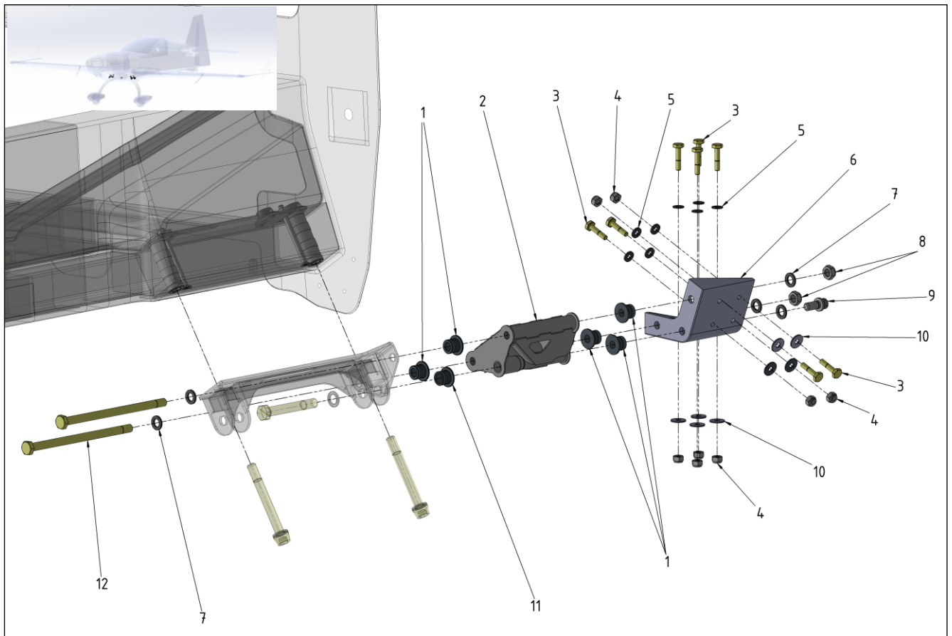
Figure 32-3 Bracket Bridge Fuselage (LH/RH)
