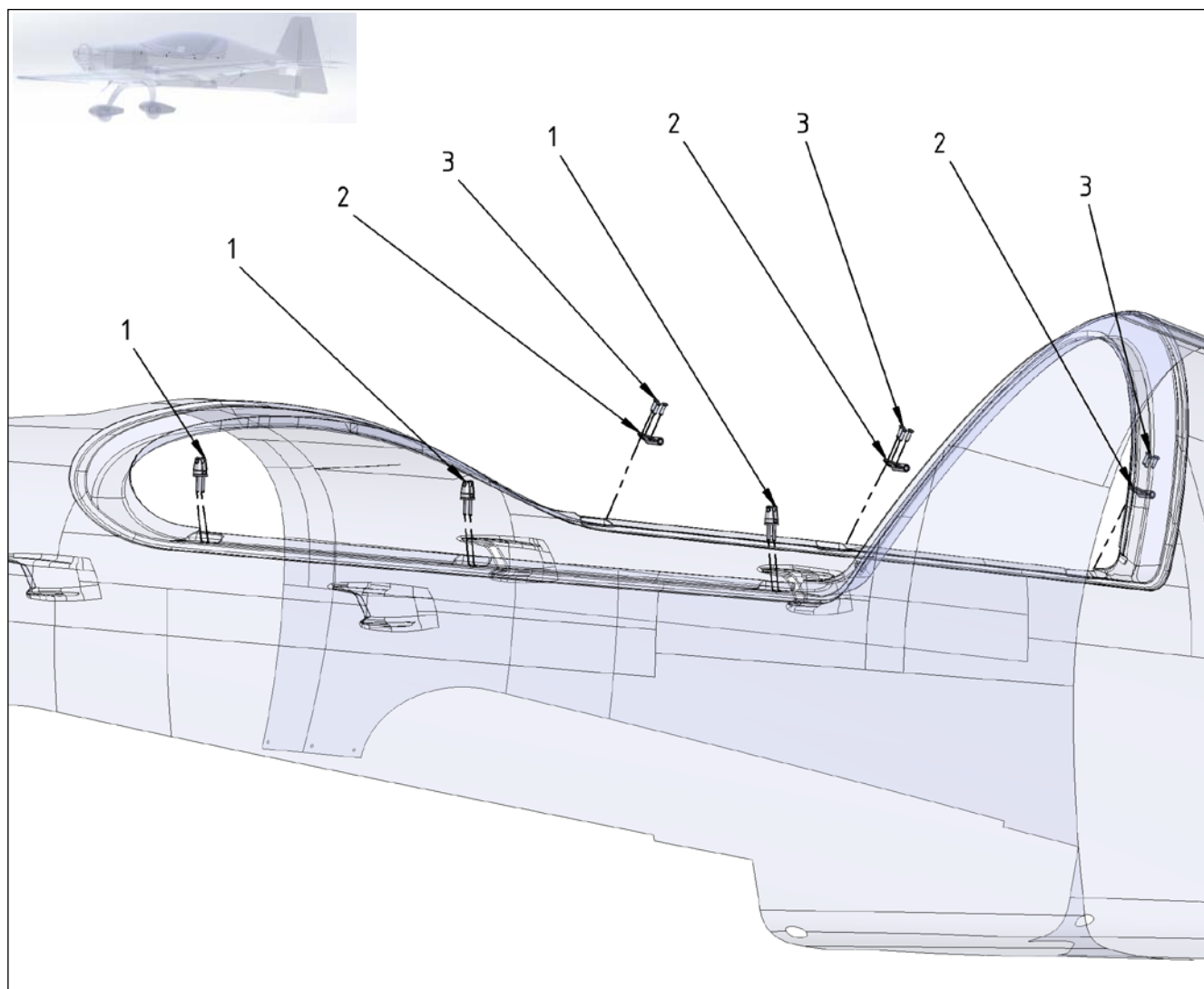
Figure 53-4 Canopy Attachment
