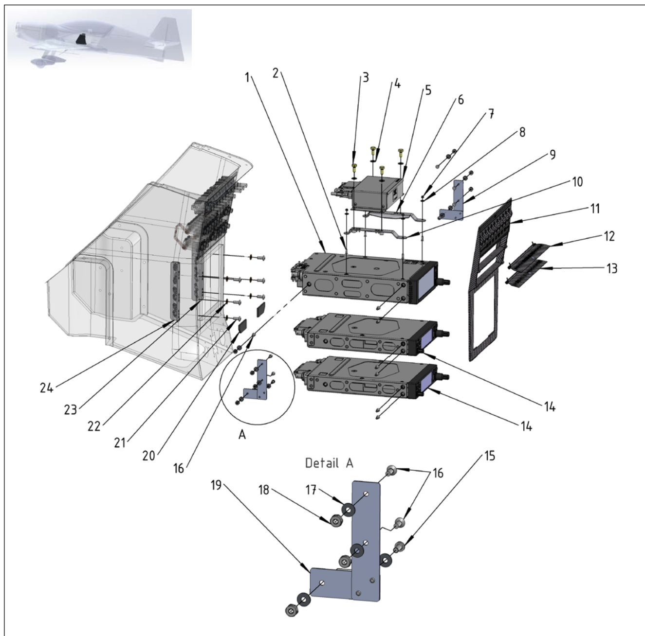
Figure 31-8 Center Console Options – GNX 375 + 2x GTR 205A + GAD 29 (≥089)
