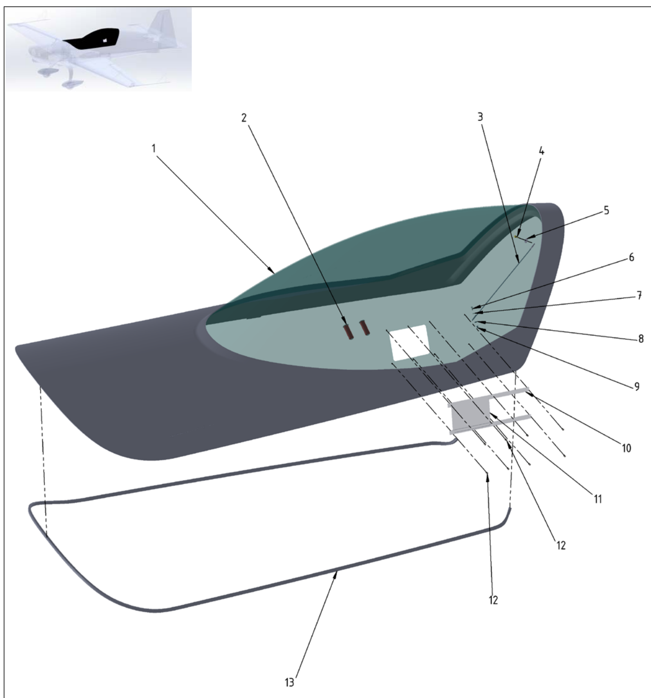
Figure 53-3 Single Seat Canopy
