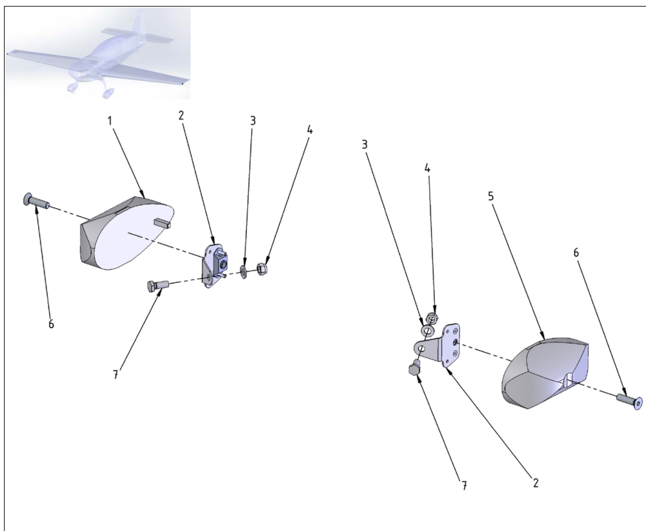
Figure 33-1 Exterior – Navigation/Strobe Light
