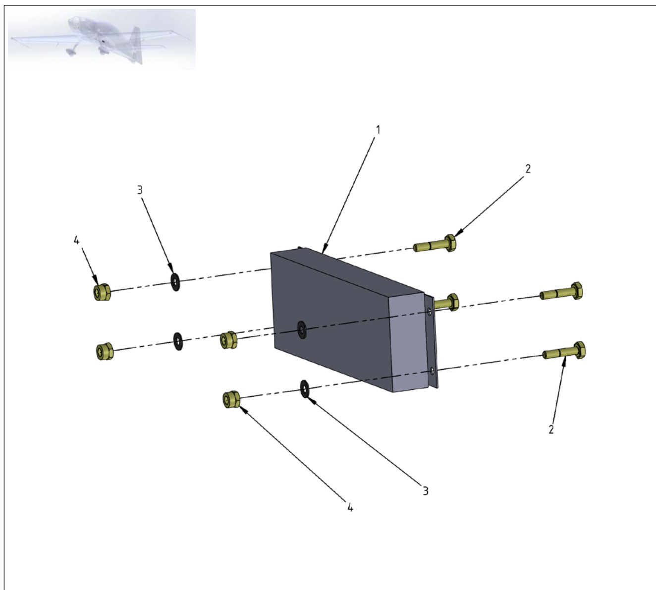
Figure 24-2 Integrated Battery Back-up System
