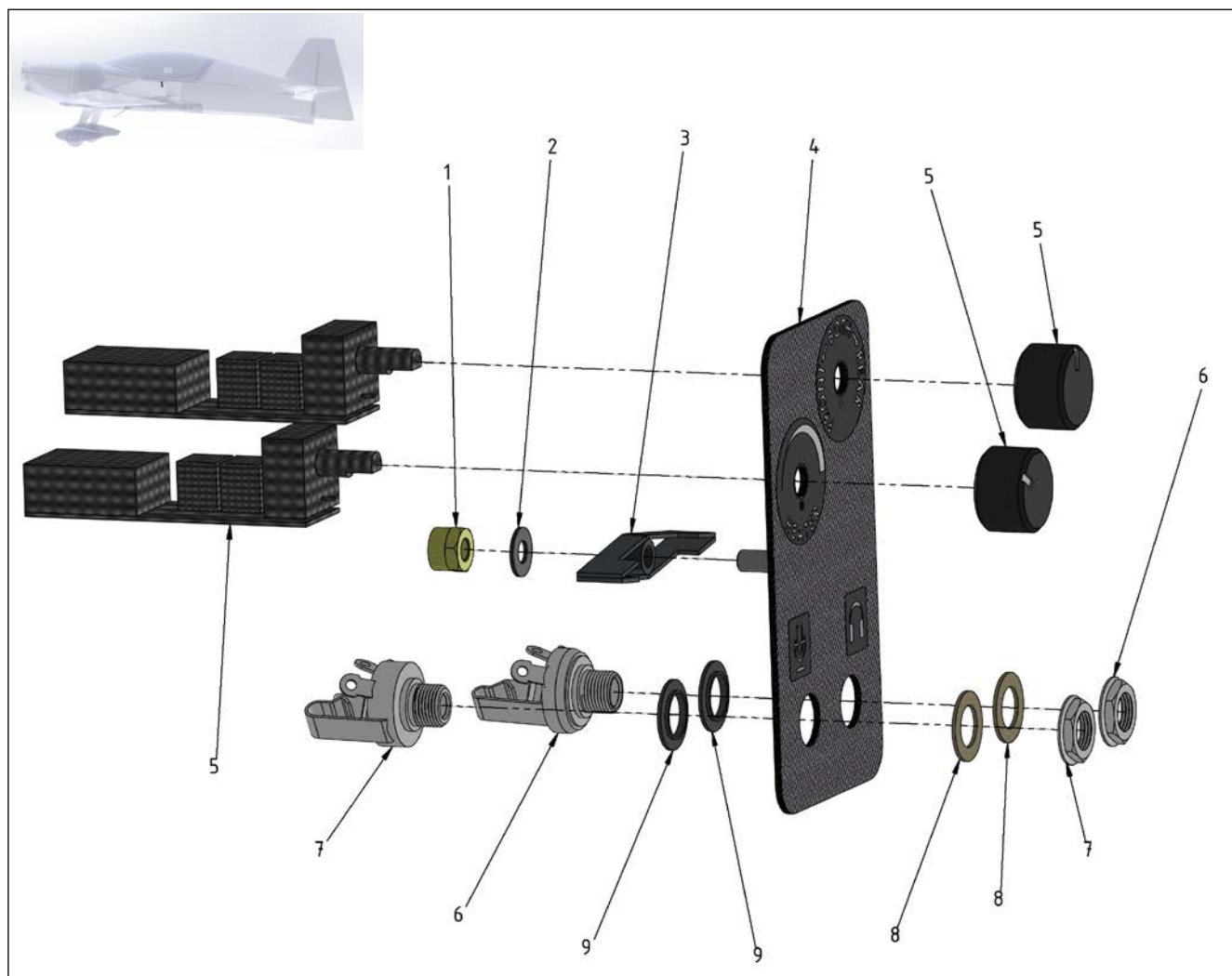
Figure 25-7 Control Panel (Pilot) – Cabin Heating System
