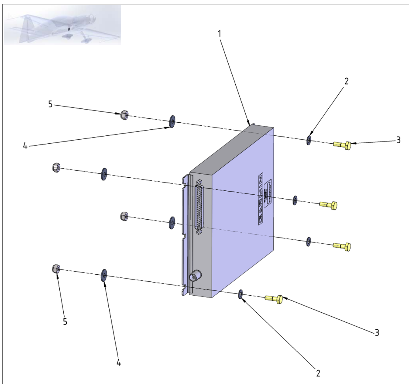
Figure 23-4 GTR 20 VHF DUAL COM
