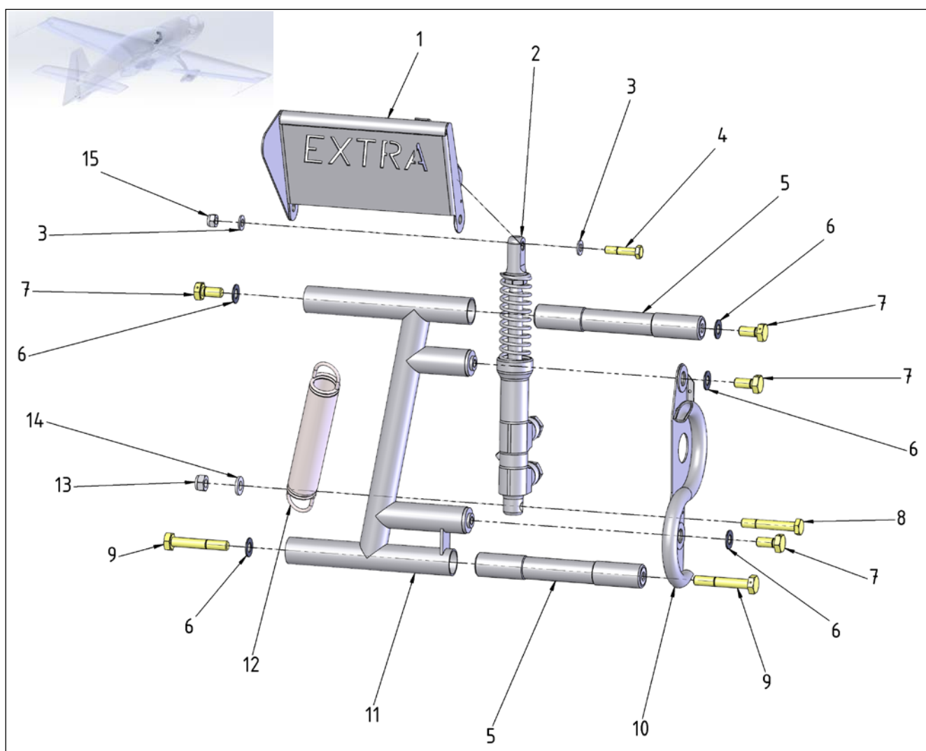
Figure 27-24 Front Pedal LH - Pedal
