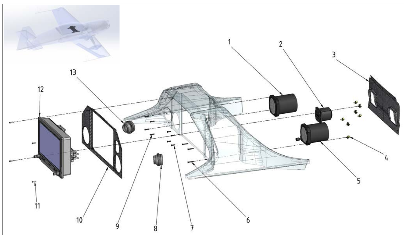
Figure 31-3 Instrument and Control Panels – Rear Instrument Panel
