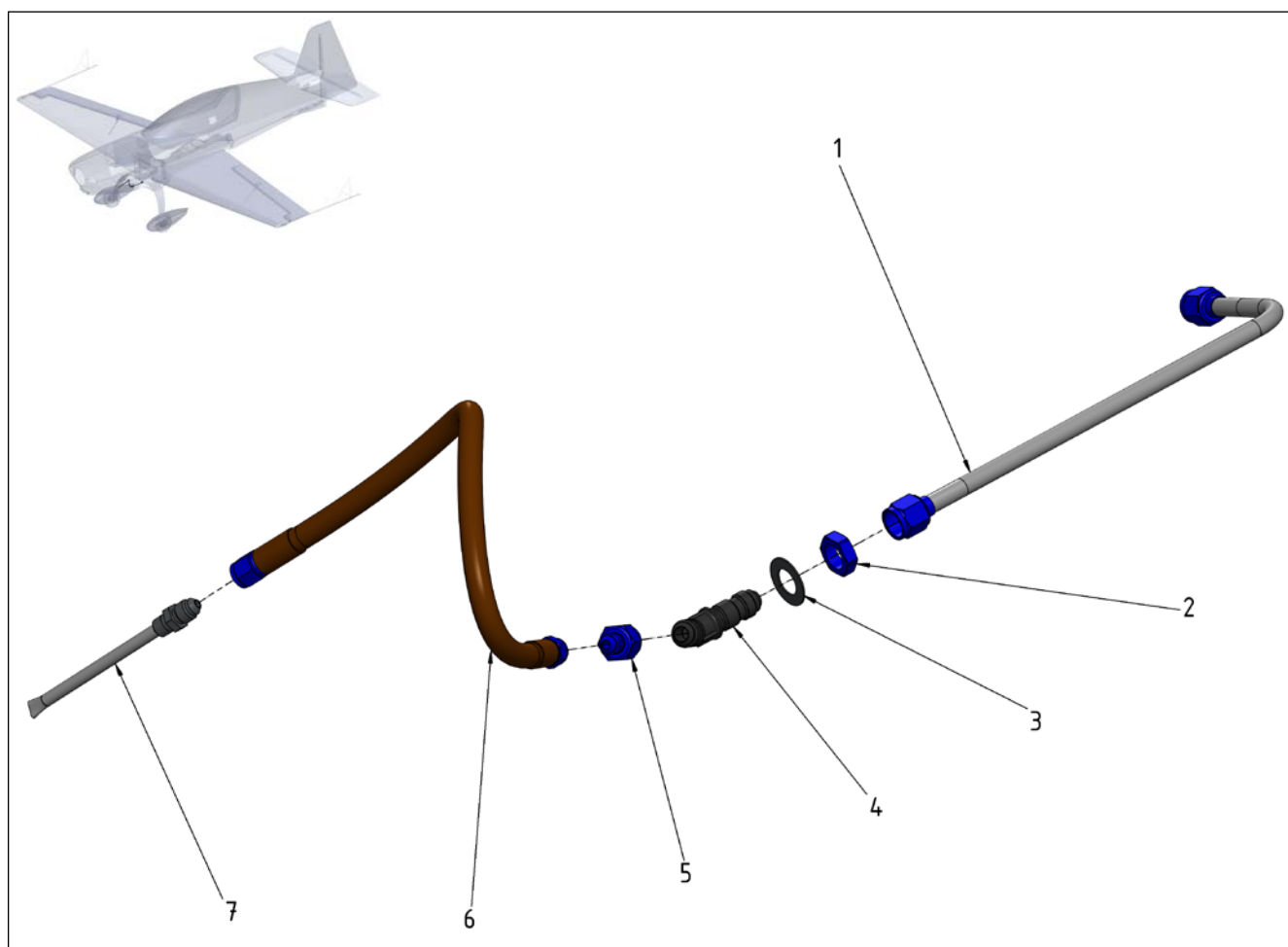
Figure 87-3 Smoke - Injection Gomolzig
