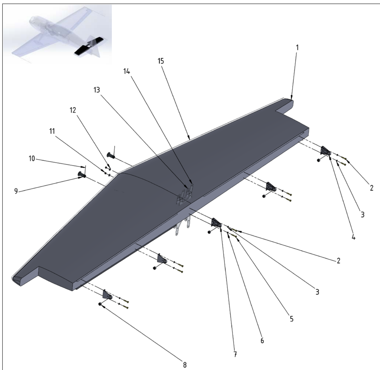
Figure 55-1 Horizontal Stabilizer
