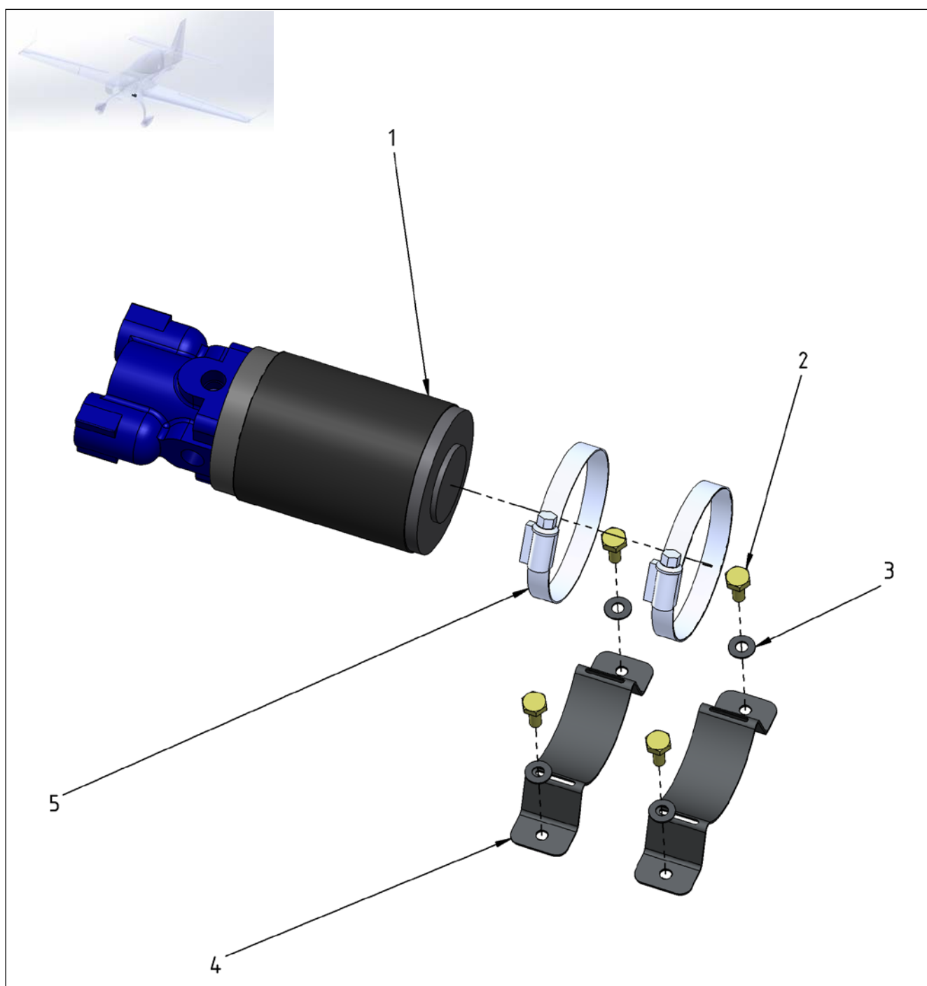
Figure 28-13 Distribution – Boost Pump
