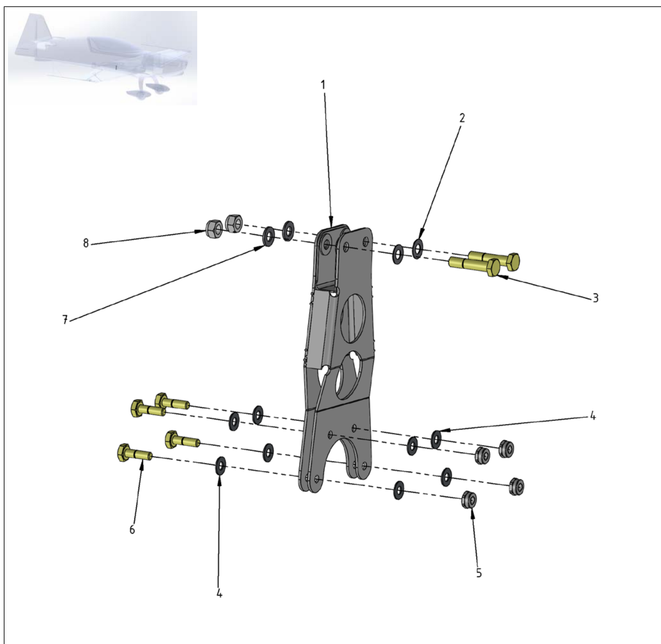
Figure 27-13 Aileron Drive Lever
