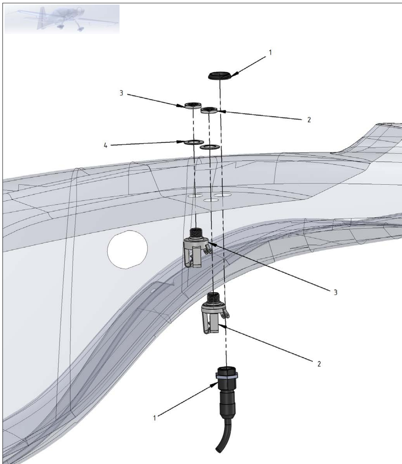
Figure 25-9 Headset Jacks (Copilot)
