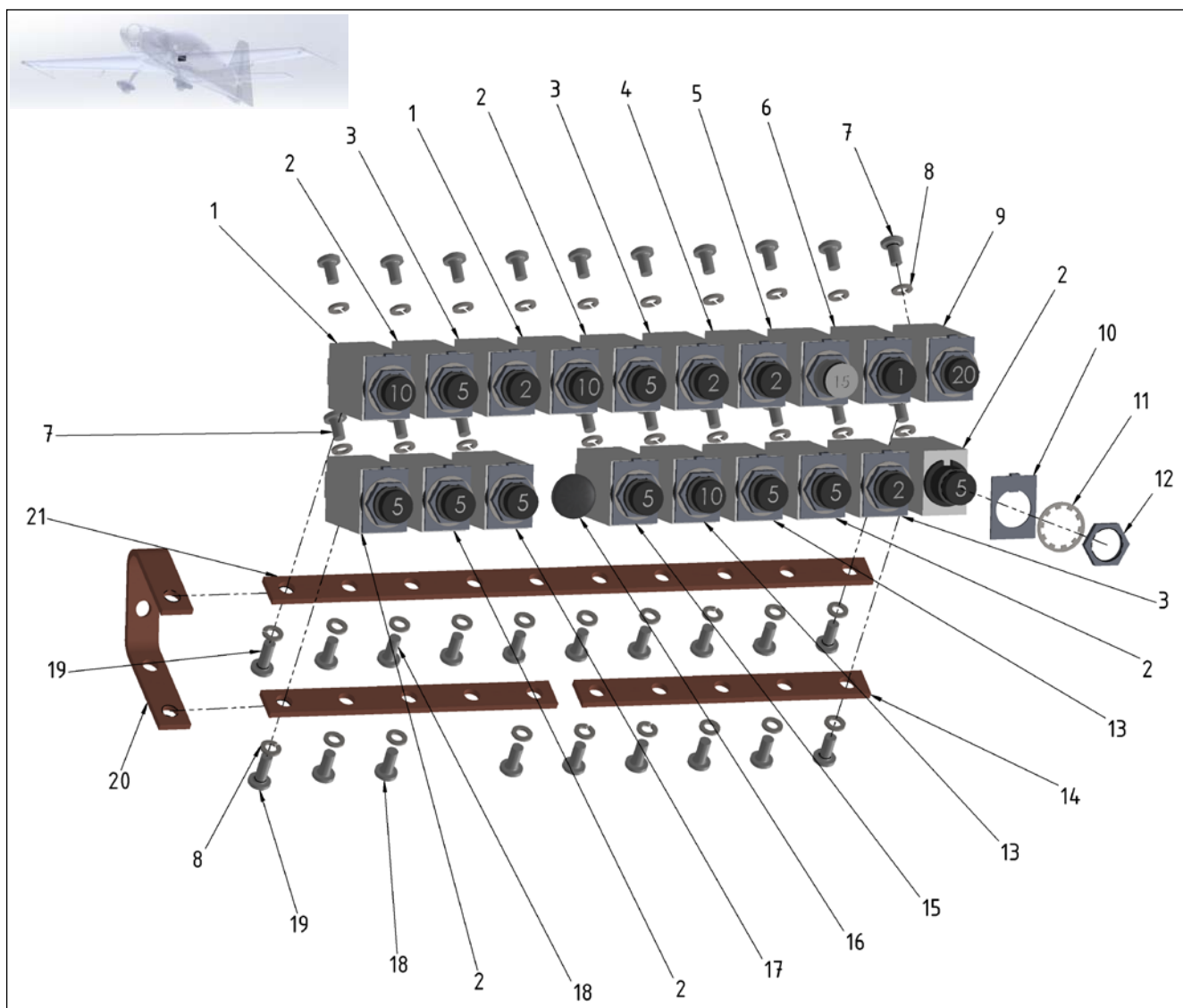
Figure 24-5 Circuit Breaker
