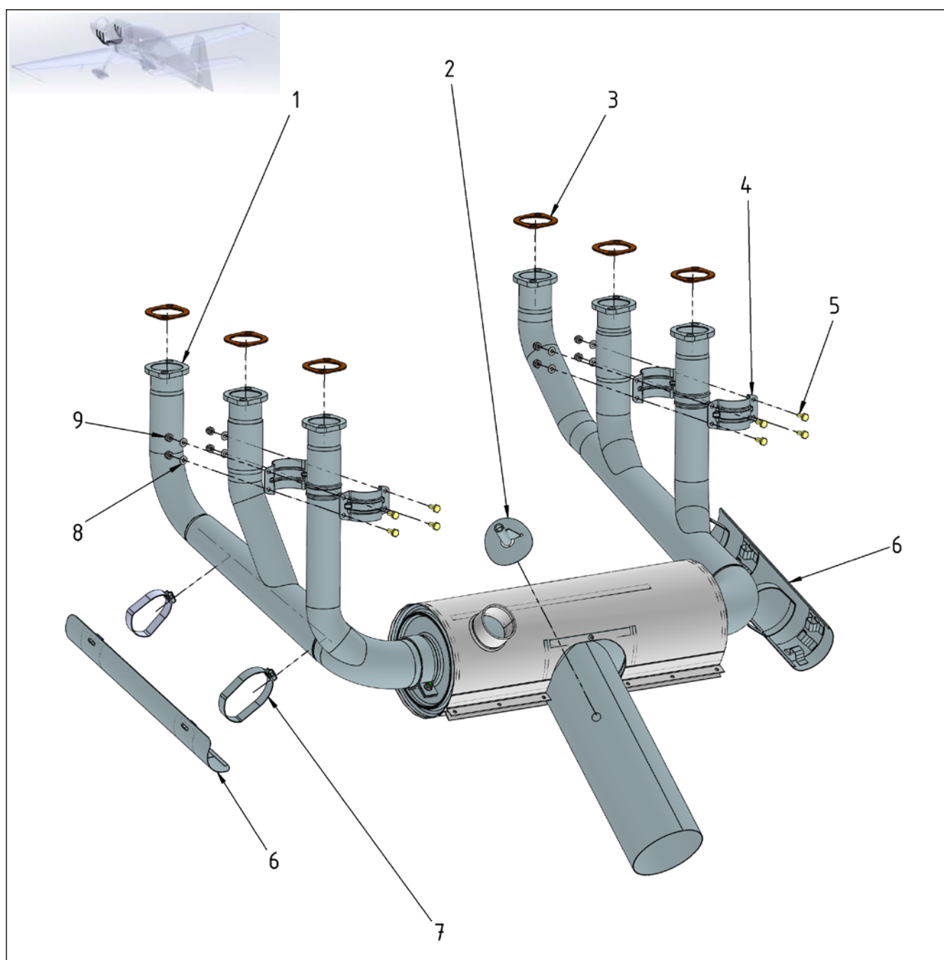
Figure 78-1 GOMOLZIG 6 in 1
