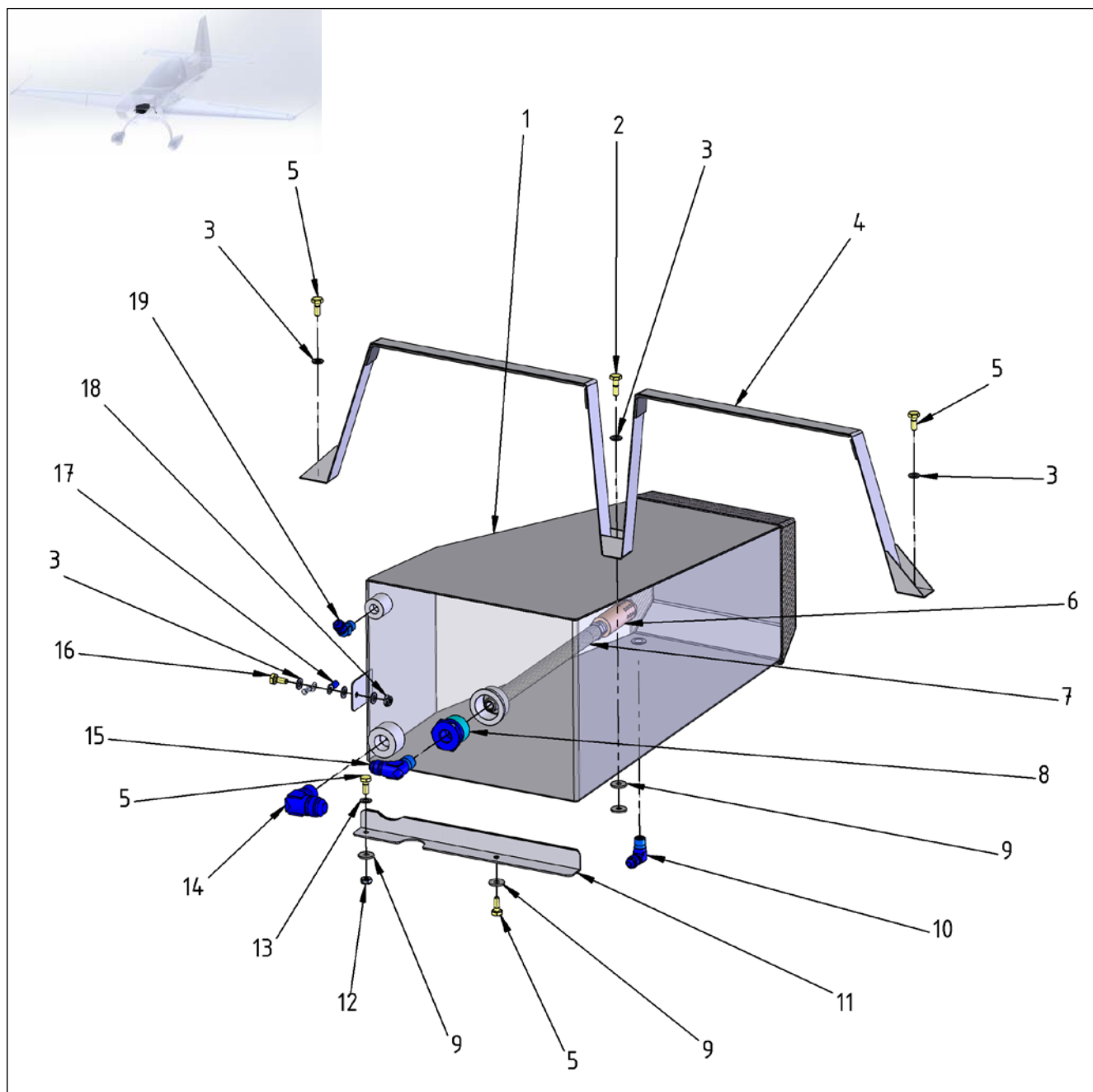
Figure 28-2 Storage – Acro Tank
