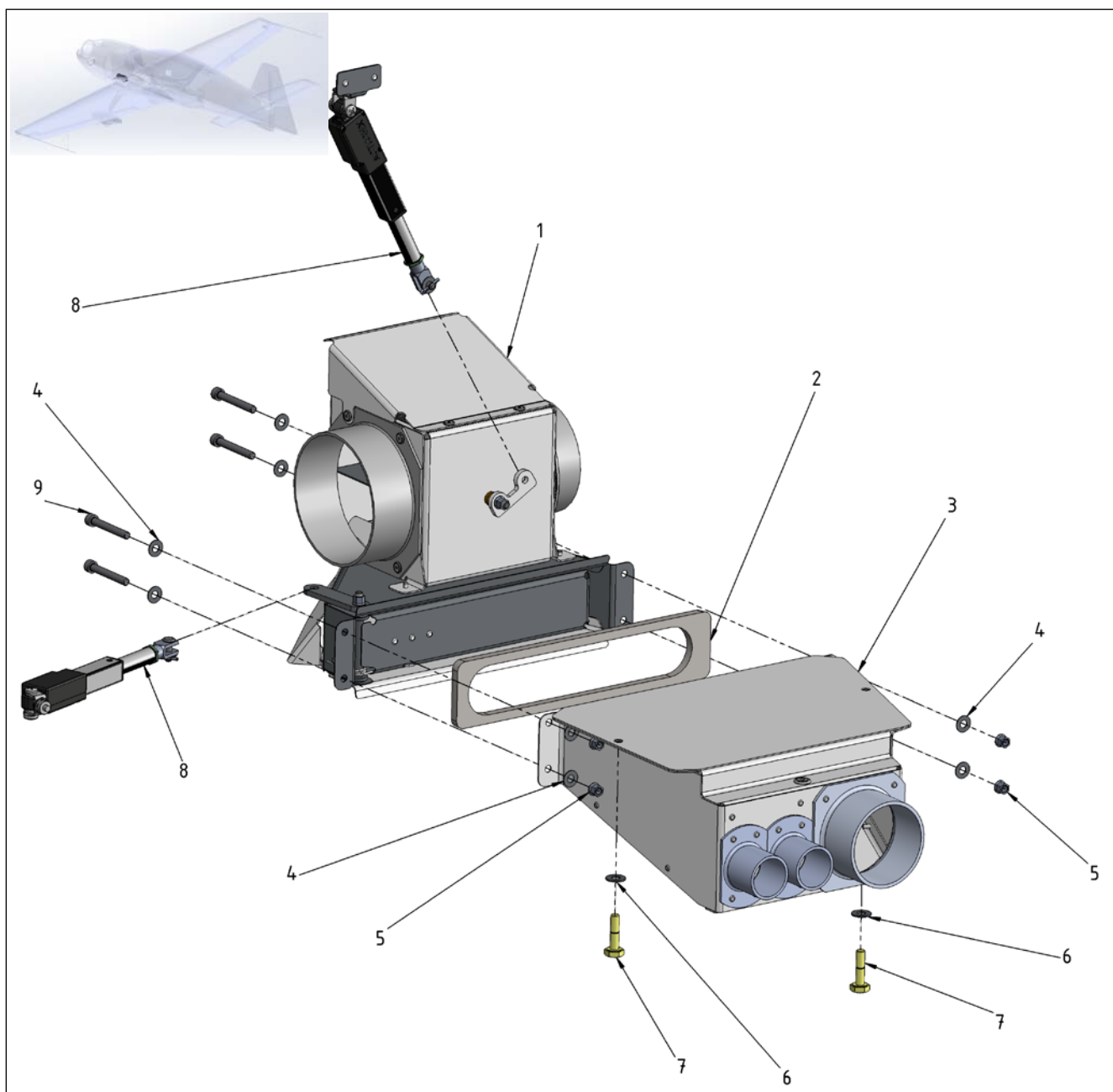
Figure 21 -4 Cabin Ventilation System - Boxes
