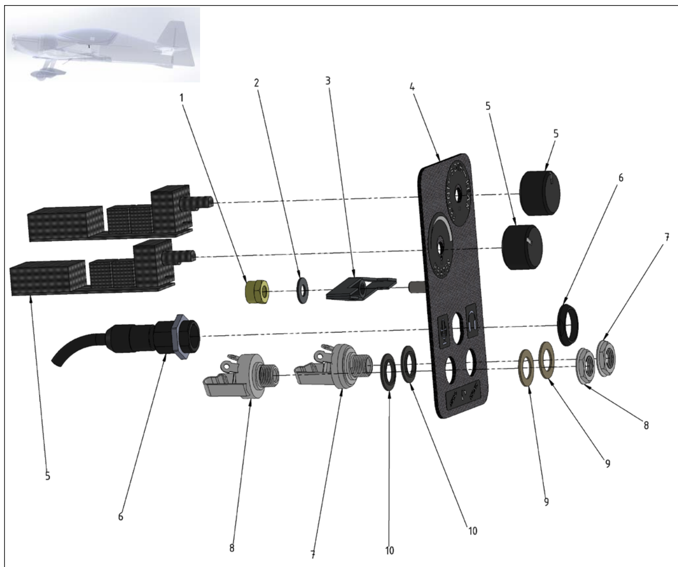
Figure 25-8 Control Panel (Pilot) – Complete
