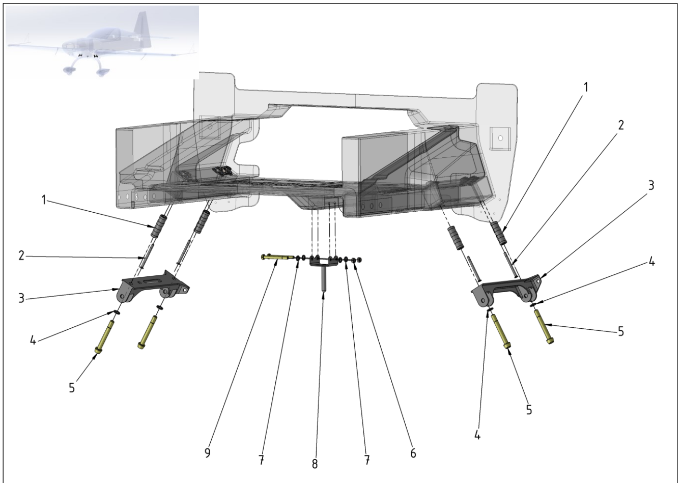
Figure 32-2 Main Gear - Landing Gear Brackets
