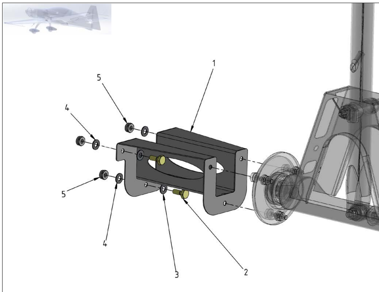
Figure 27-12 Torque Tube Bracing
