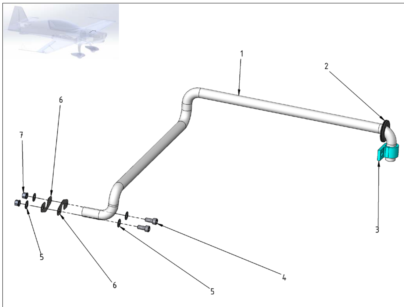
Figure 28-9 Ventilation Line – Tank Compartment Vent
