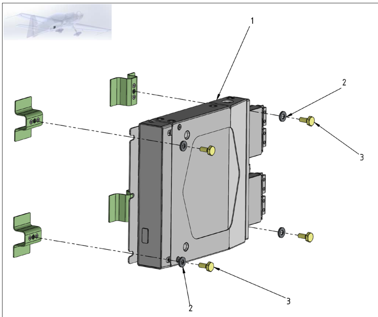
Figure 23-2 GMA 245R Audio Panel
