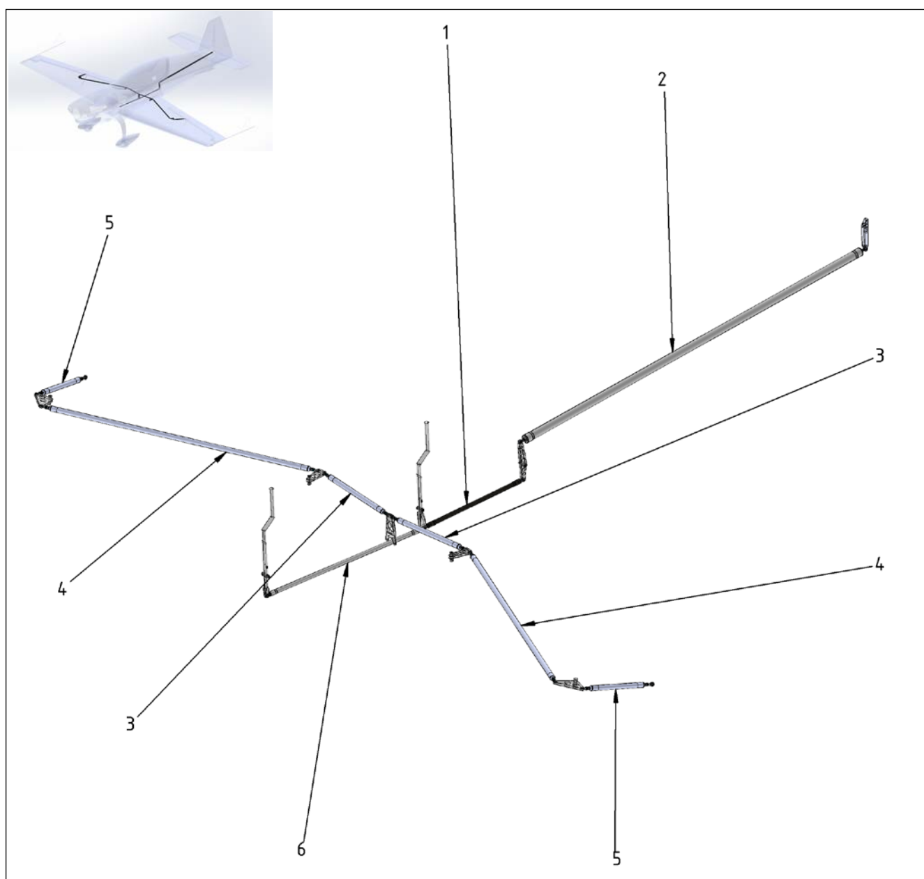
Figure 27-1 Control Rods
