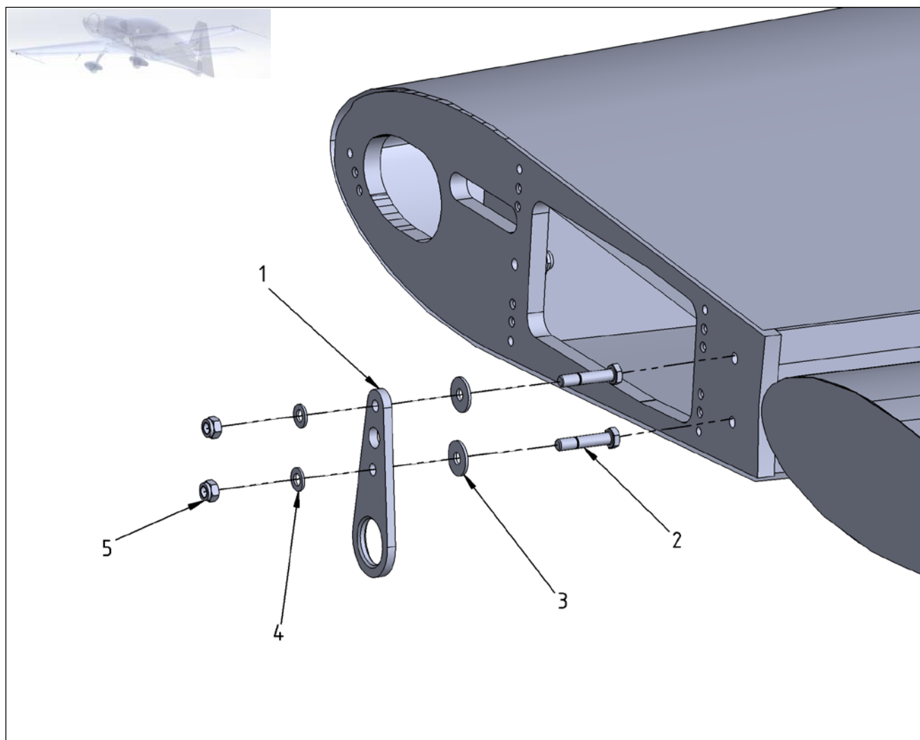
Figure 57-3 Wing Tie Down Ring
