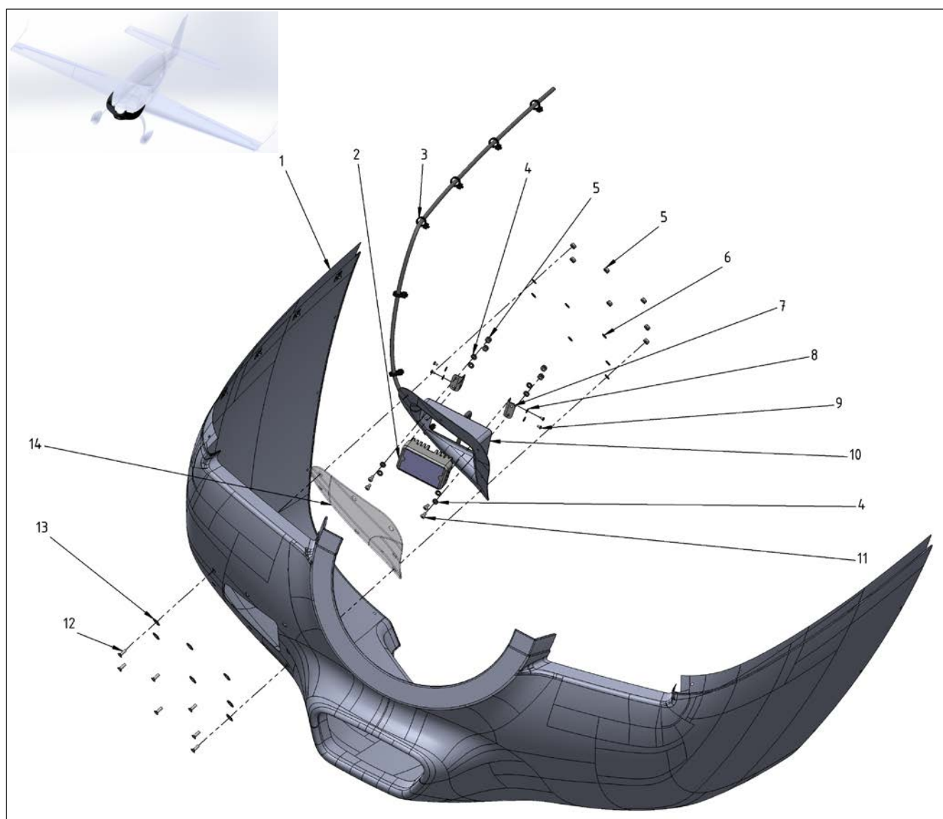
Figure 33-2 Exterior – Landing Light System
