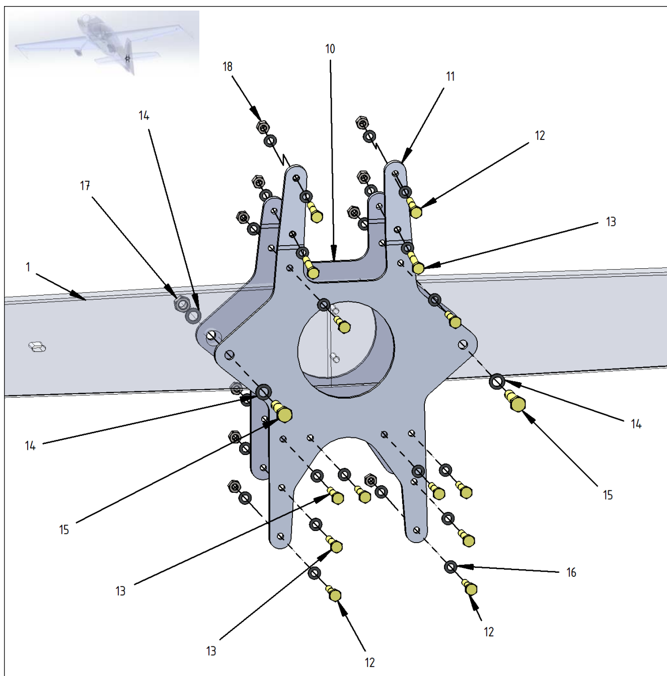
Figure 55-2 Connection Plates
