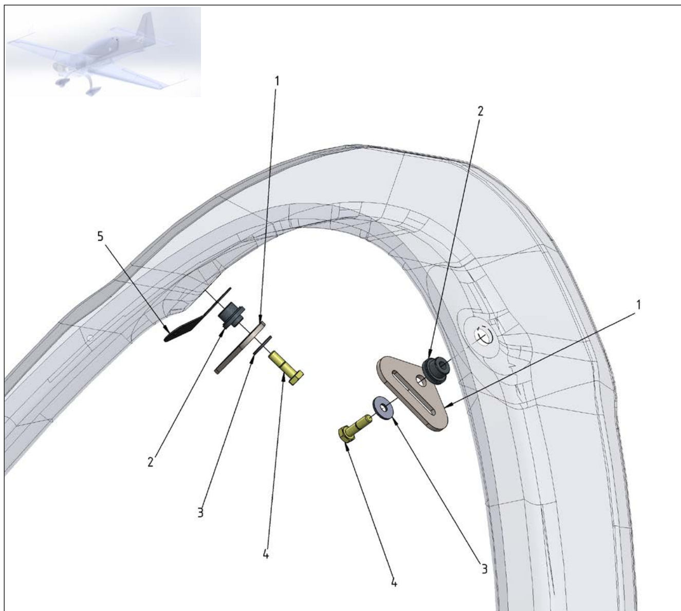
Figure 25-15 Pilot Shoulder Harness
