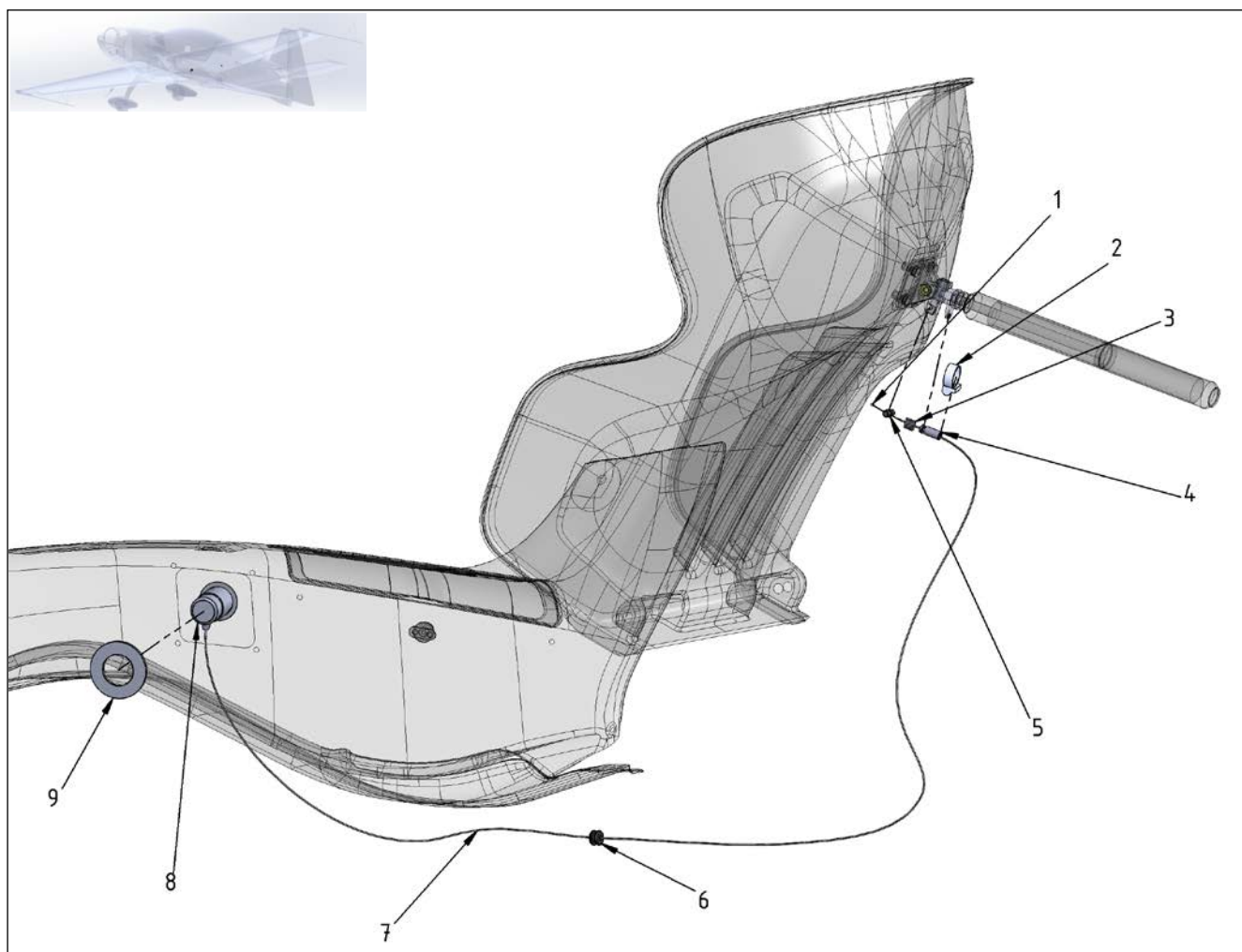
Figure 25-2 Bowden Cable Backrest
