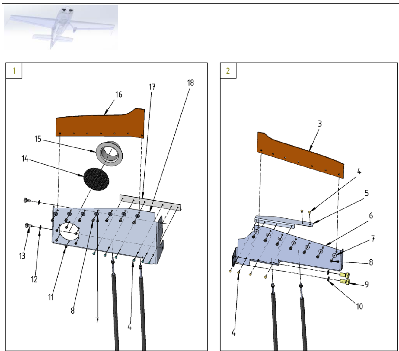
Figure 71-4 Air Baffles – Air Baffles FWD
