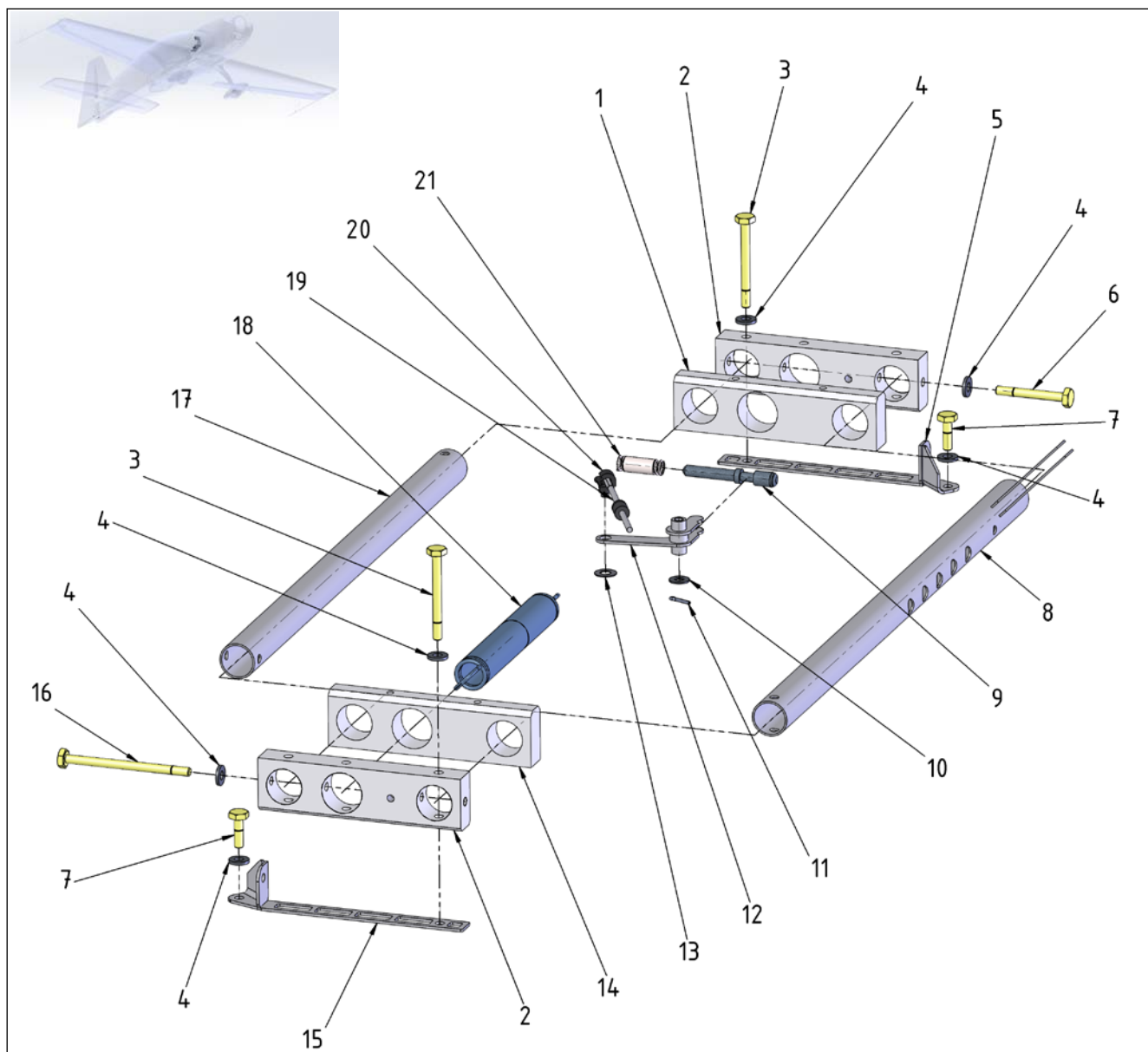
Figure 27-26 Front Pedal LH - Base
