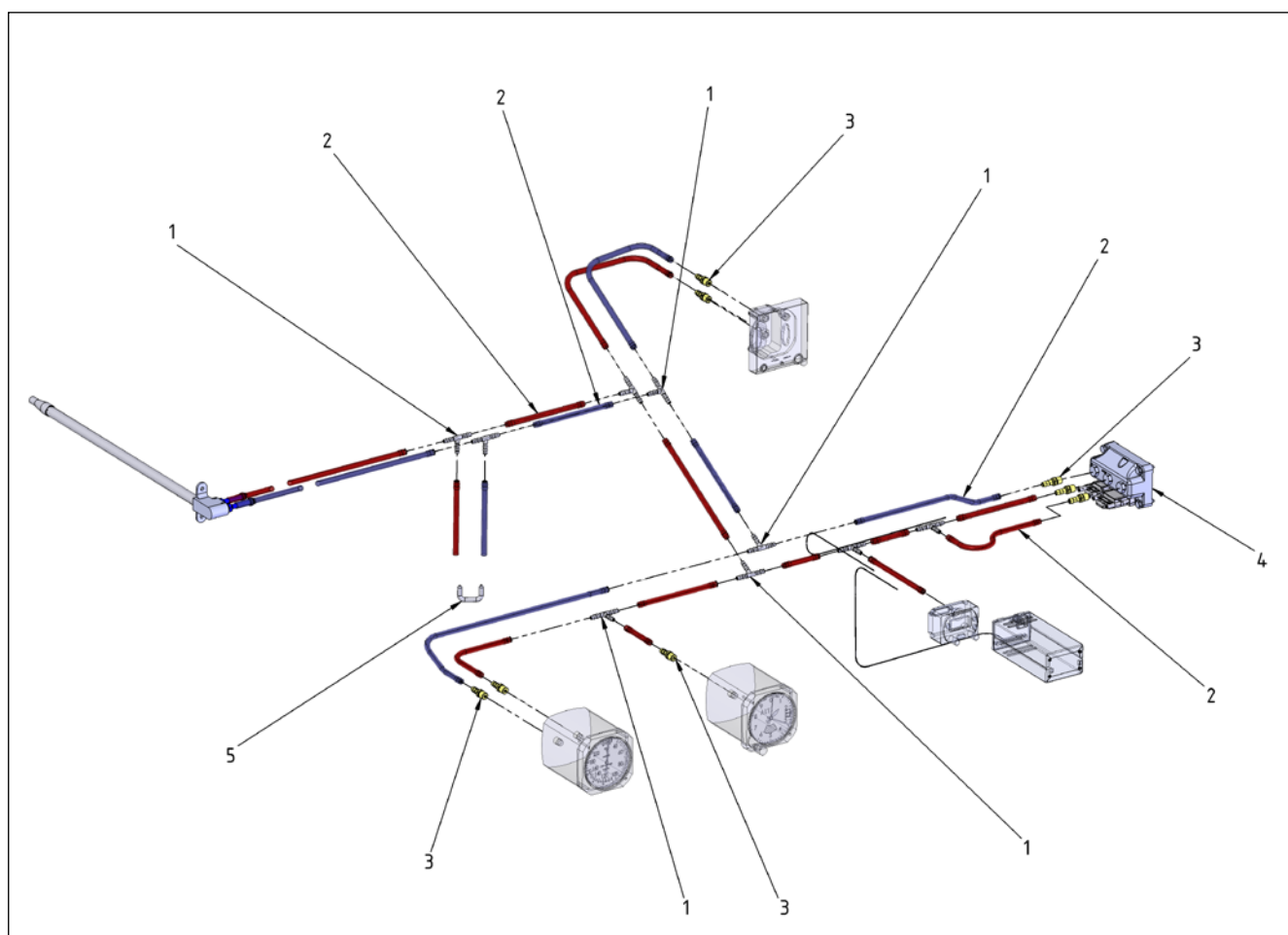
Figure 34-2 Environment Data – Static System
