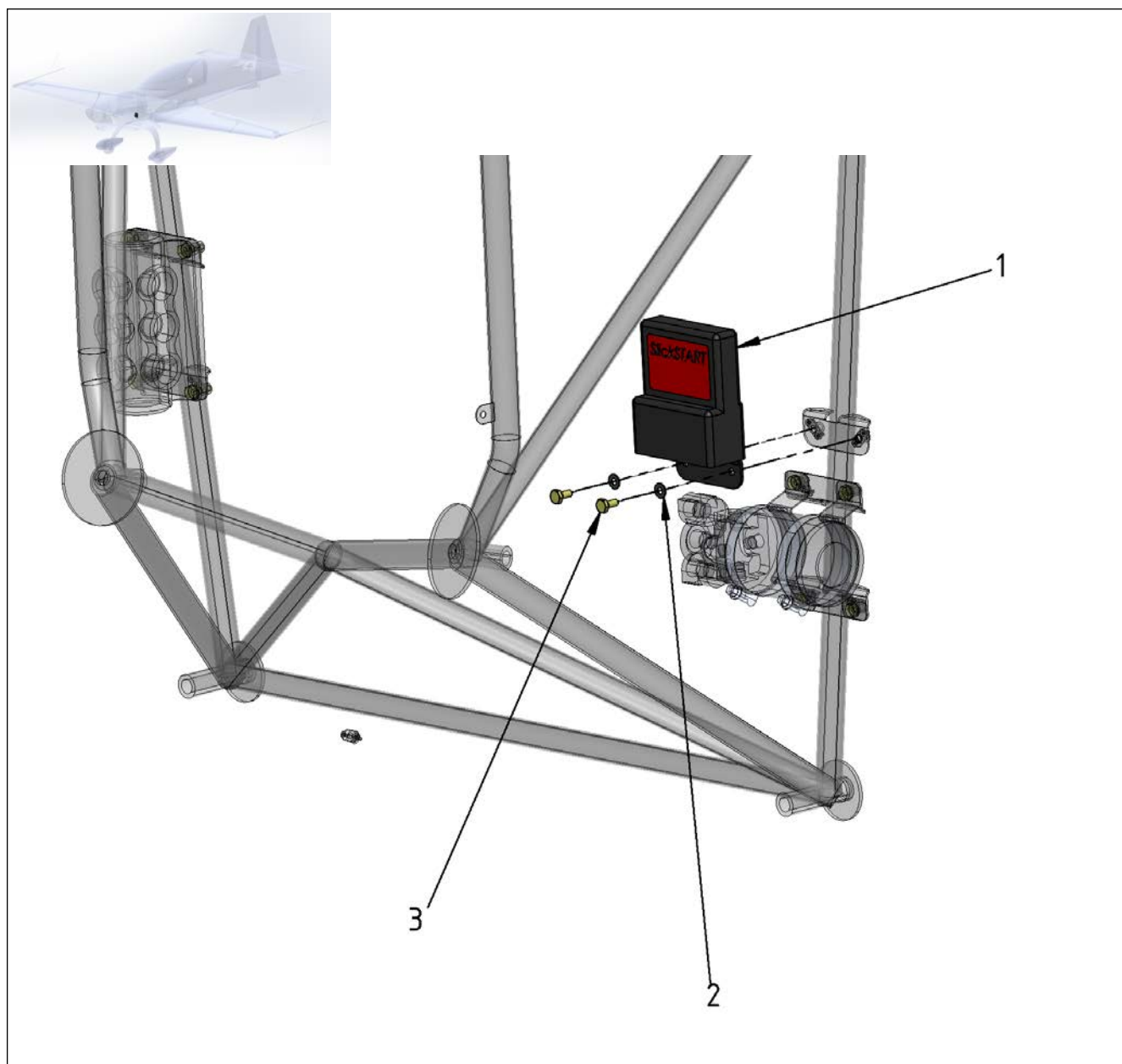
Figure 72-2 Slick Start
