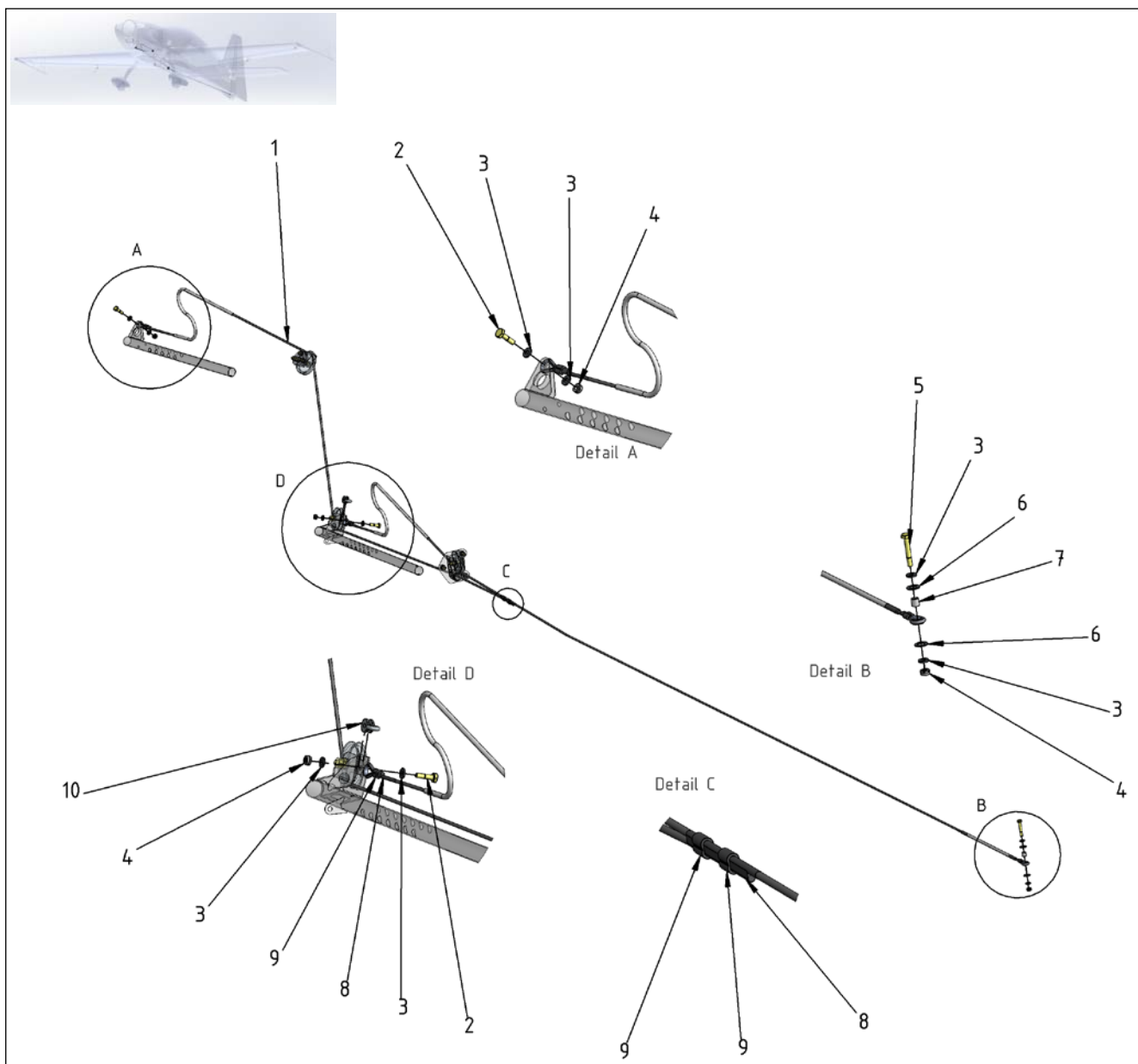
Figure 27-22 Rudder Control – Control Cable
