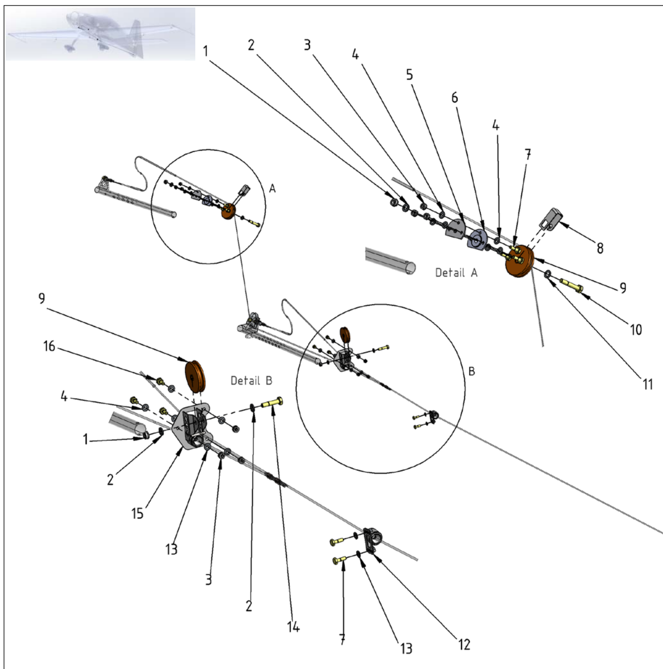
Figure 27-23 Rudder Control – Control Cable Guidance
