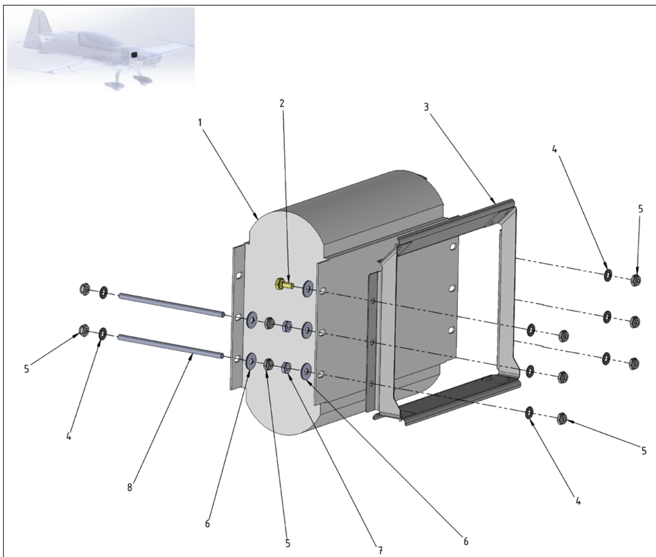
Figure 79-2 Distribution – Oil Cooler
