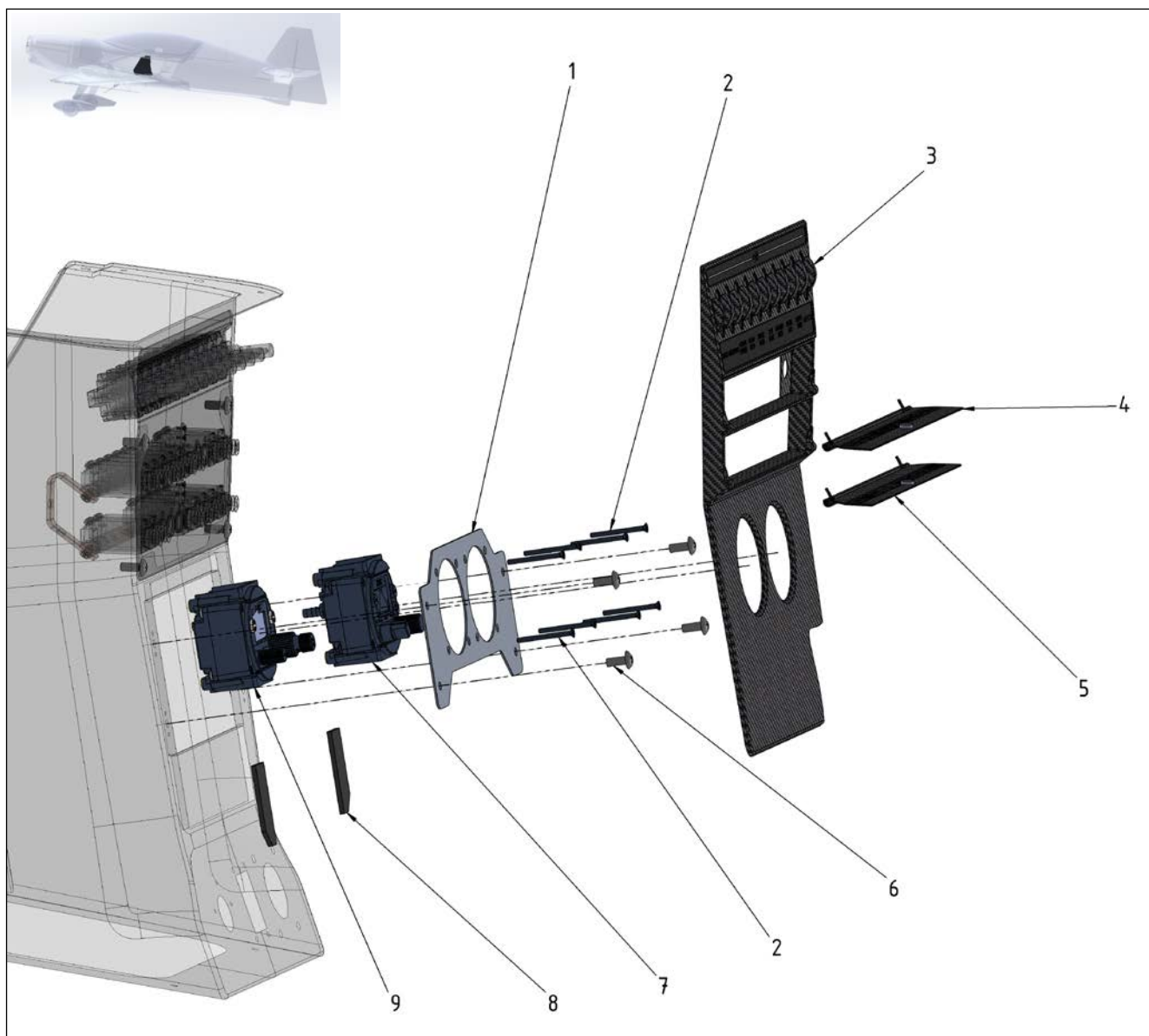
Figure 31-5 Instrument and Control Panels – Center Console Cover
