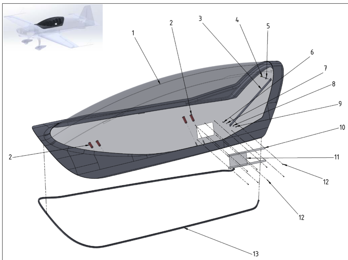
Figure 53-2 Canopy
