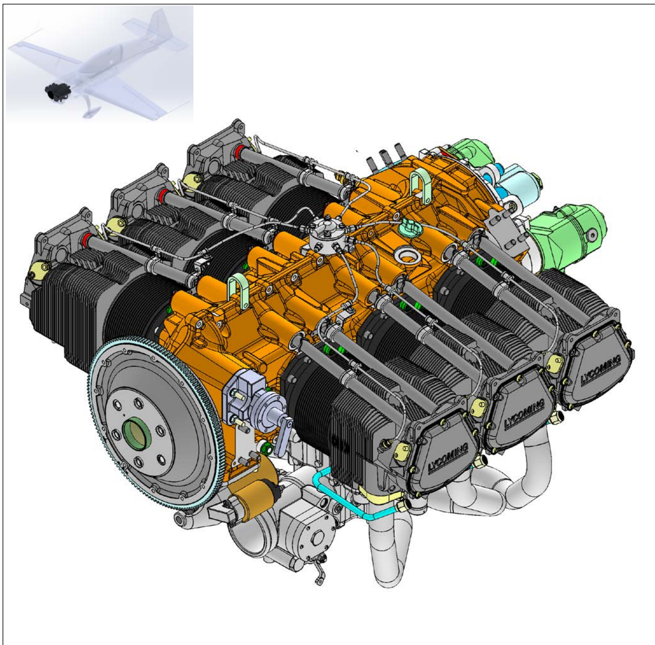
Figure 72-1 Engine
