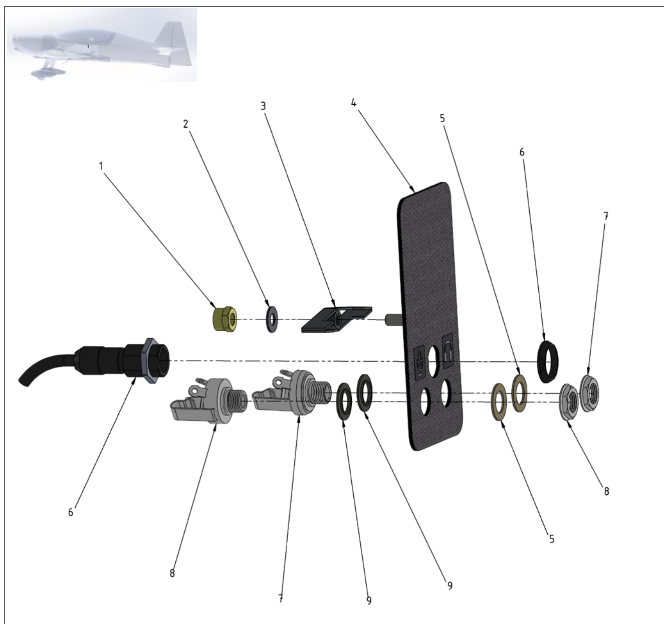
Figure 25-6 Control Panel (Pilot) – Bose LEMO
