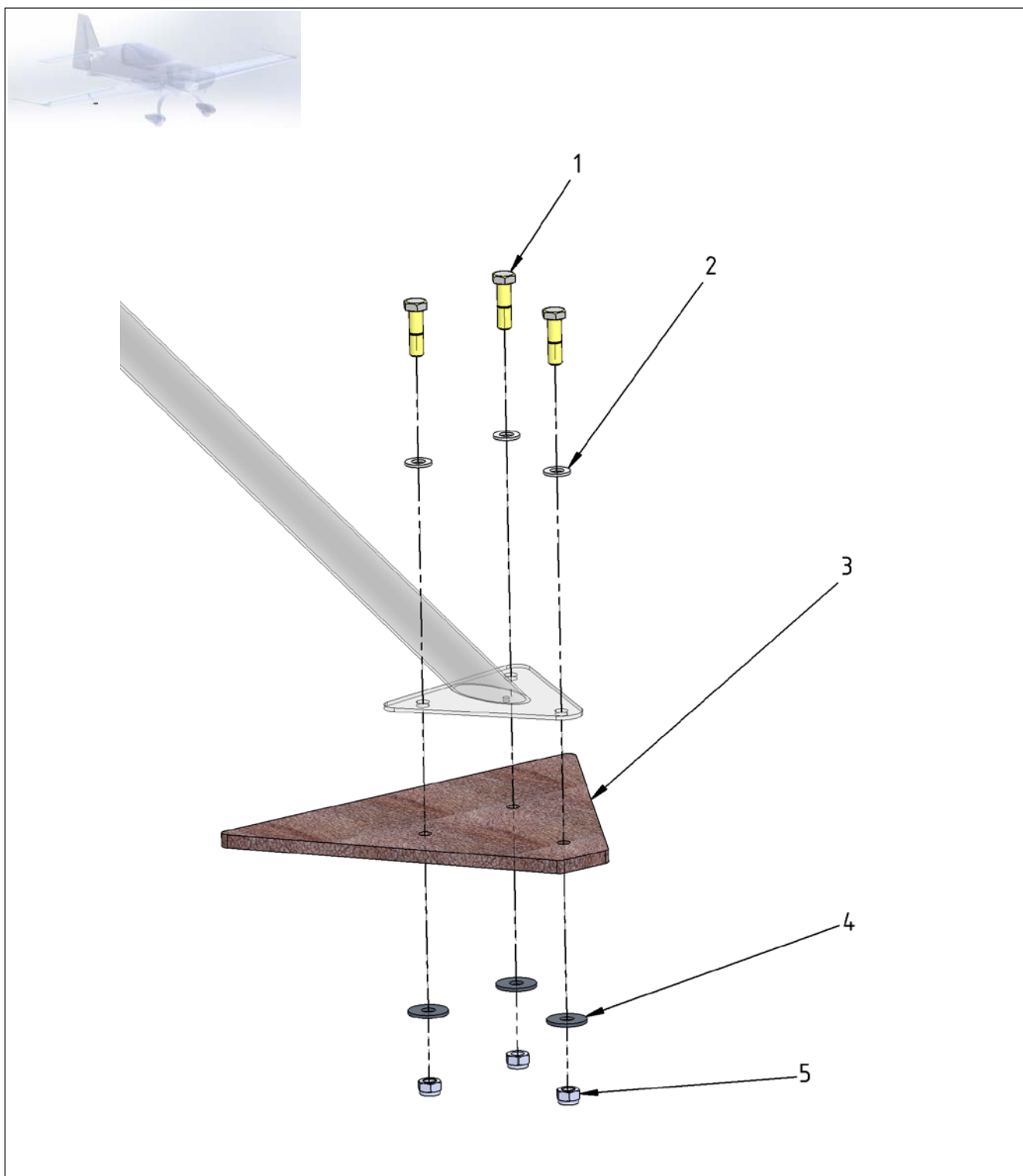
Figure 27-19 Spades – RH Spade
