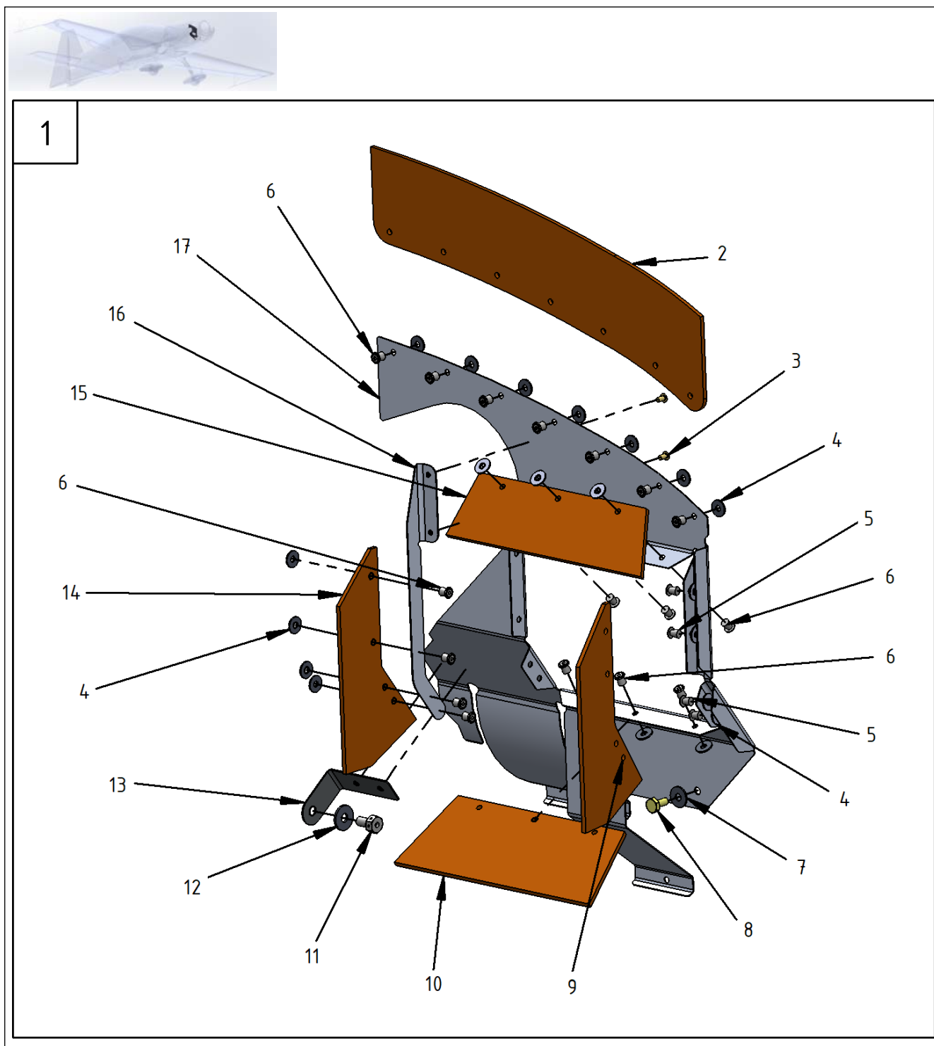
Figure 71-8 Air Baffles – Air Baffles AFT RH
