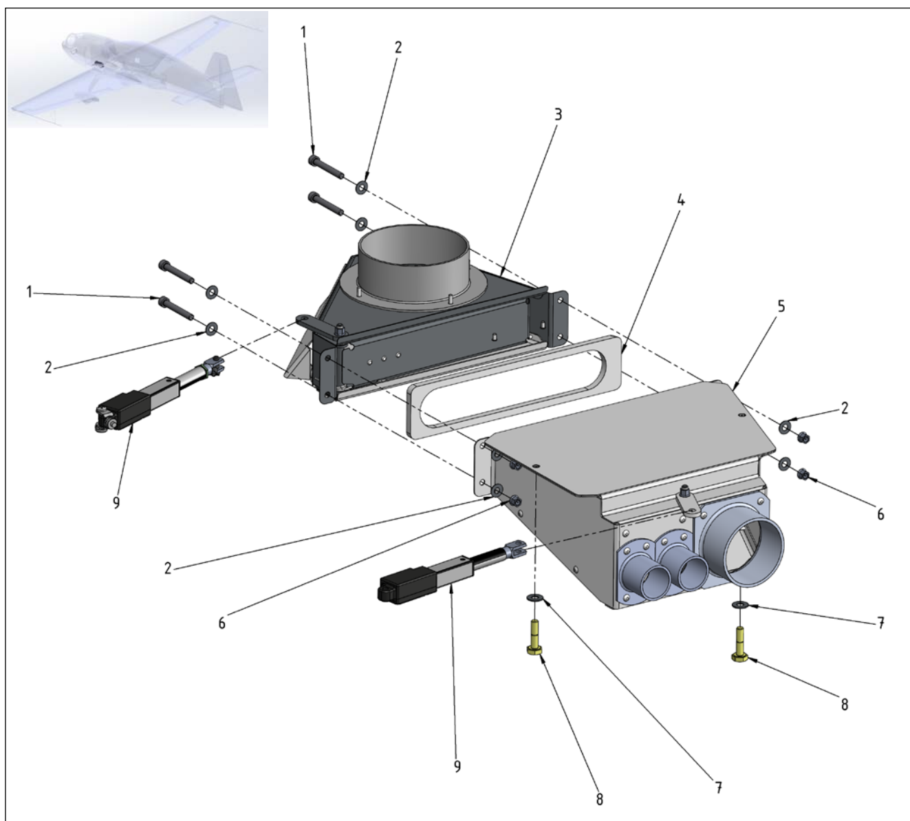
Figure 21-2 Boxes
