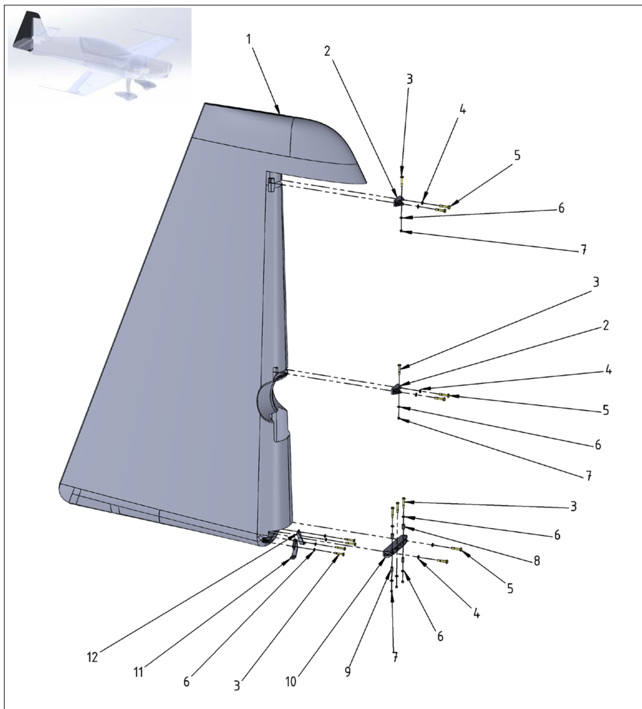
Figure 27-20 Rudder Control - Rudder
