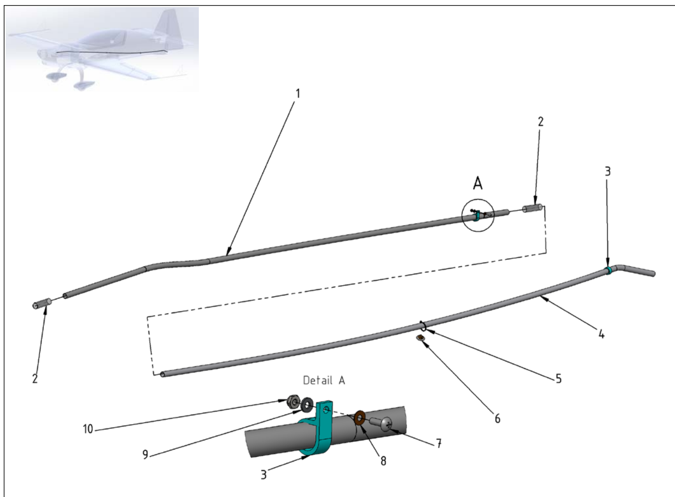
Figure 79-1 Breather Line
