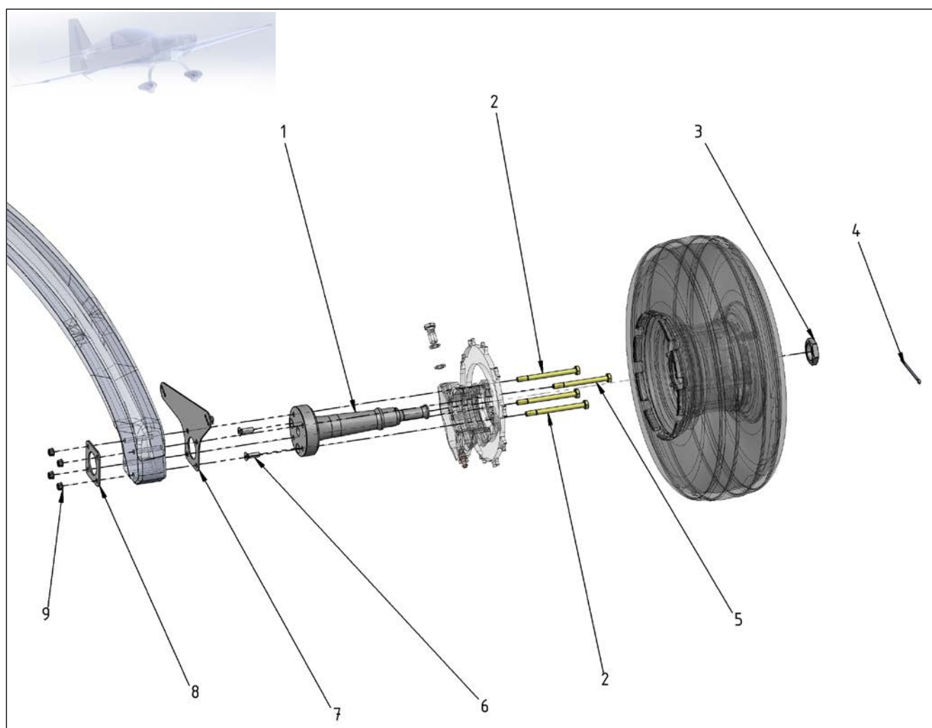
Figure 32-4 Main Gear – Wheel Axis
