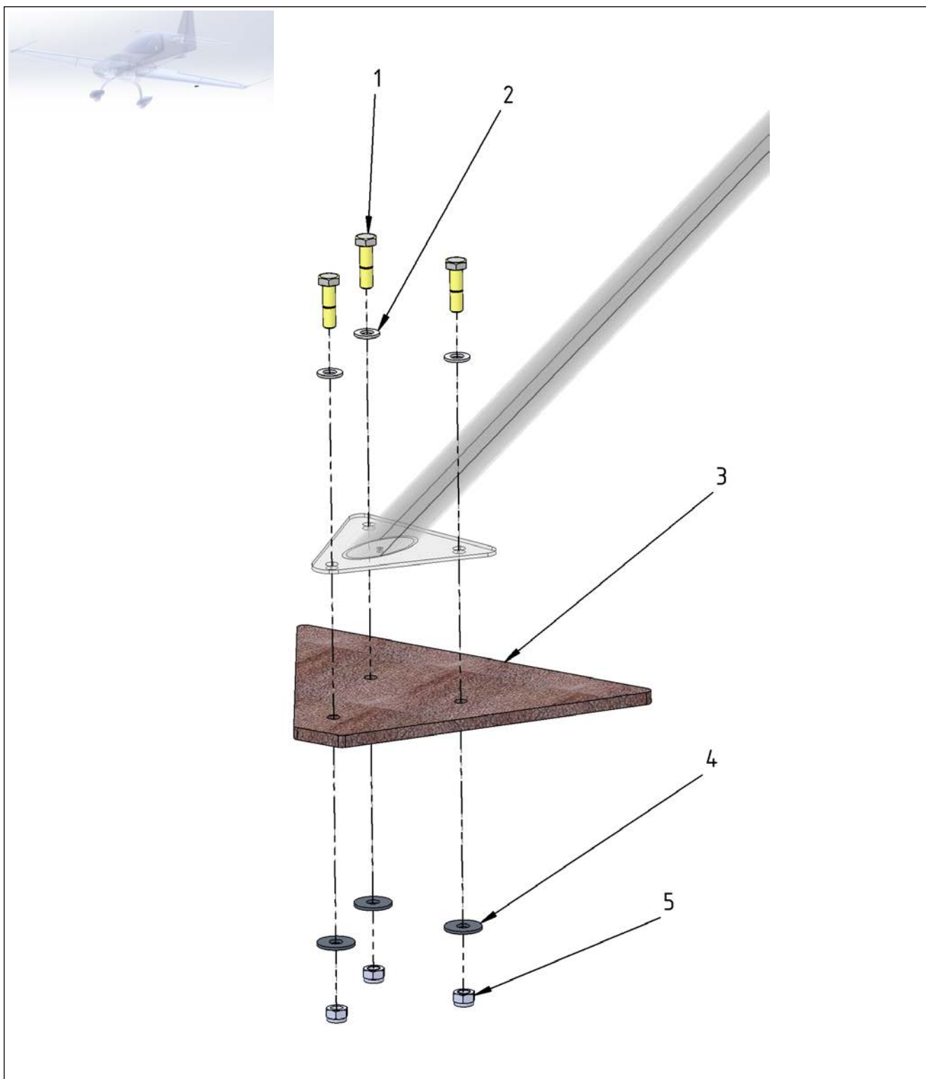
Figure 27-18 Spades – LH Spade
