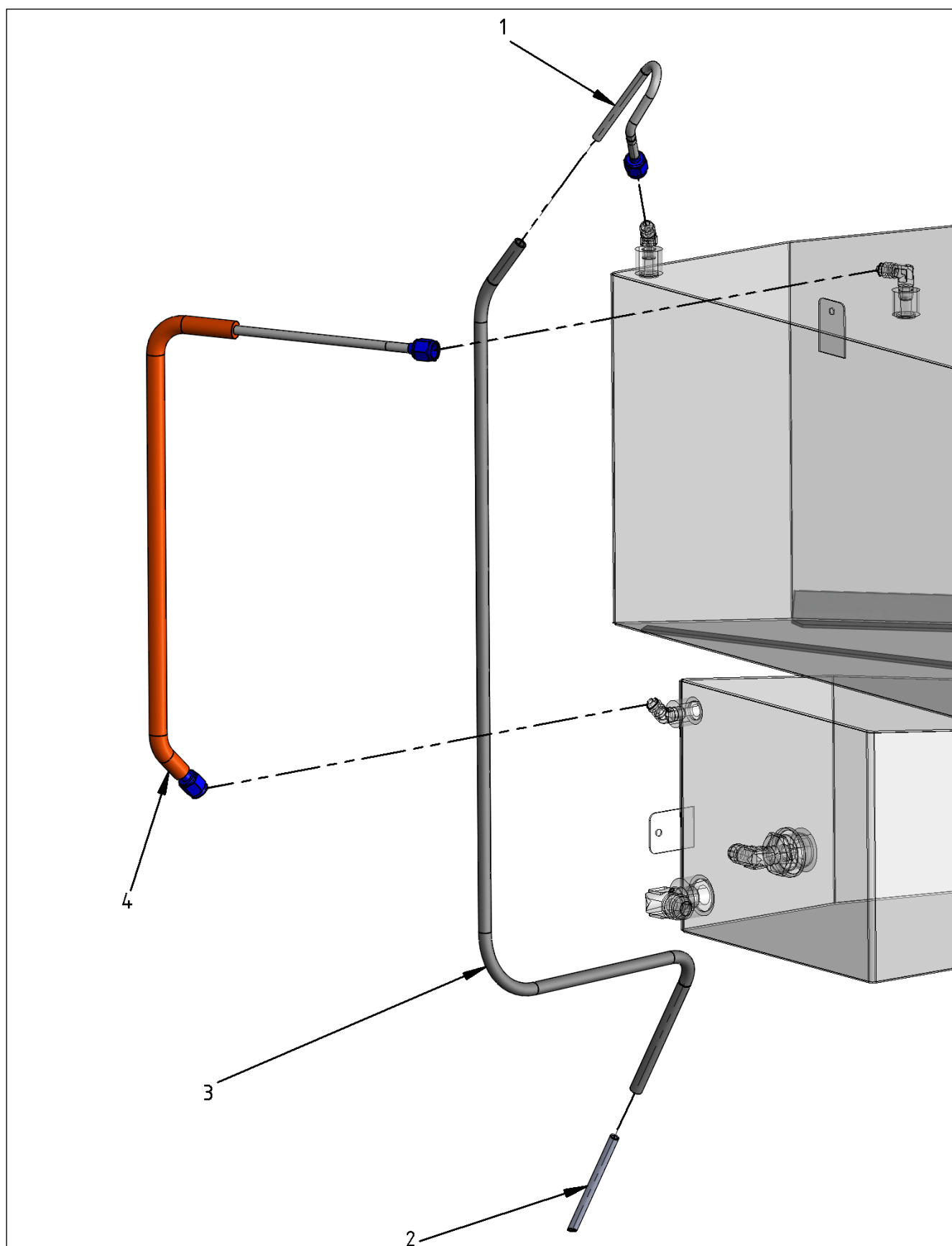
Figure 28-7 Ventilation Line – Center Tank
