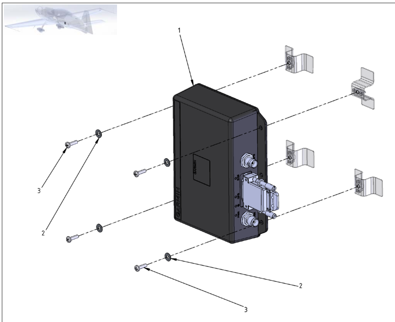
Figure 34-6 Dependent Position Determining – Garmin GDL 51R
