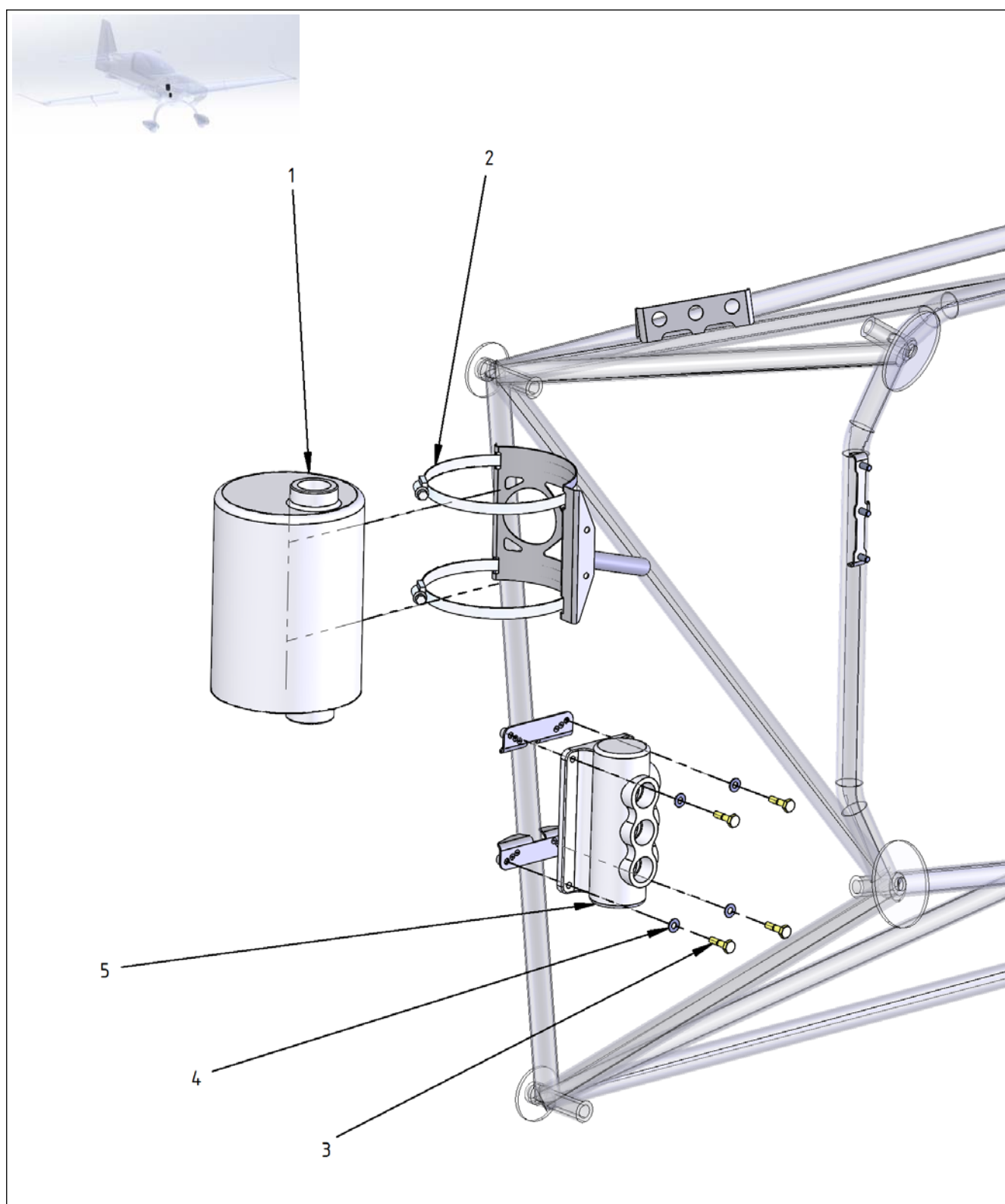
Figure 79-4 Oil Separator and Oil Valve
