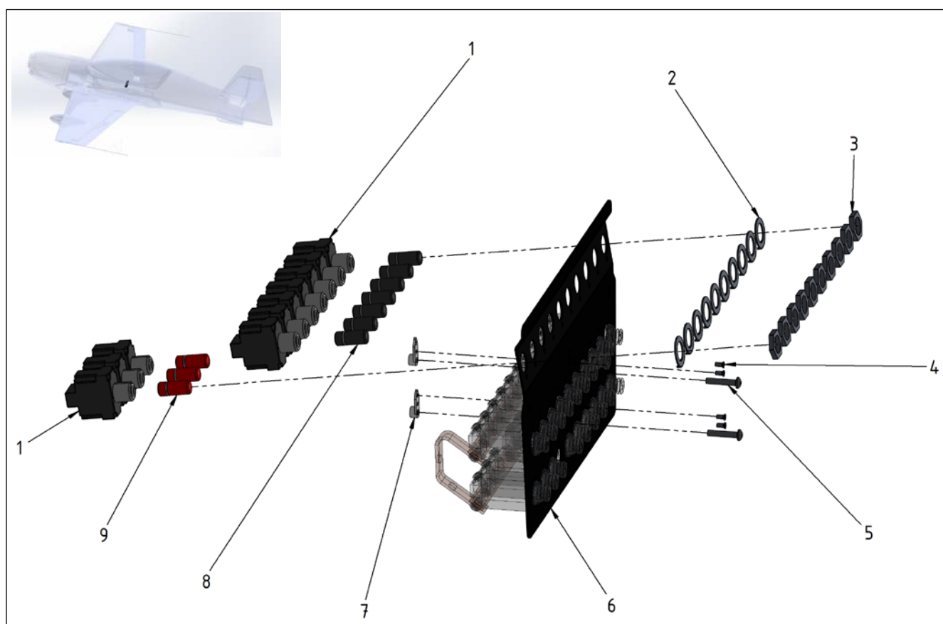
Figure 24-6 Toggle Switch
