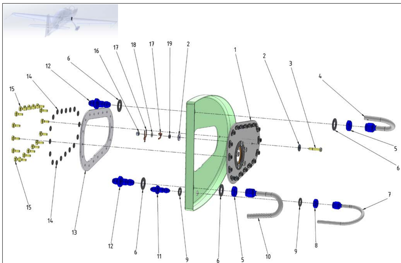
Figure 28-4 Storage - Wing Tank Inspection Door with Outlets - RH
